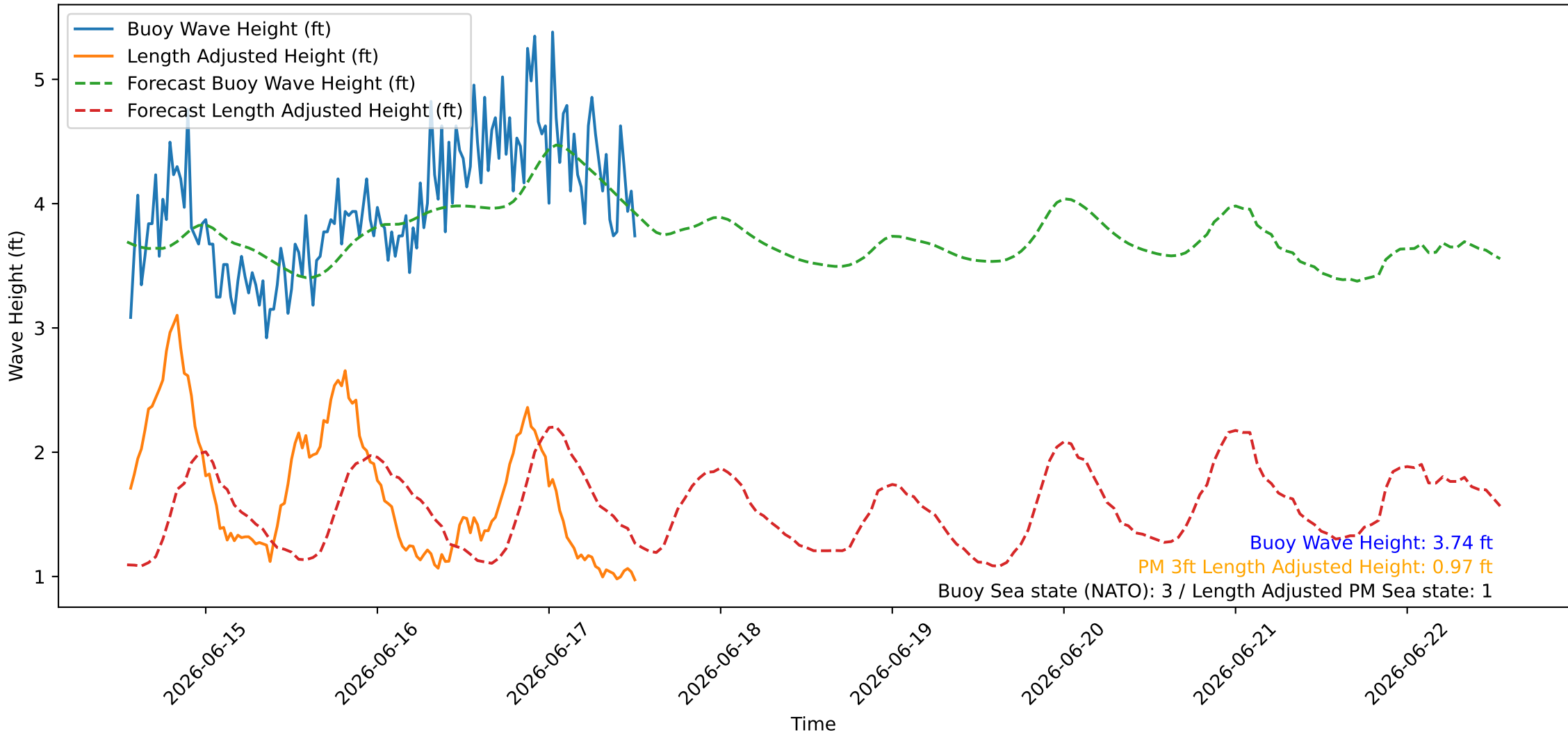
Wave Heights over Time for Red Beach at 2026-06-17 13:10:45
