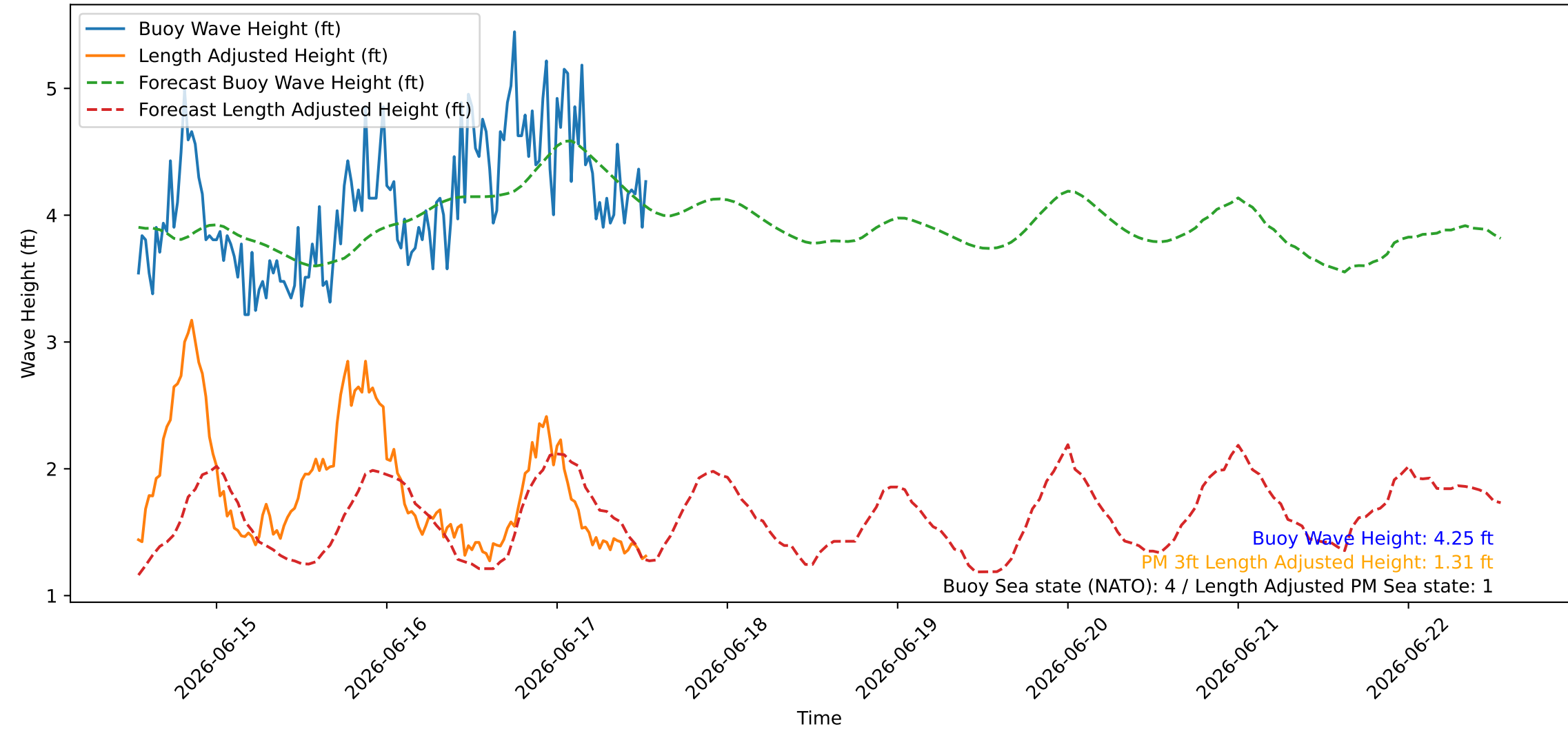
Wave Heights over Time for Oceanside Harbor at 2026-06-17 13:10:26
