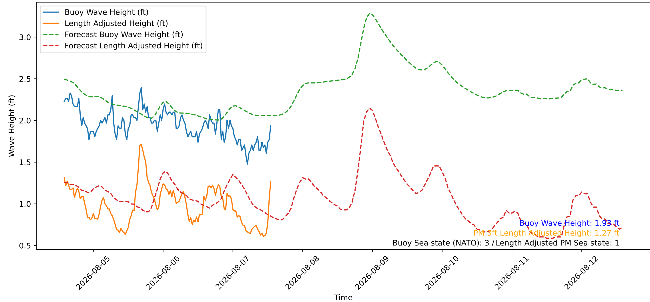
Wave Heights over Time for Red Beach at 2026-08-07 13:50:47
