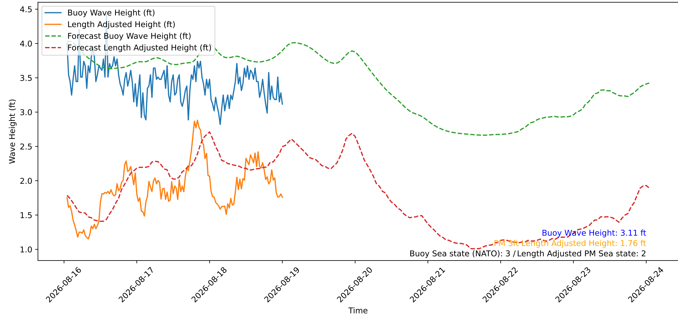
Wave Heights over Time for Oceanside Harbor at 2026-08-19 00:50:26
