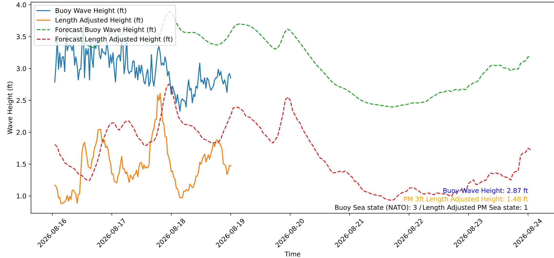
Wave Heights over Time for Red Beach at 2026-08-19 00:50:47
