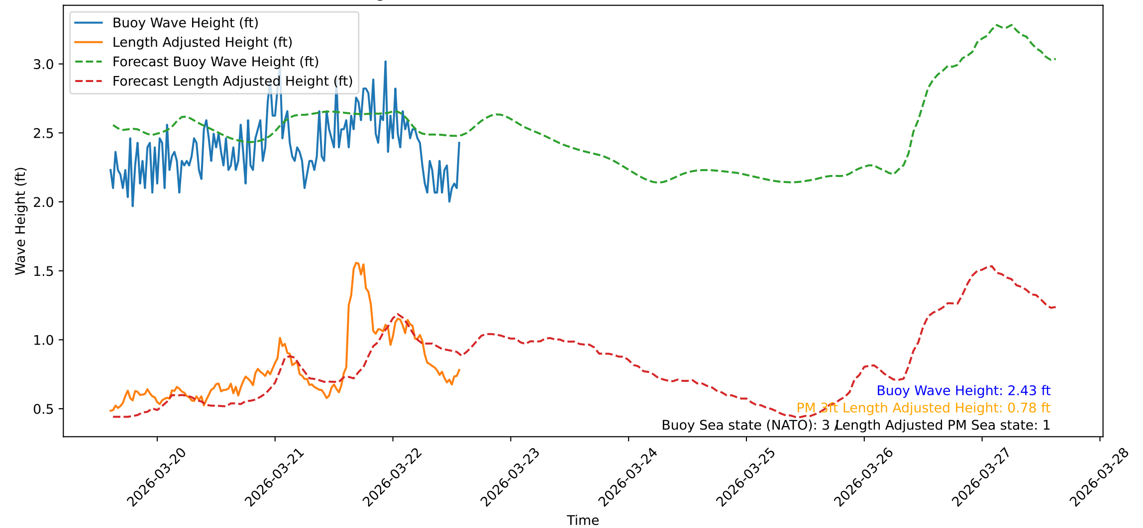
Wave Heights over Time for Oceanside Harbor at 2026-03-22 14:30:32
