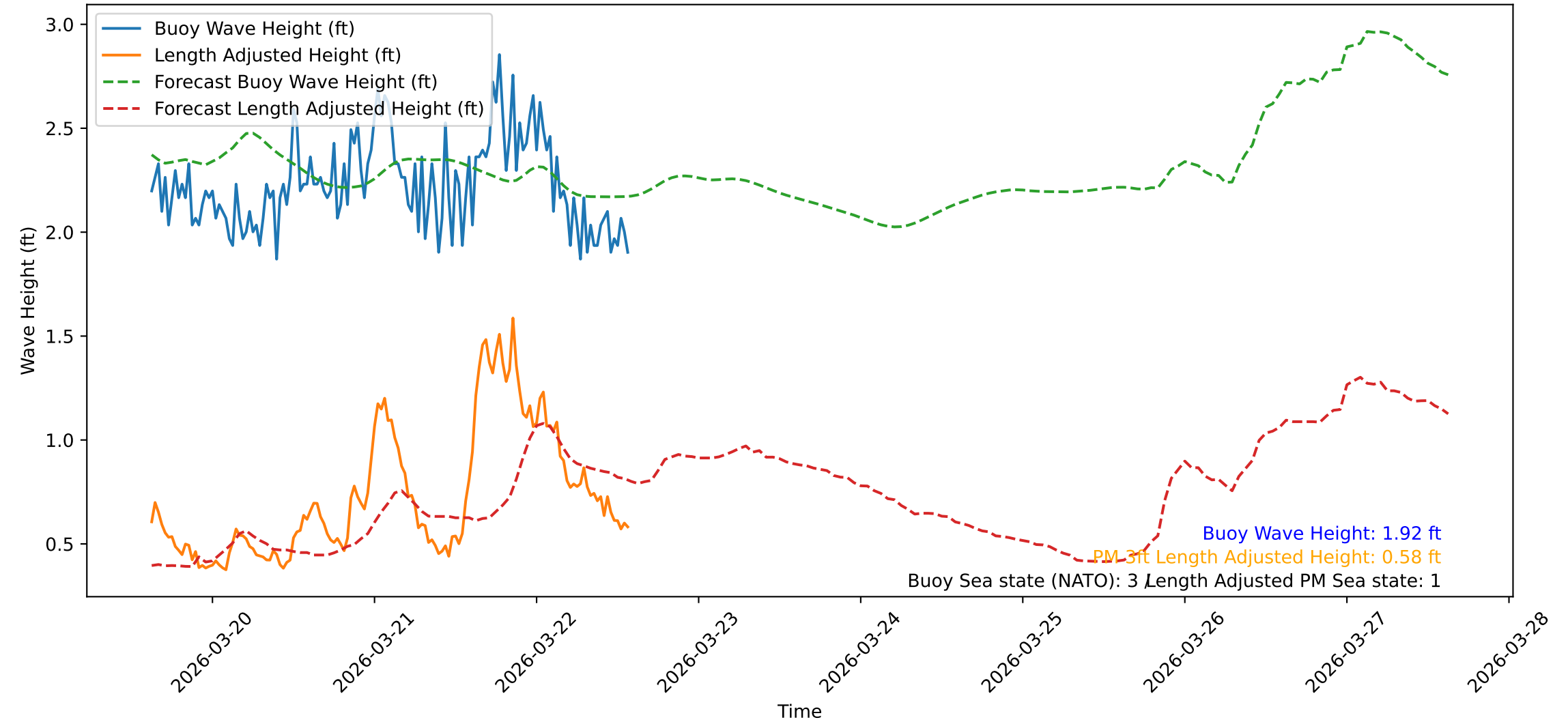
Wave Heights over Time for Red Beach at 2026-03-22 14:30:47
