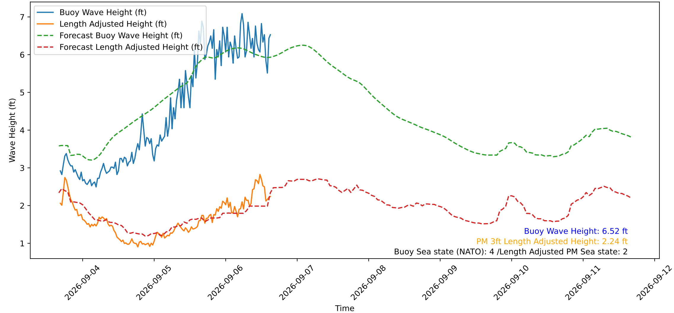
Wave Heights over Time for Green Beach at 2026-09-06 16:01:13
