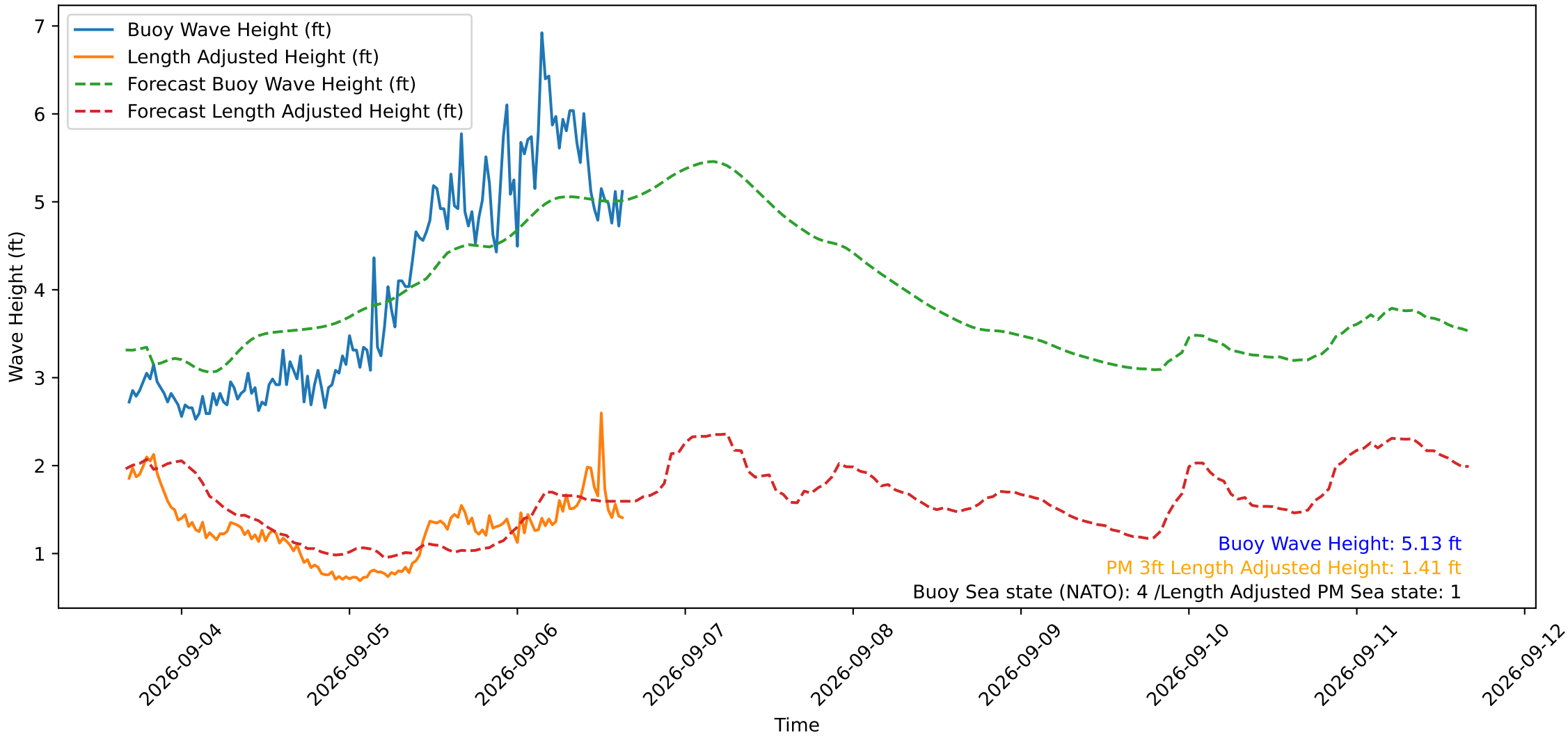
Wave Heights over Time for Red Beach at 2026-09-06 16:00:50
