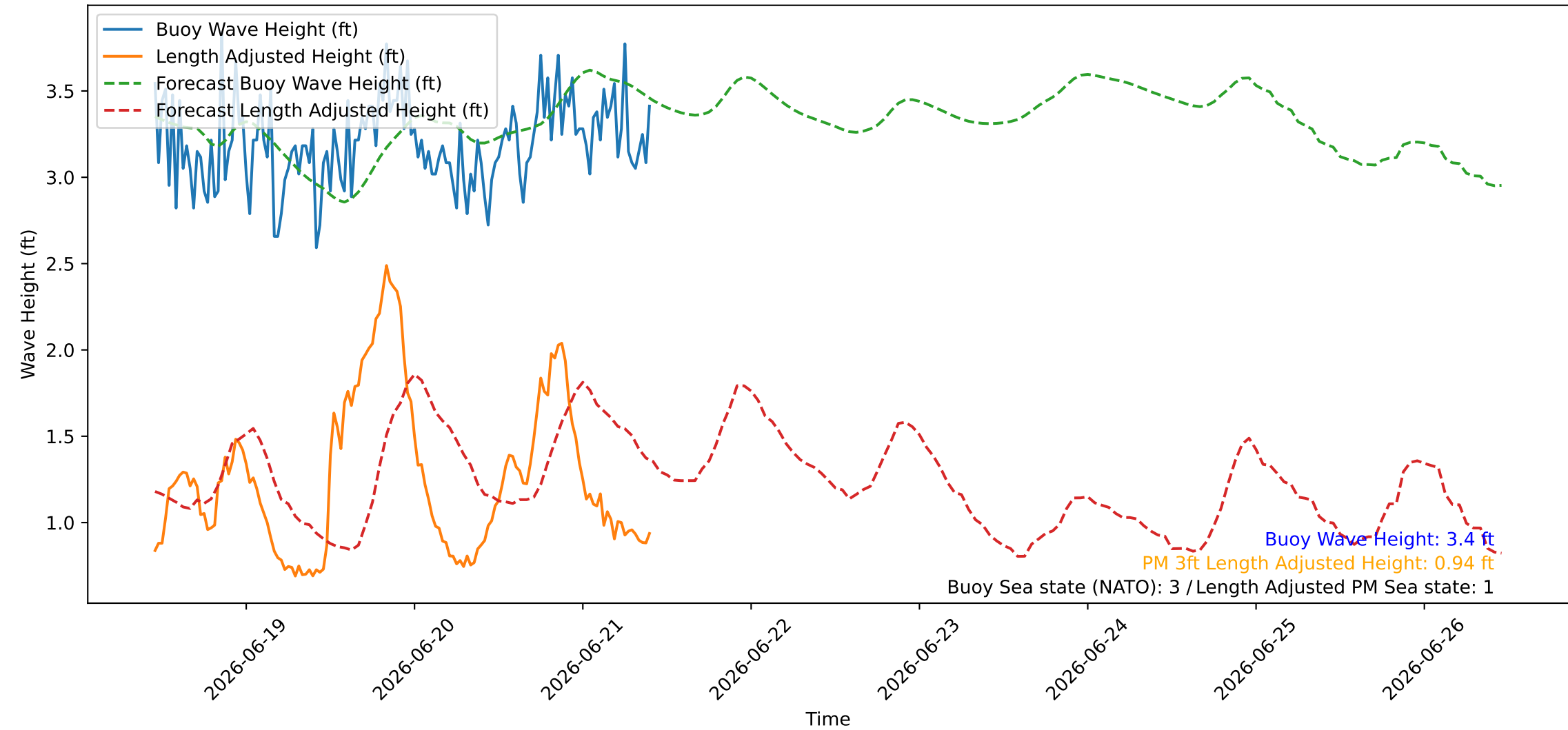
Wave Heights over Time for Red Beach at 2026-06-21 10:30:45
