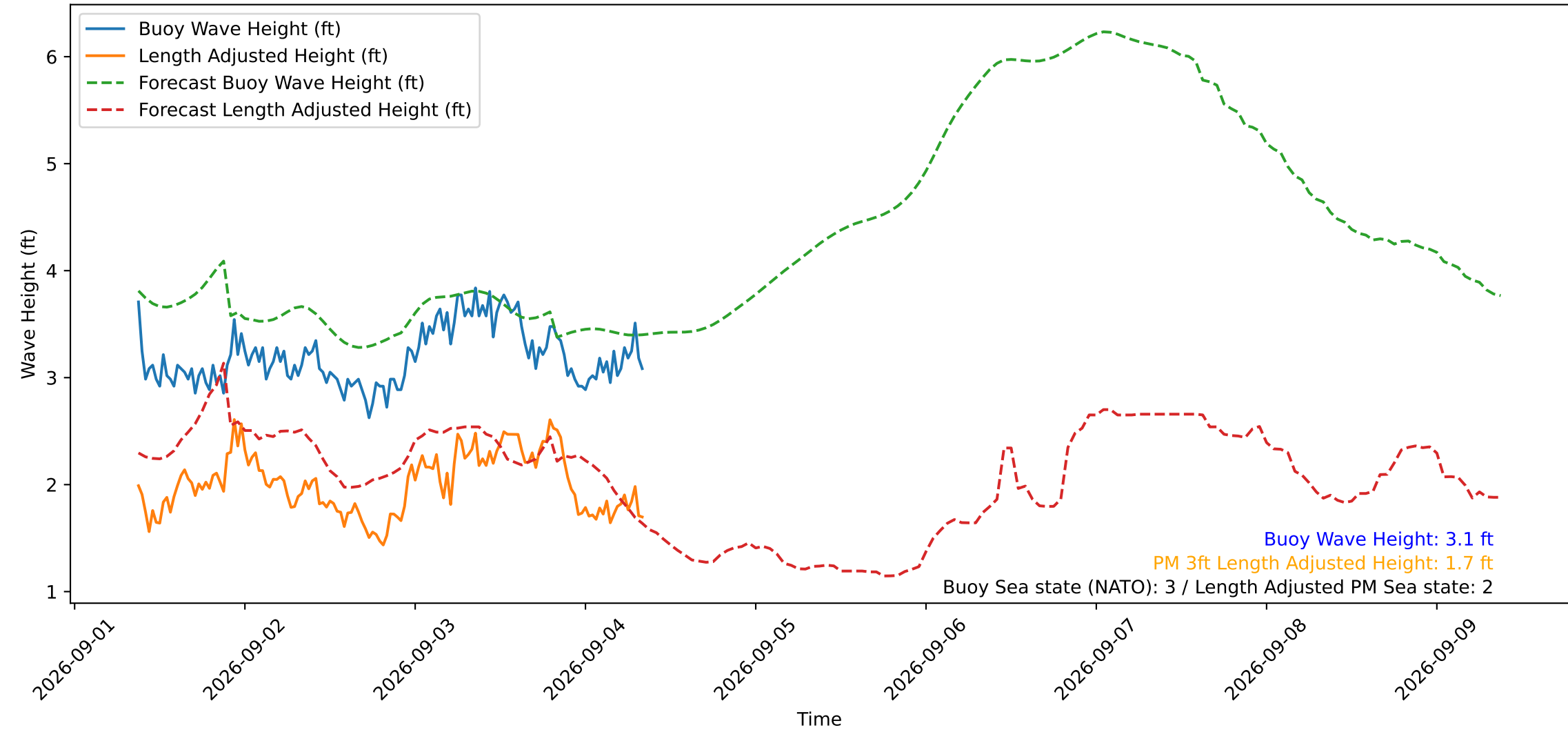
Wave Heights over Time for Oceanside Harbor at 2026-09-04 08:50:30
