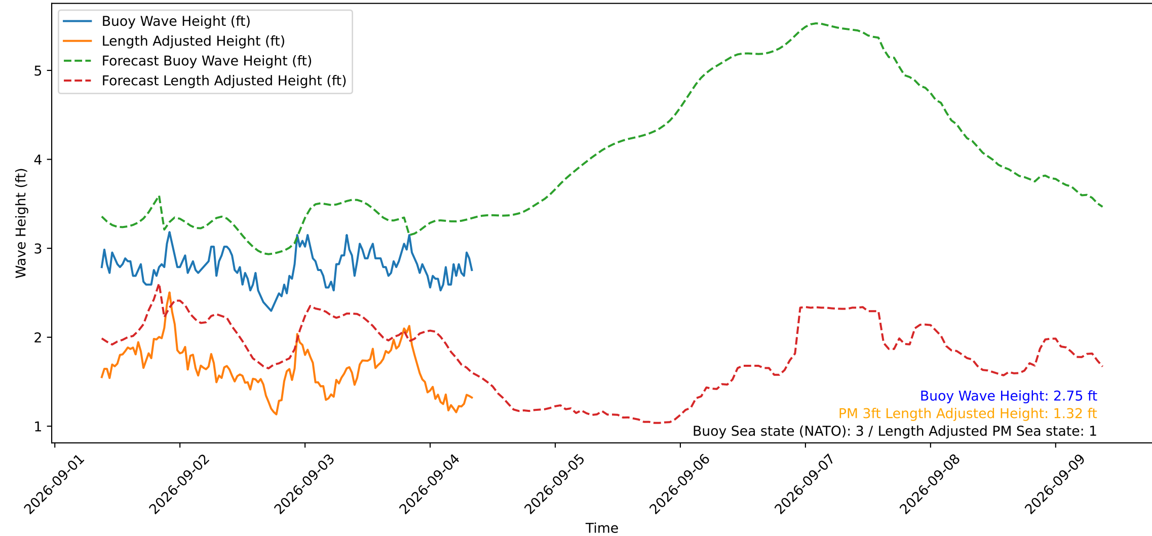
Wave Heights over Time for Red Beach at 2026-09-04 08:50:51
