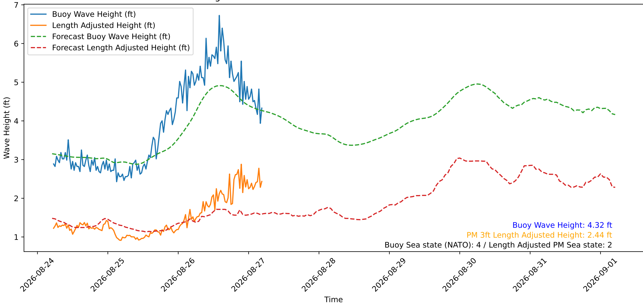
Wave Heights over Time for Oceanside Harbor at 2026-08-27 05:20:30
