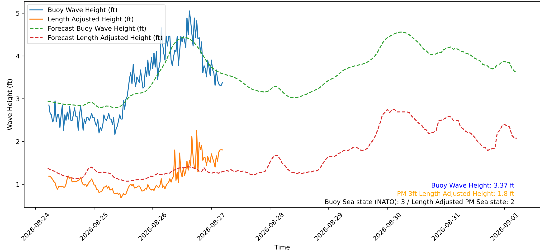
Wave Heights over Time for Red Beach at 2026-08-27 05:20:51
