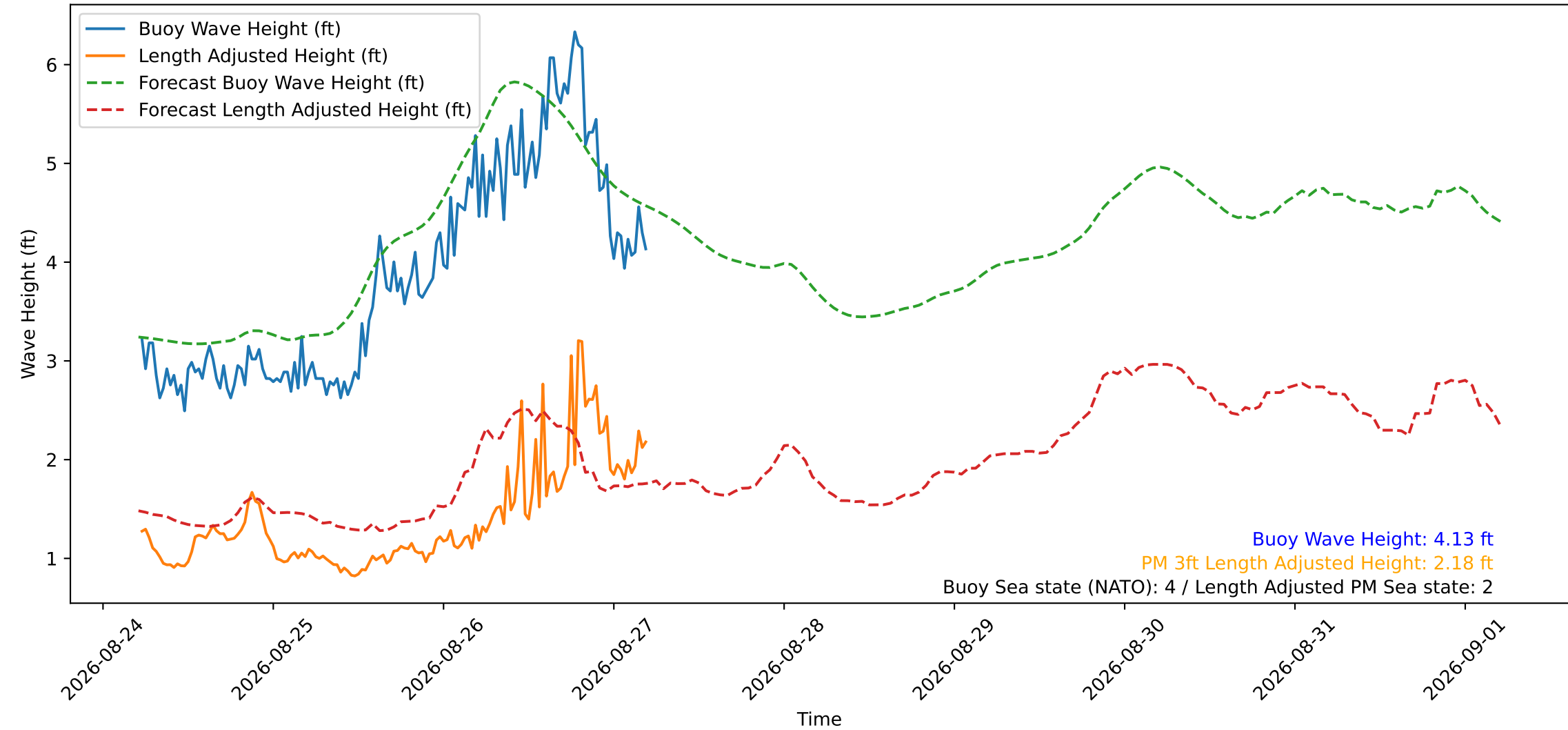
Wave Heights over Time for Green Beach at 2026-08-27 05:21:17
