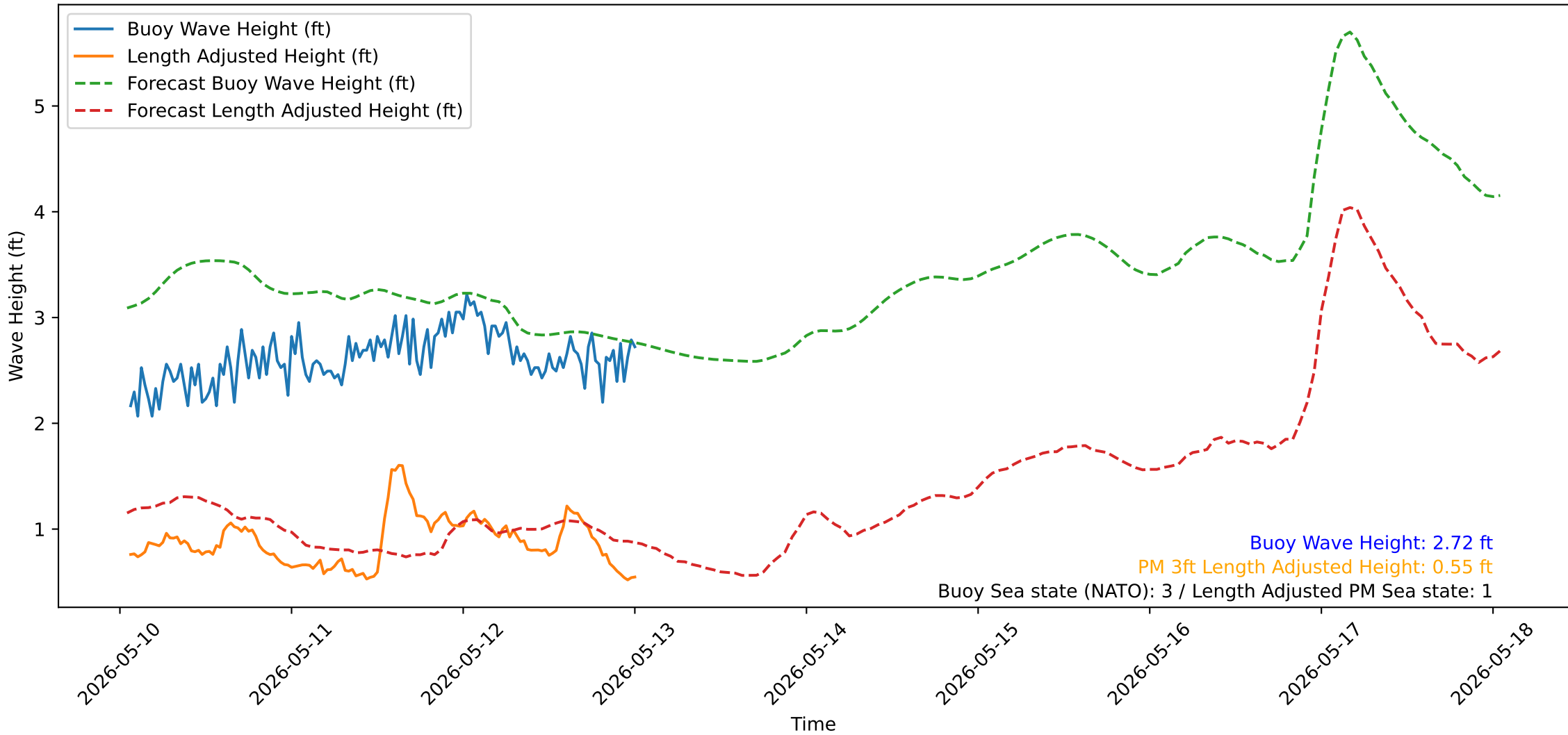
Wave Heights over Time for Red Beach at 2026-05-13 01:00:51
