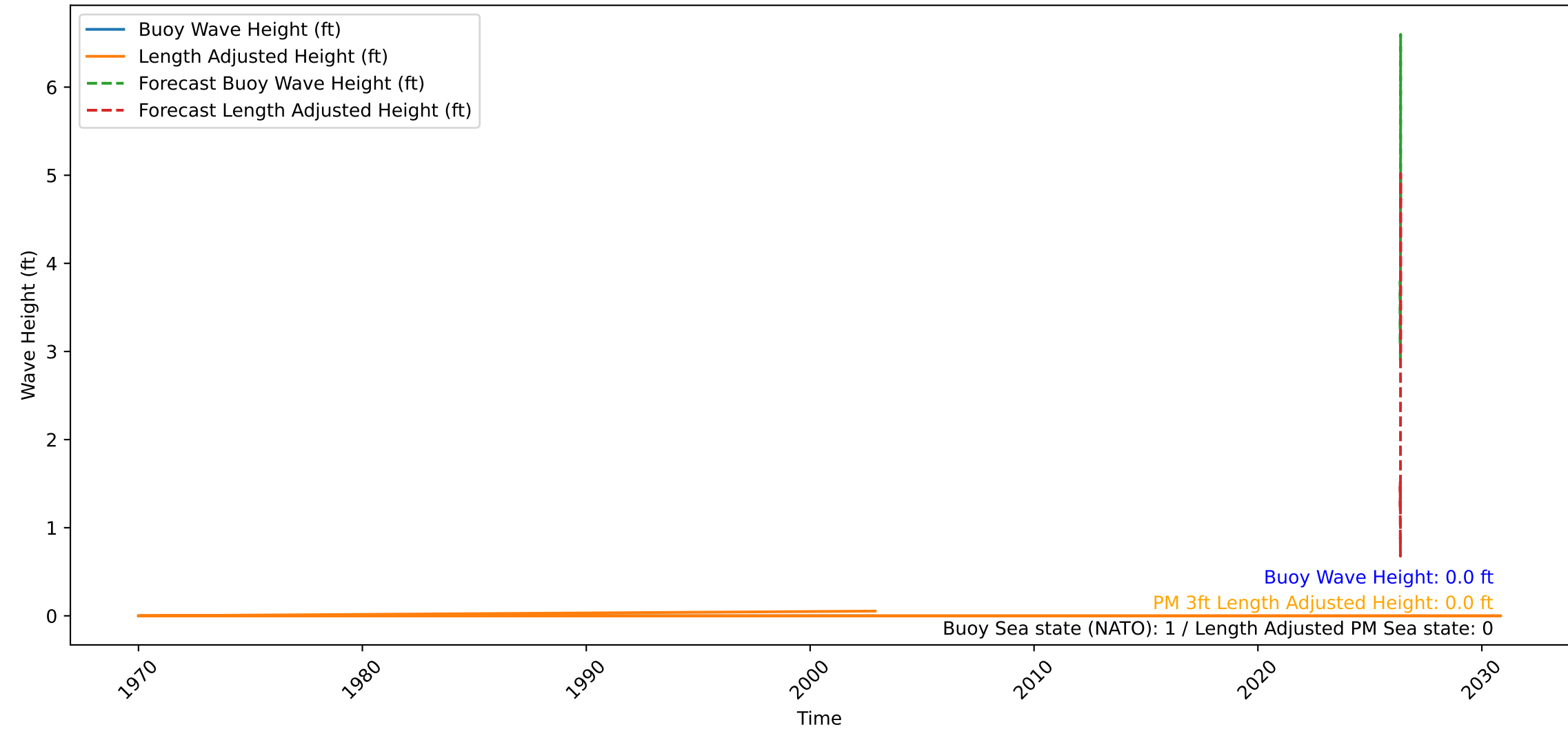
Wave Heights over Time for Oceanside Harbor at 2026-05-13 01:00:32
