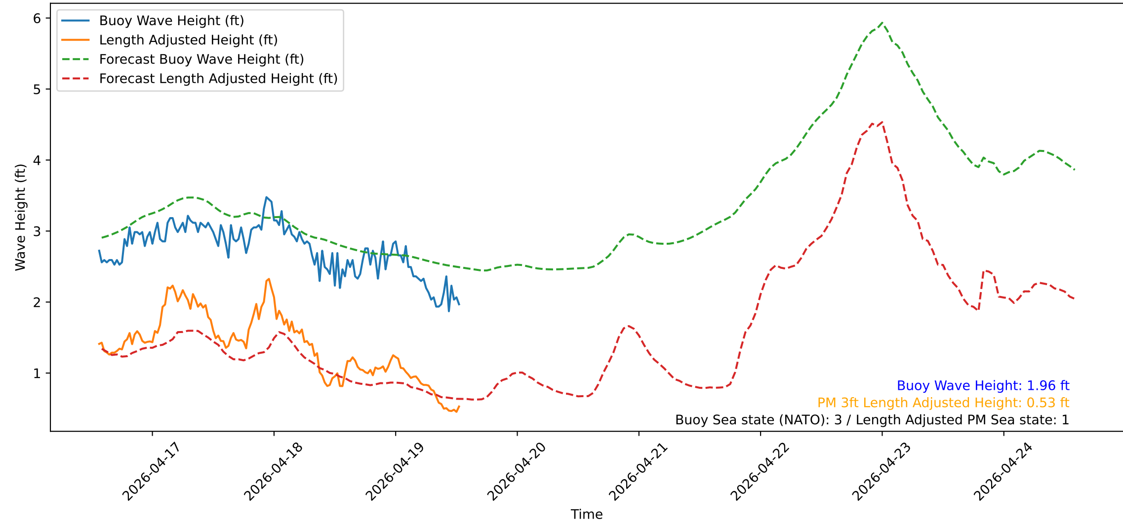
Wave Heights over Time for Green Beach at 2026-04-19 13:31:13
