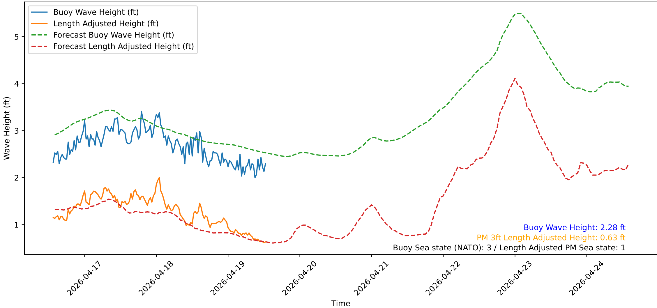
Wave Heights over Time for Oceanside Harbor at 2026-04-19 13:30:31
