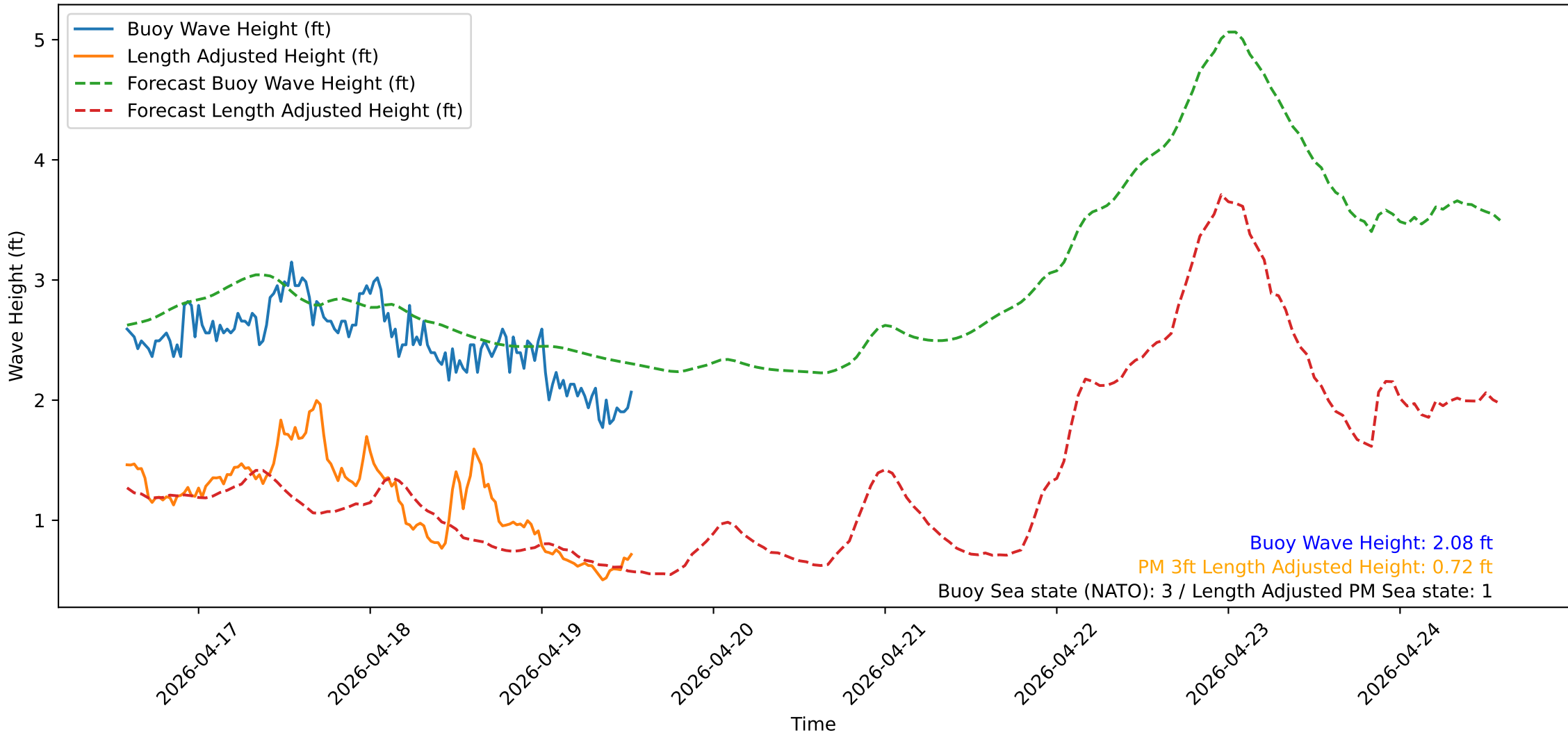
Wave Heights over Time for Red Beach at 2026-04-19 13:30:51
