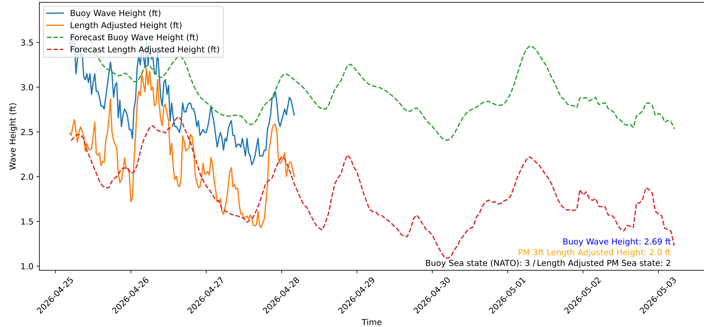
Wave Heights over Time for Green Beach at 2026-04-28 04:41:12
