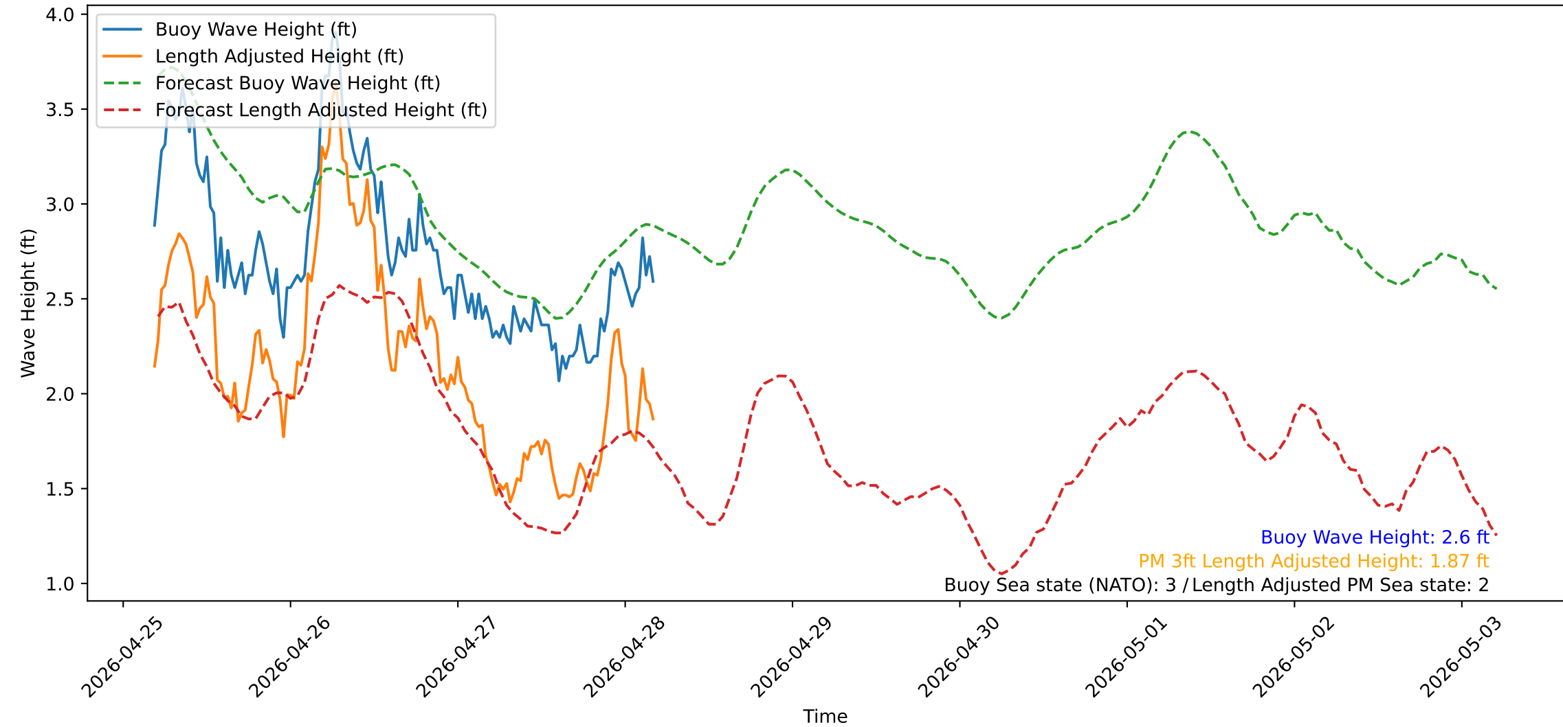
Wave Heights over Time for Oceanside Harbor at 2026-04-28 04:40:31
