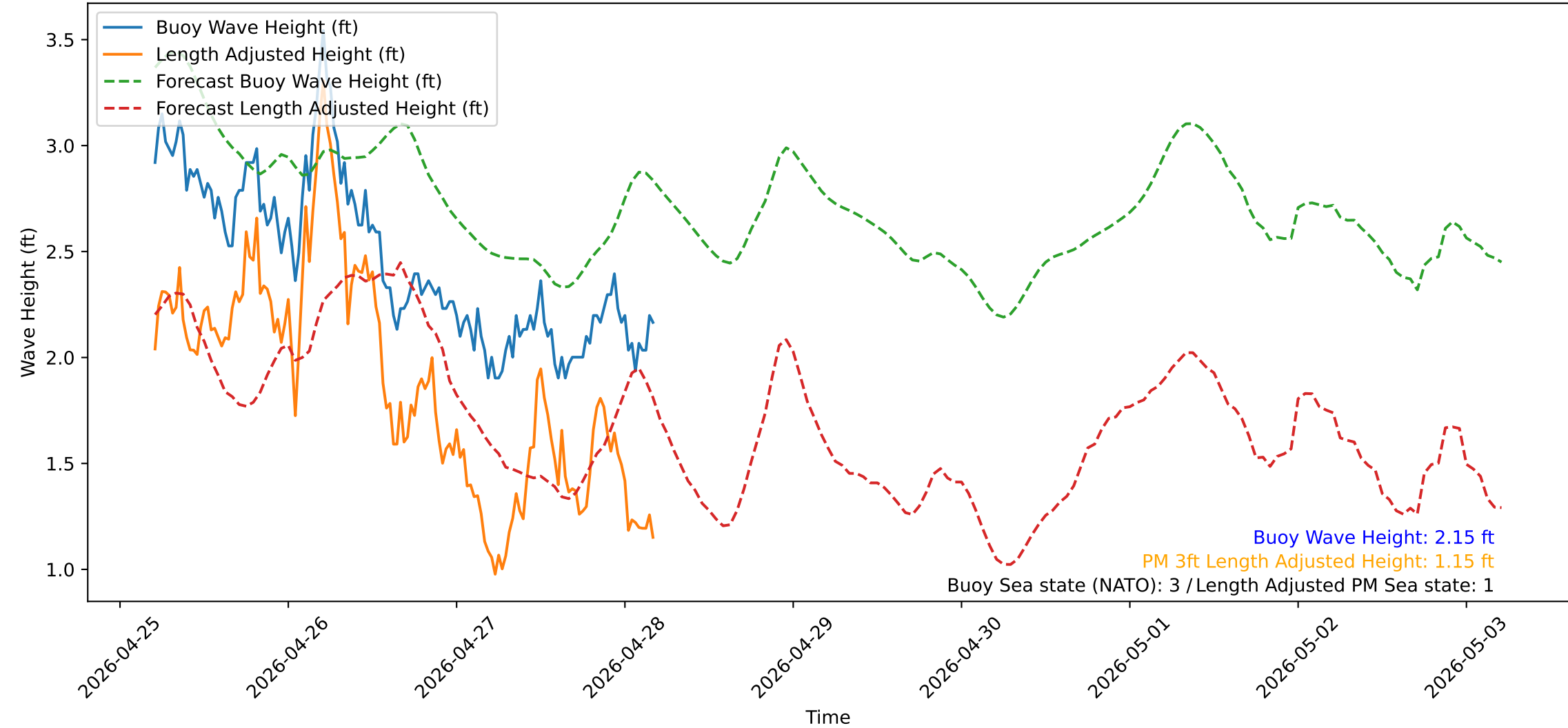
Wave Heights over Time for Red Beach at 2026-04-28 04:40:50
