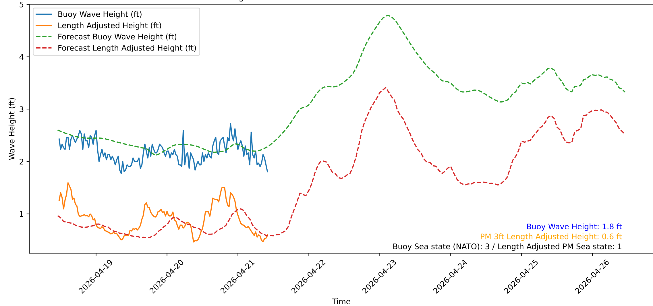
Wave Heights over Time for Red Beach at 2026-04-21 11:00:52
