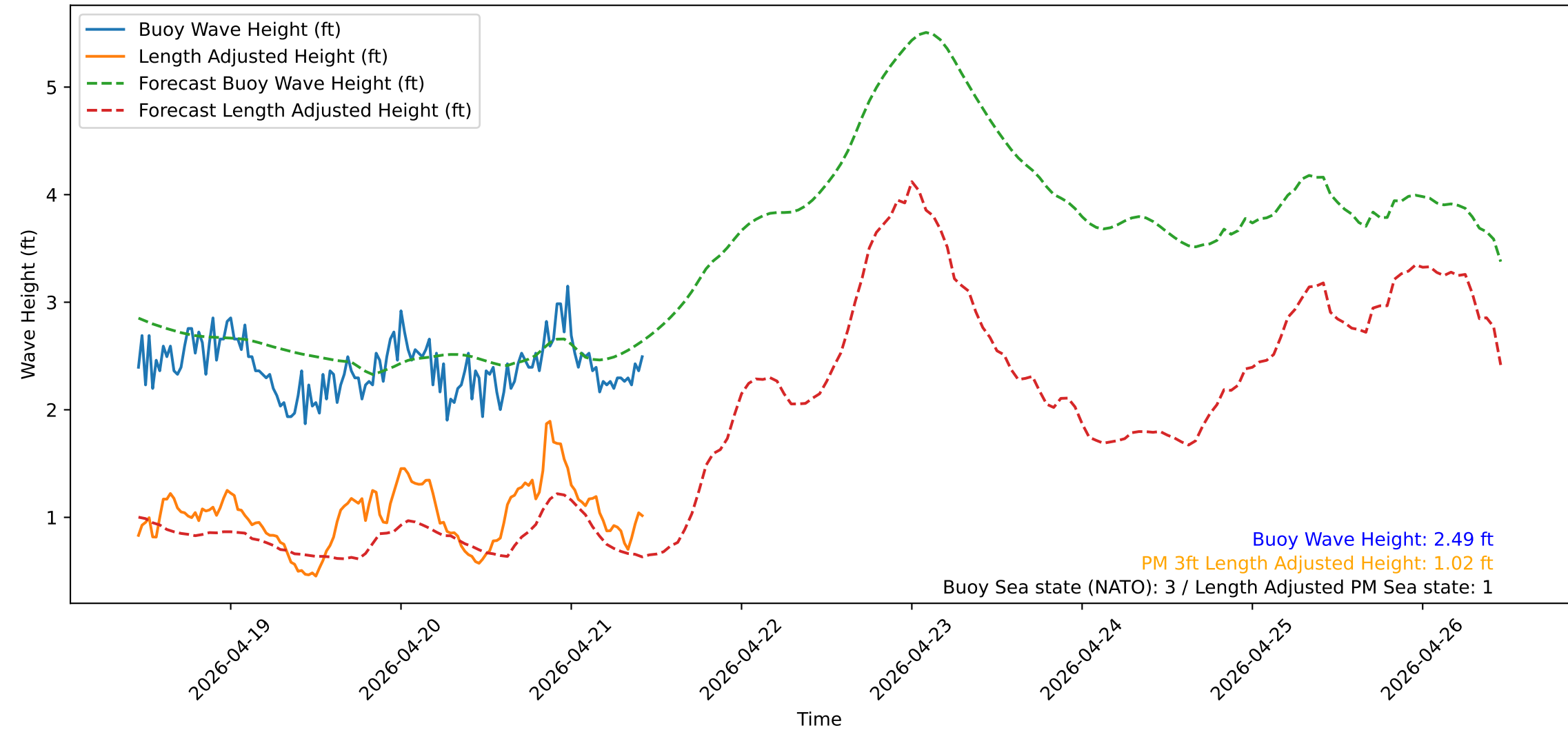
Wave Heights over Time for Green Beach at 2026-04-21 11:01:15
