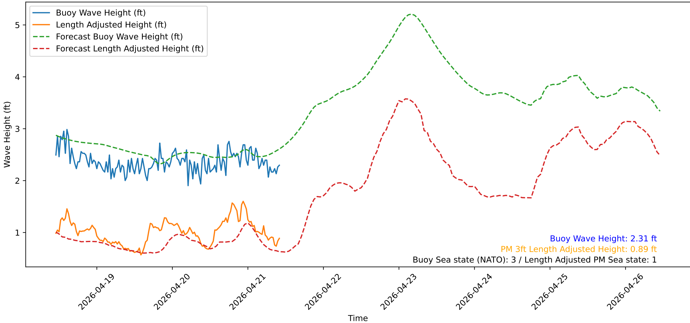
Wave Heights over Time for Oceanside Harbor at 2026-04-21 11:00:33
