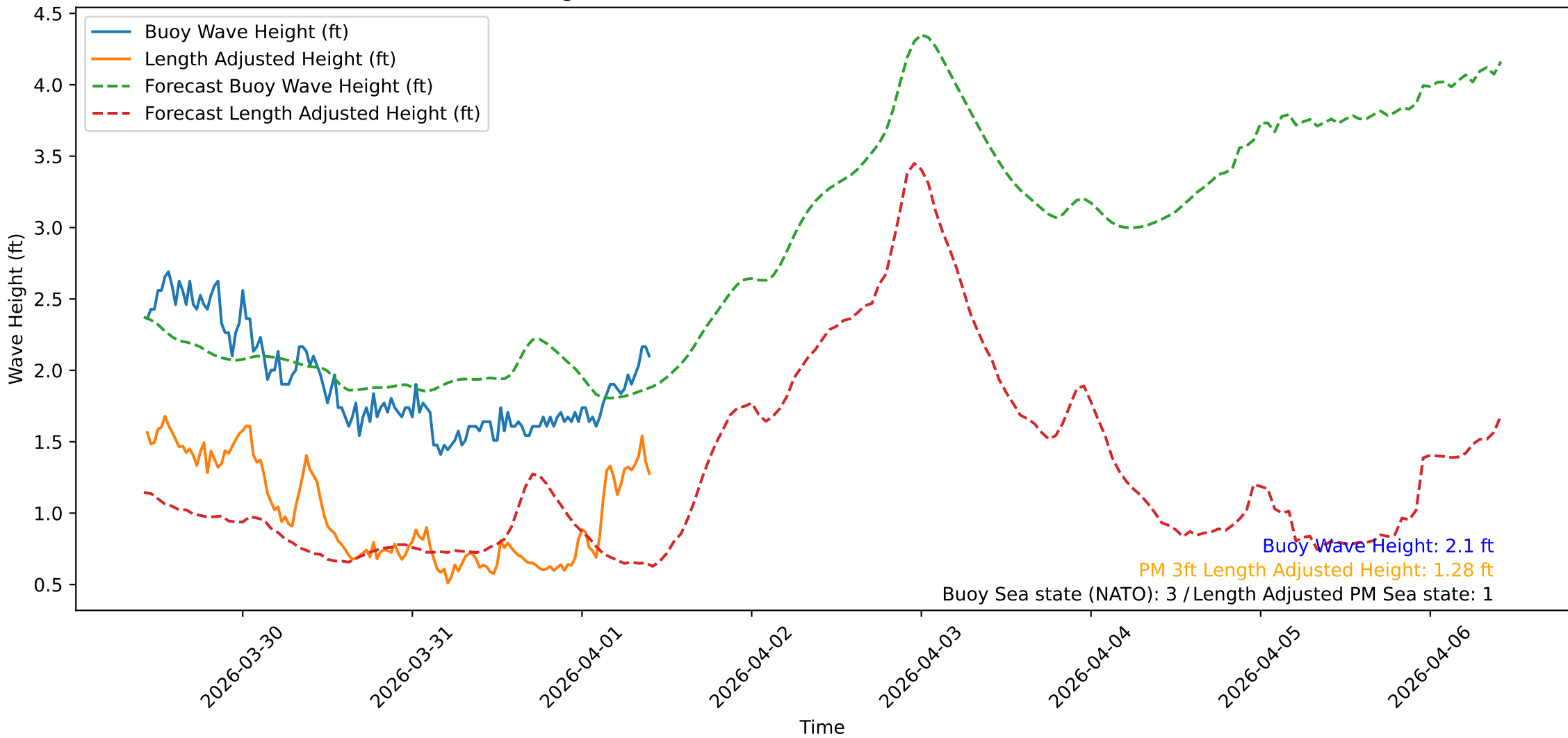
Wave Heights over Time for Green Beach at 2026-04-01 10:21:08
