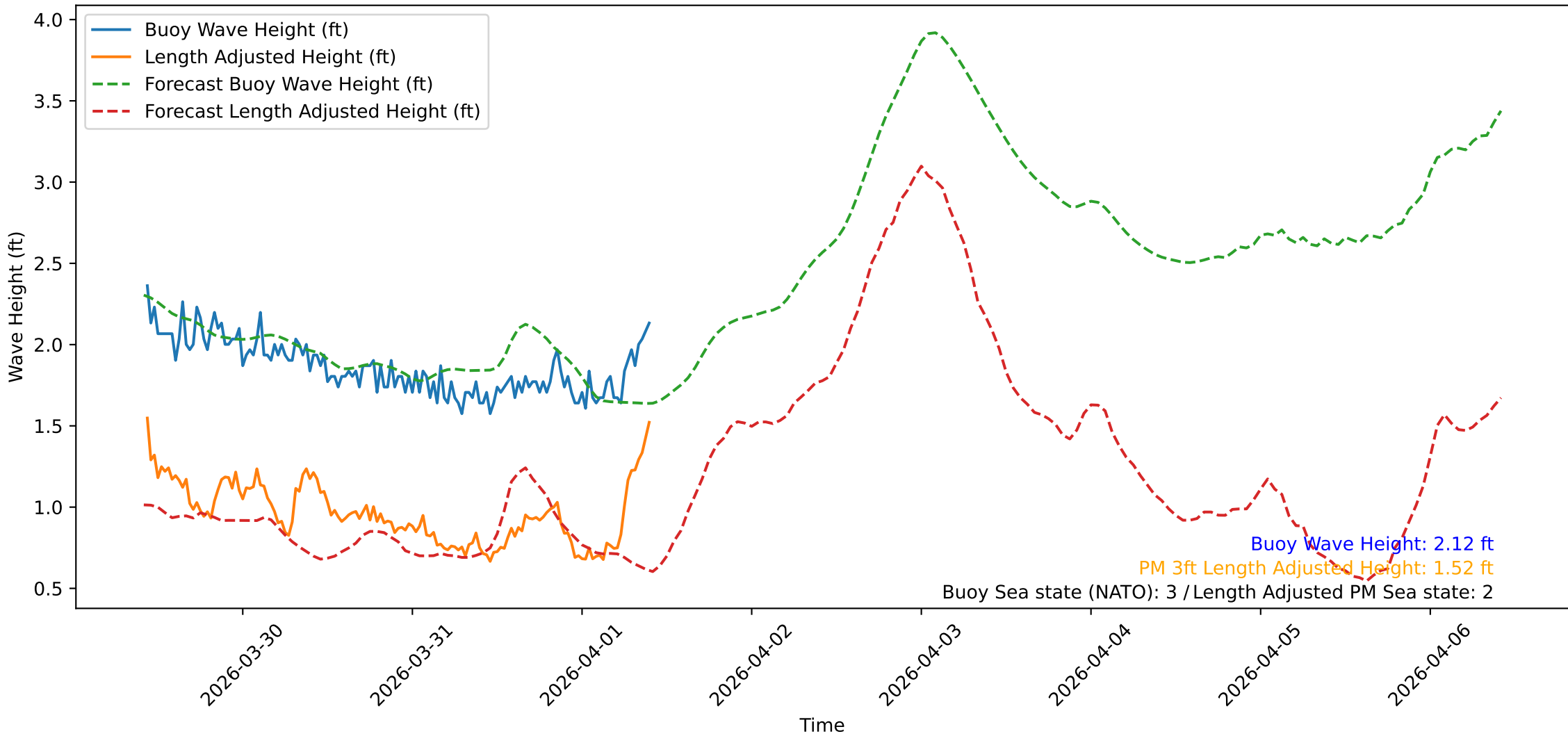
Wave Heights over Time for Oceanside Harbor at 2026-04-01 10:20:31
