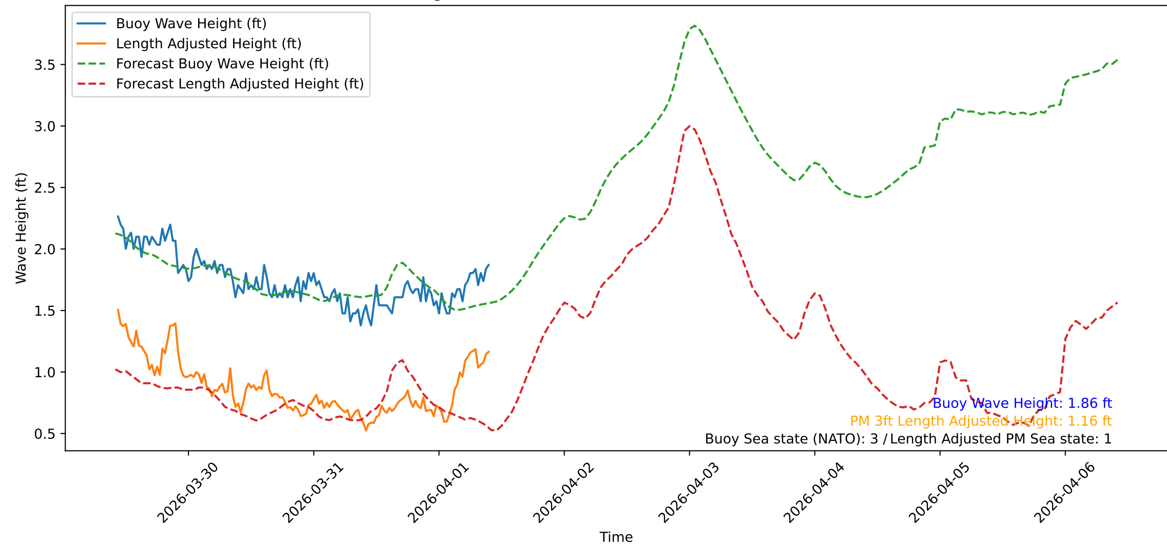
Wave Heights over Time for Red Beach at 2026-04-01 10:20:46
