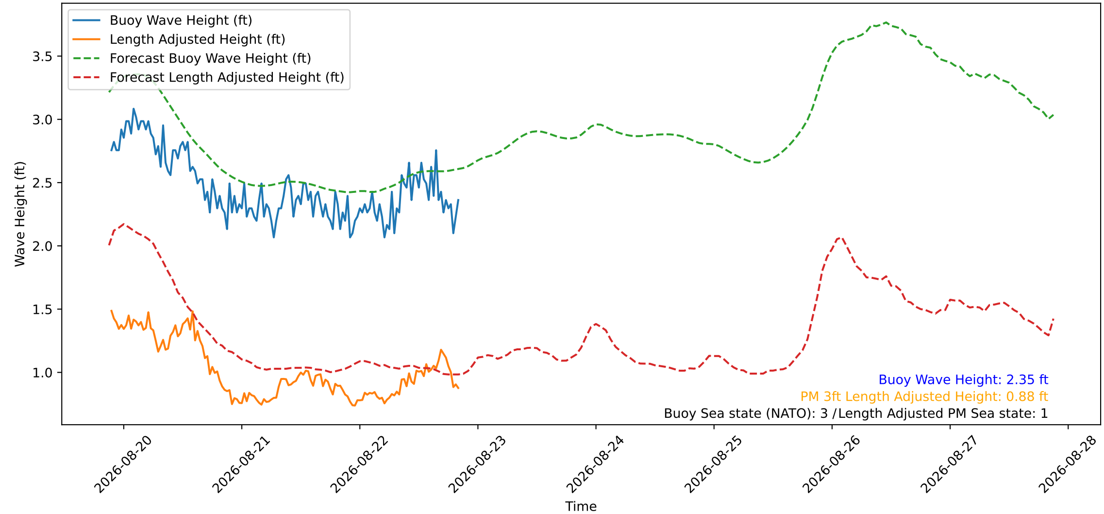
Wave Heights over Time for Red Beach at 2026-08-22 21:00:49
