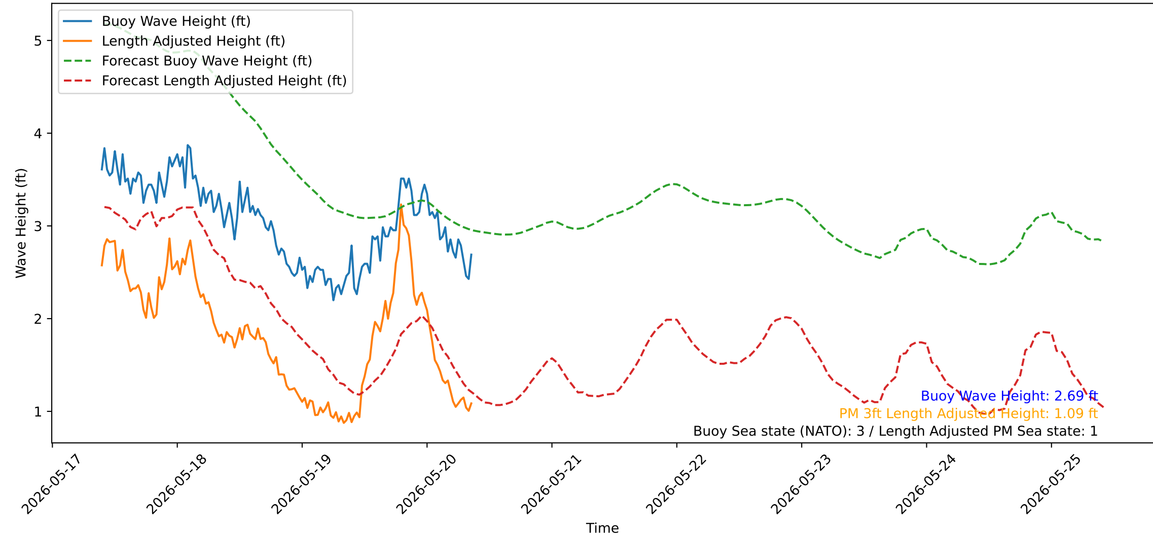
Wave Heights over Time for Oceanside Harbor at 2026-05-20 09:30:32
