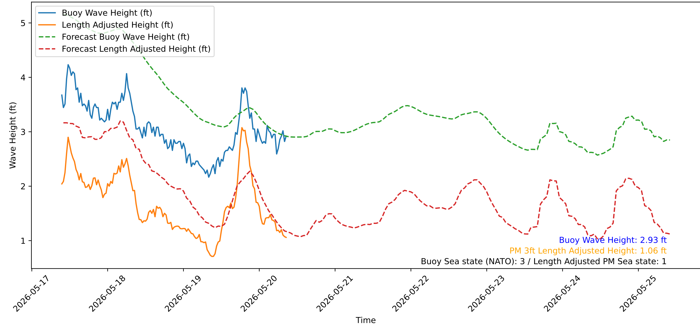
Wave Heights over Time for Green Beach at 2026-05-20 09:31:14
