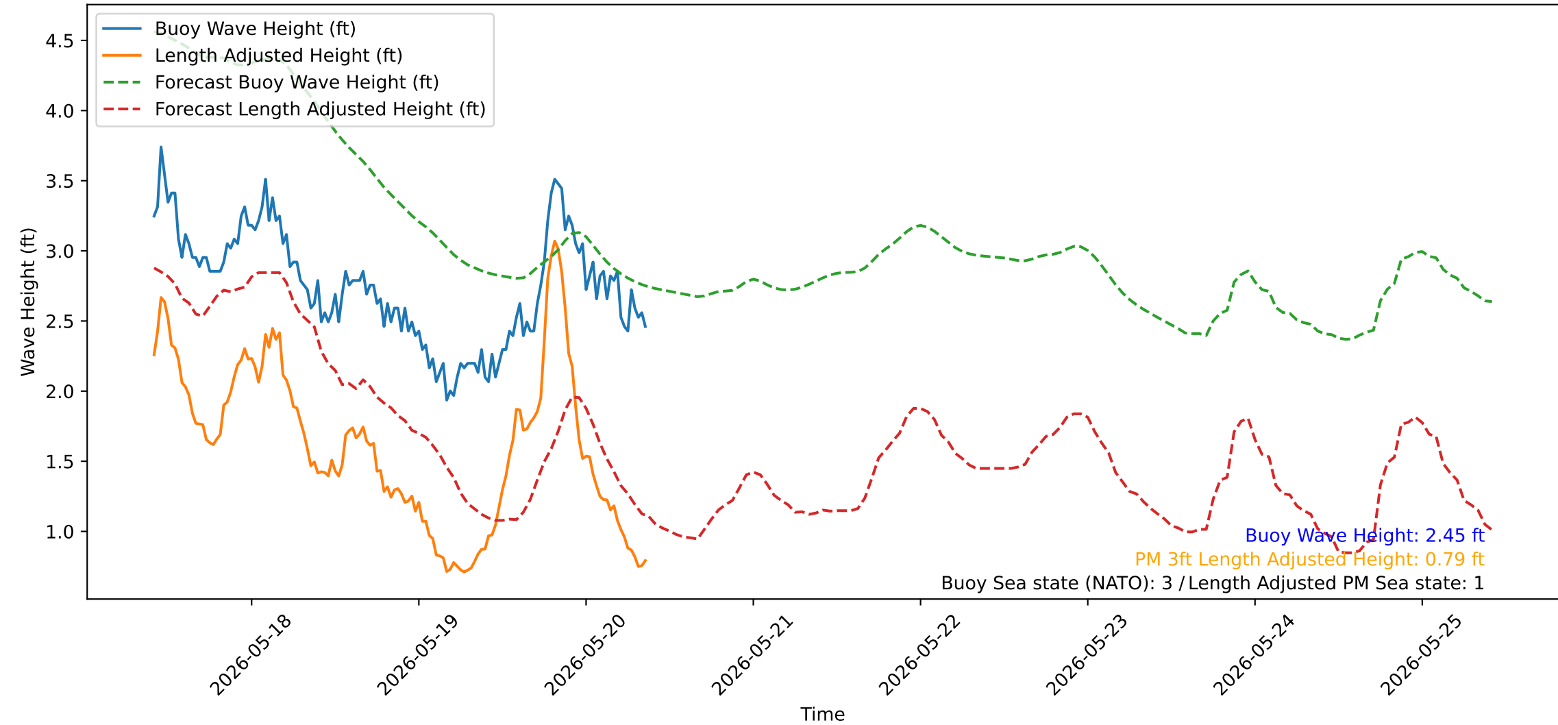
Wave Heights over Time for Red Beach at 2026-05-20 09:30:51
