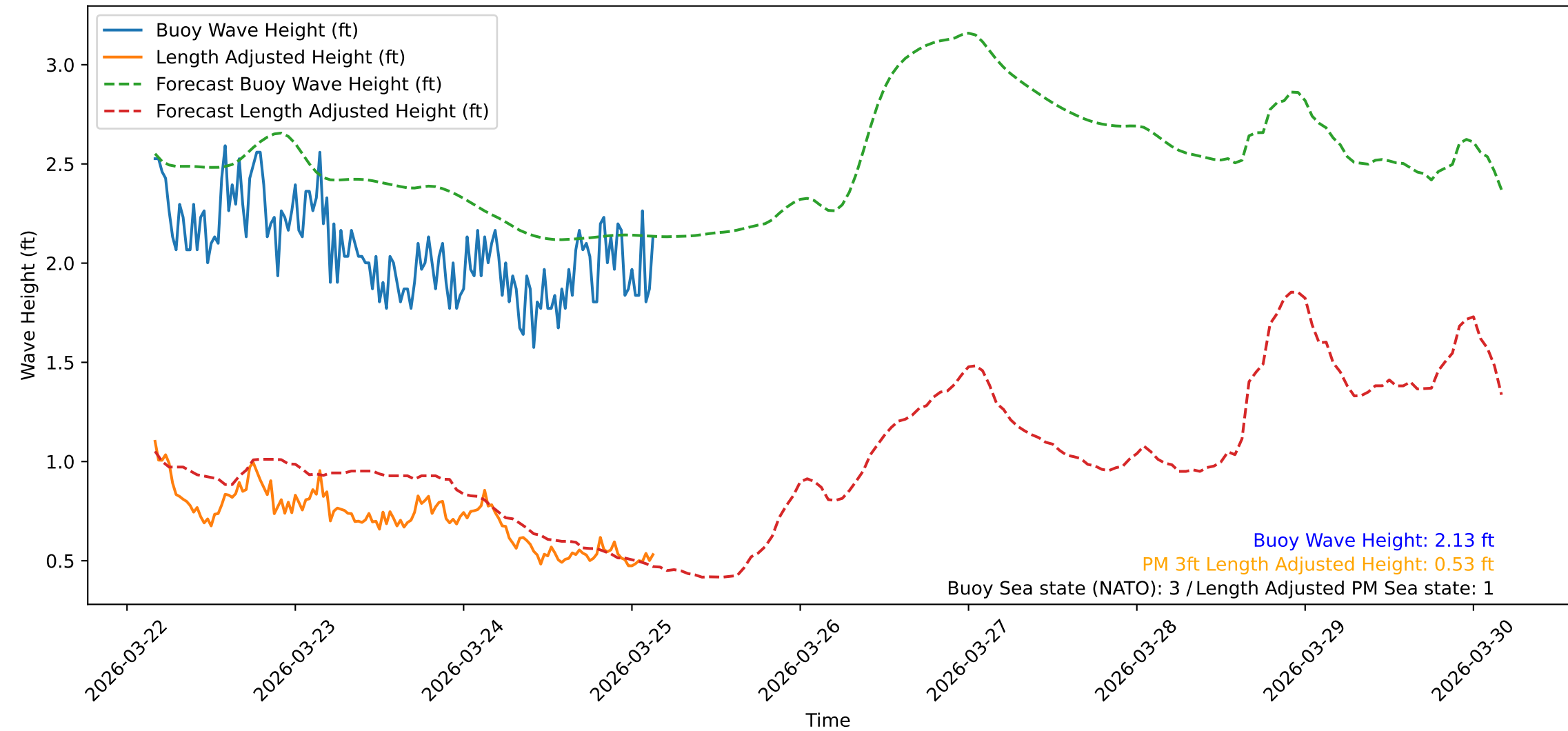
Wave Heights over Time for Oceanside Harbor at 2026-03-25 03:50:31
