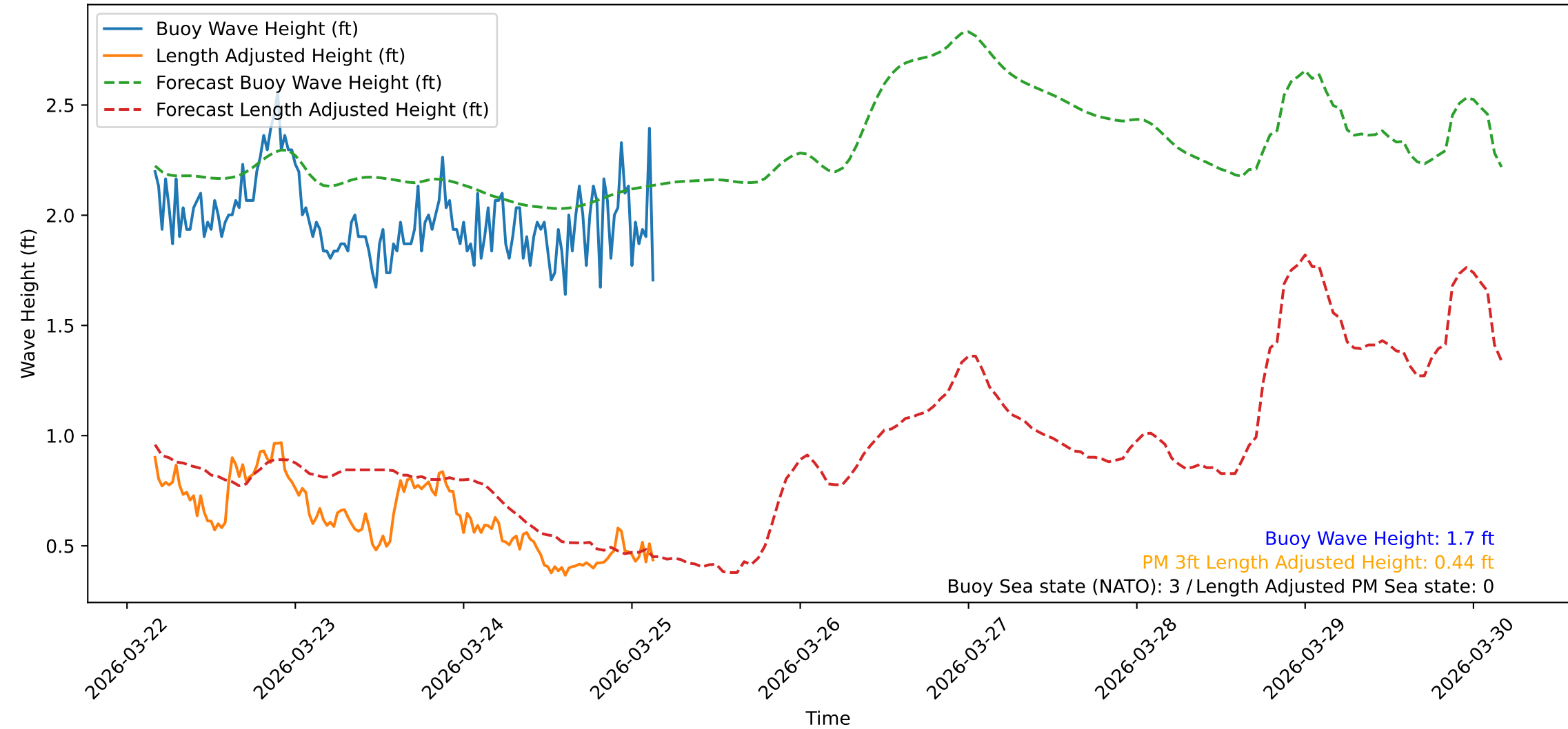
Wave Heights over Time for Red Beach at 2026-03-25 03:50:48
