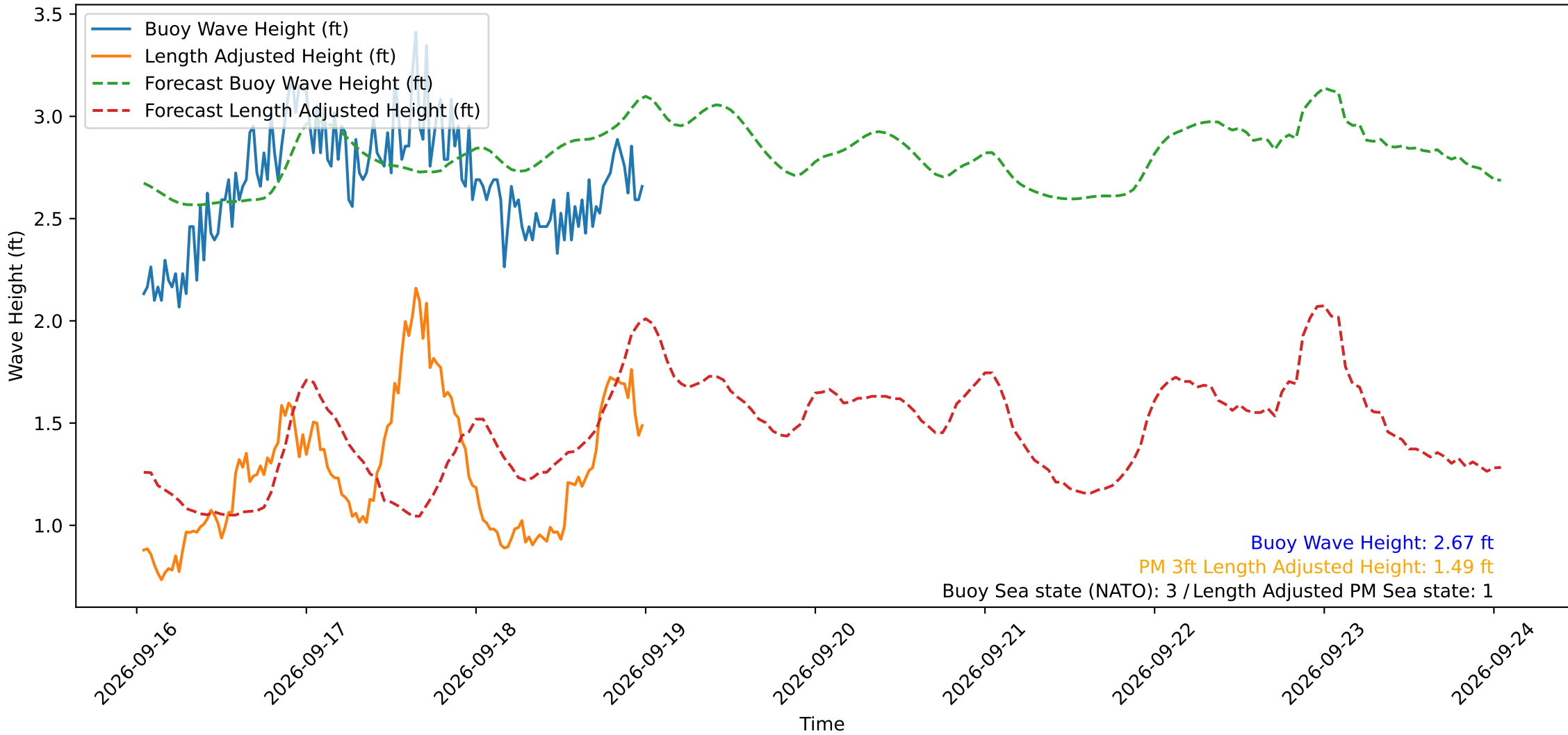
Wave Heights over Time for Red Beach at 2026-09-19 00:30:50
