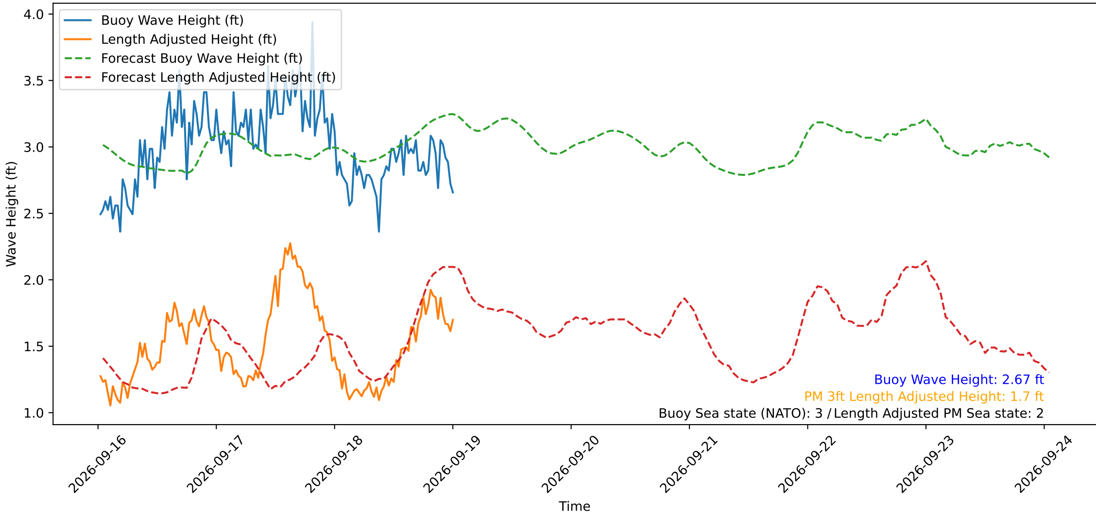
Wave Heights over Time for Oceanside Harbor at 2026-09-19 00:30:29
