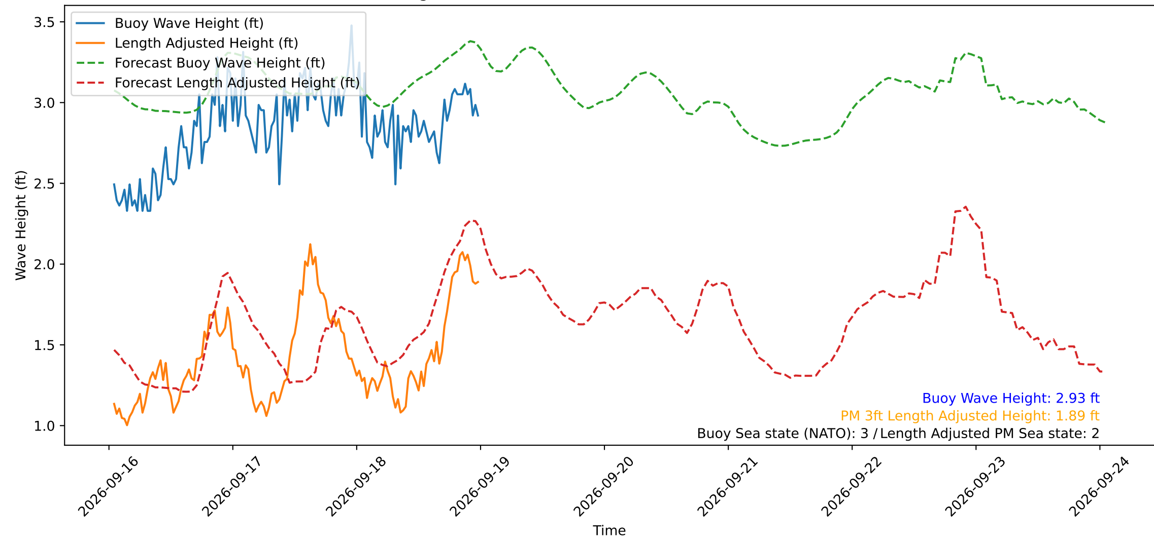
Wave Heights over Time for Green Beach at 2026-09-19 00:31:12
