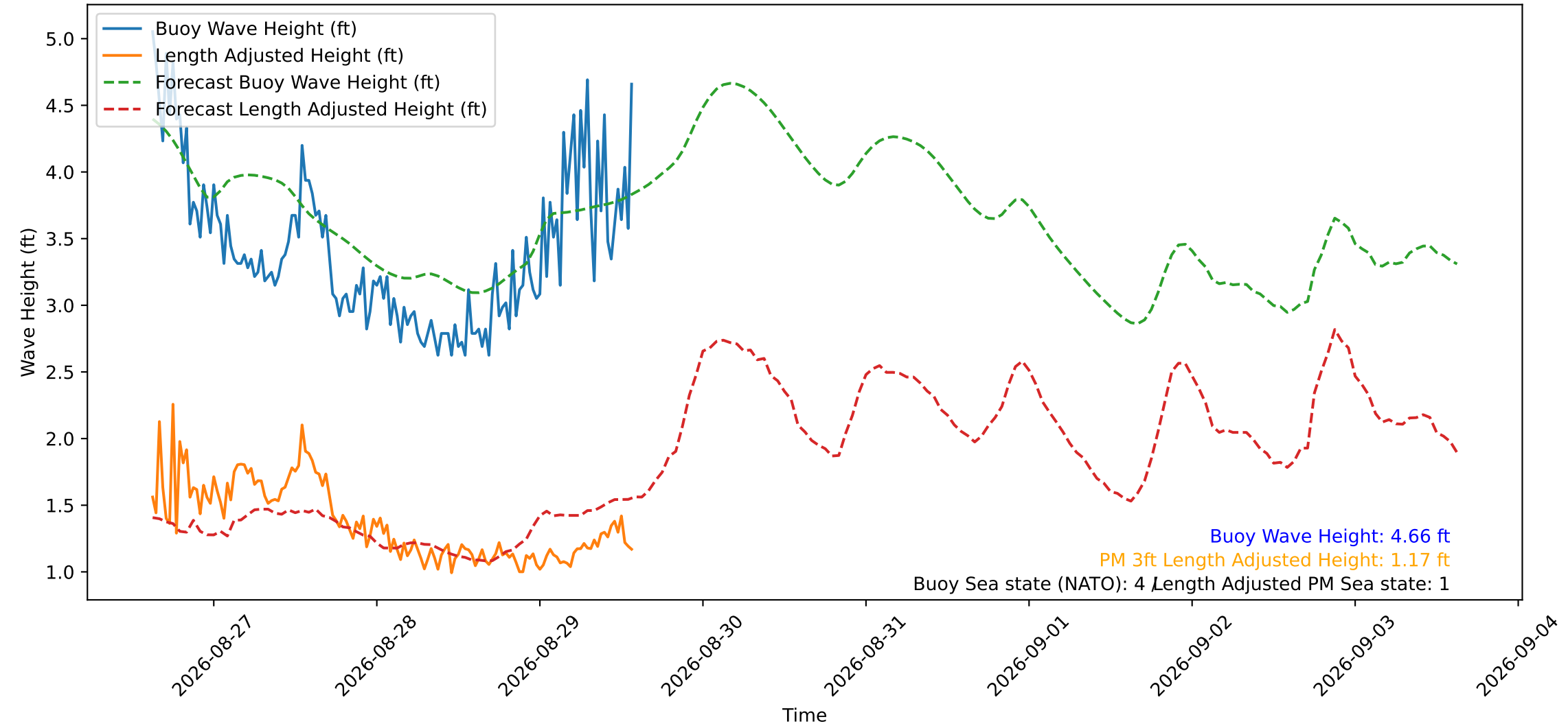
Wave Heights over Time for Red Beach at 2026-08-29 14:40:49
