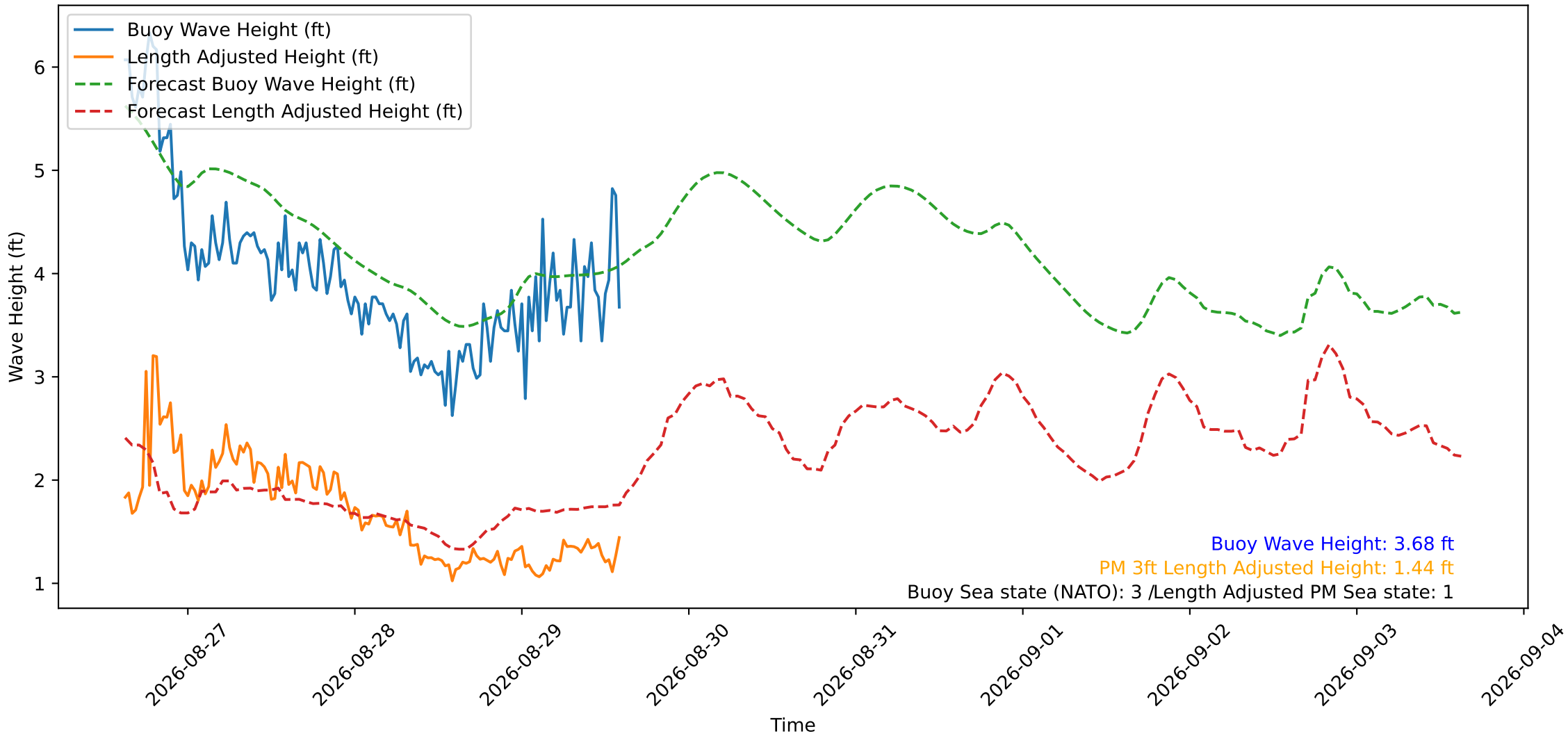
Wave Heights over Time for Green Beach at 2026-08-29 14:41:12
