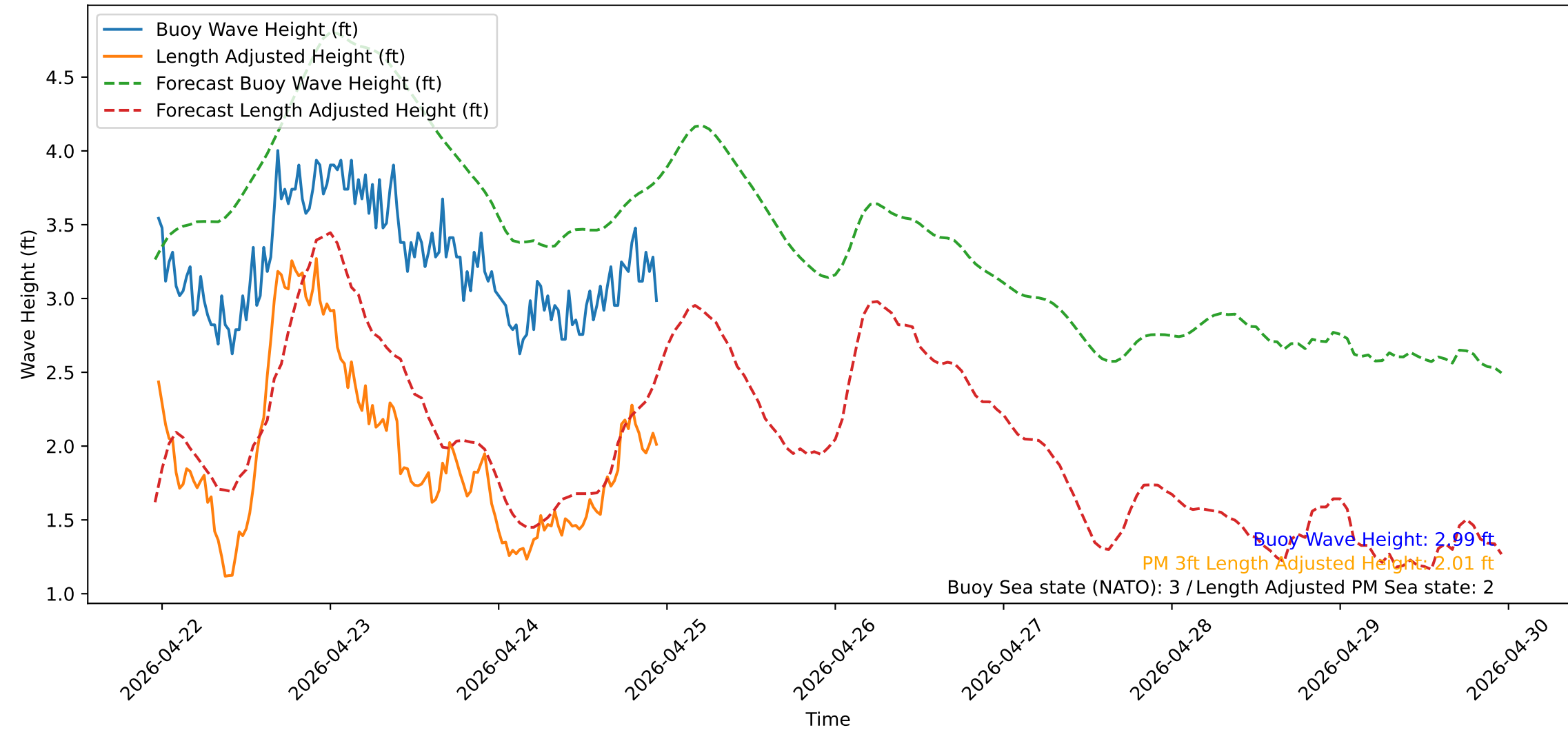
Wave Heights over Time for Green Beach at 2026-04-24 23:21:13
