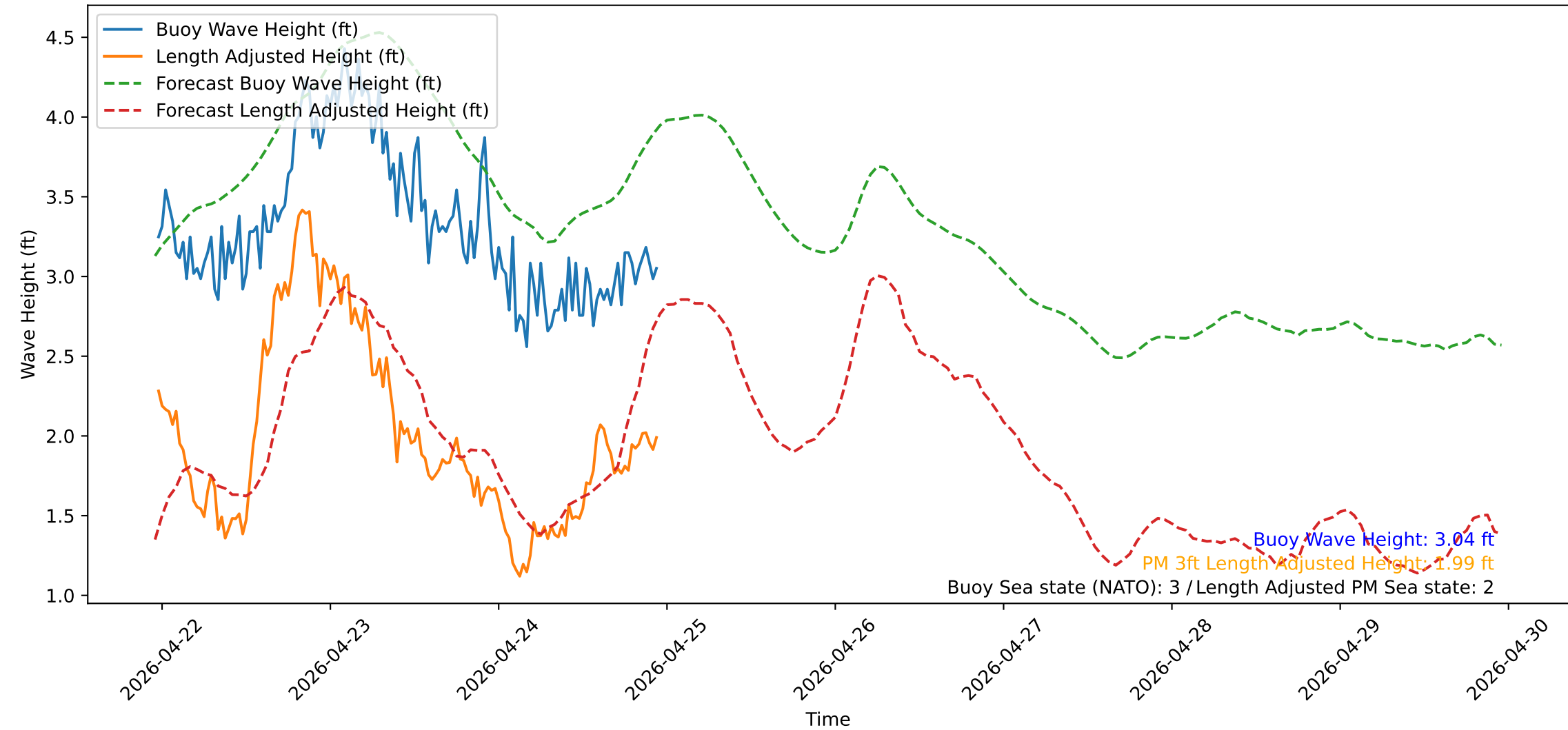
Wave Heights over Time for Oceanside Harbor at 2026-04-24 23:20:31
