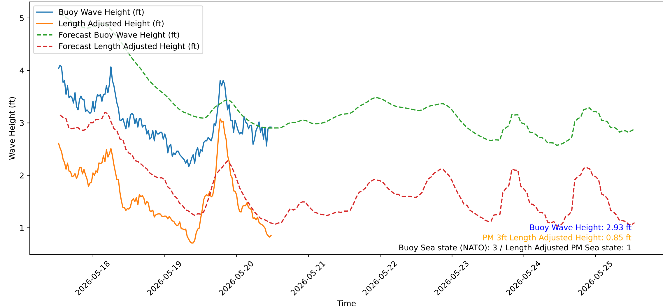
Wave Heights over Time for Green Beach at 2026-05-20 12:31:14
