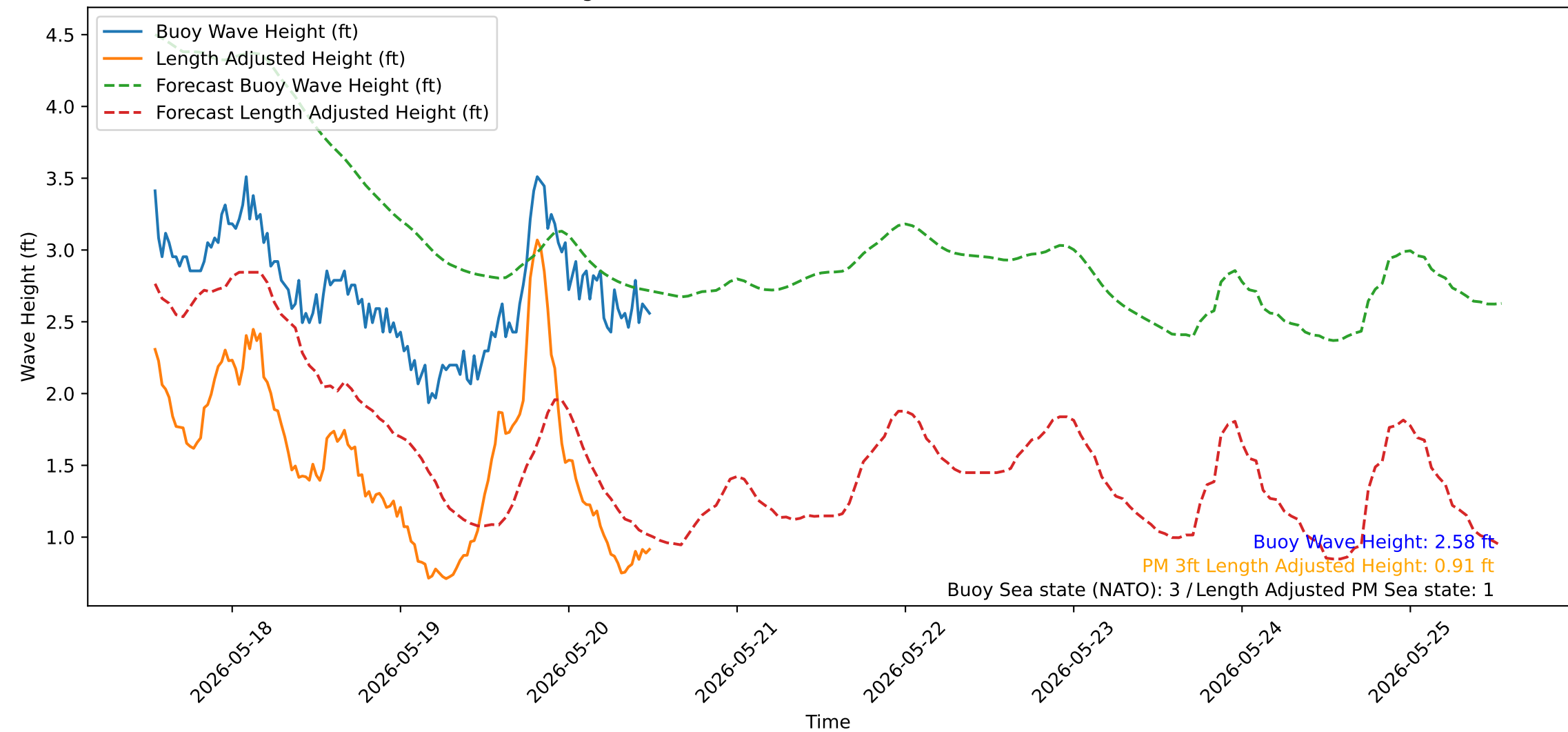
Wave Heights over Time for Red Beach at 2026-05-20 12:30:51
