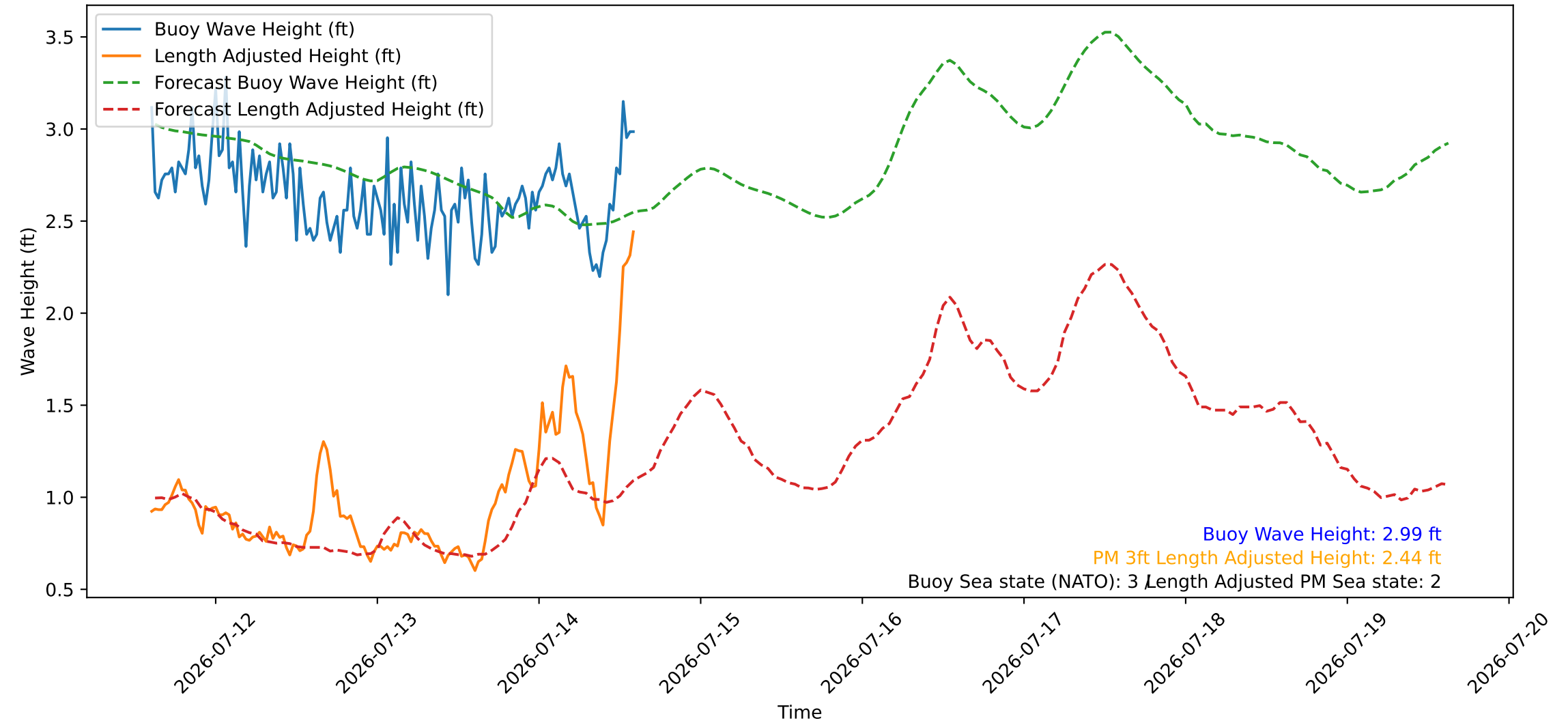
Wave Heights over Time for Oceanside Harbor at 2026-07-14 14:40:26
