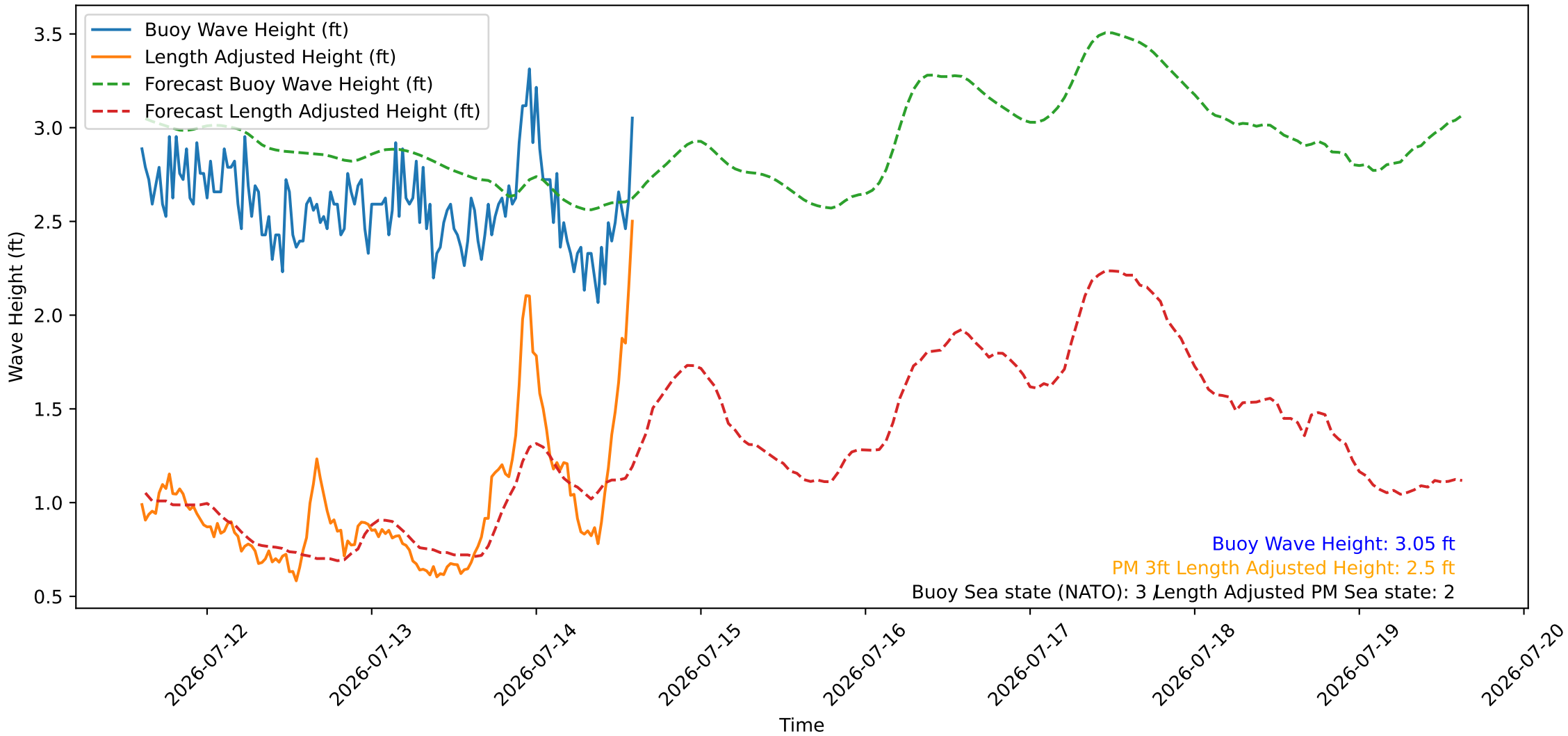
Wave Heights over Time for Green Beach at 2026-07-14 14:41:09
