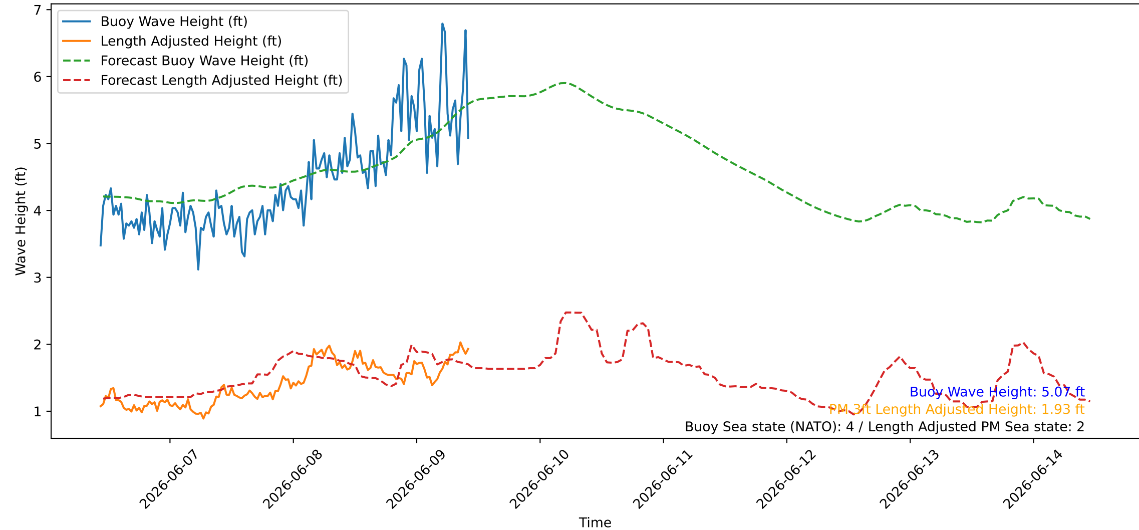
Wave Heights over Time for Green Beach at 2026-06-09 10:41:08
