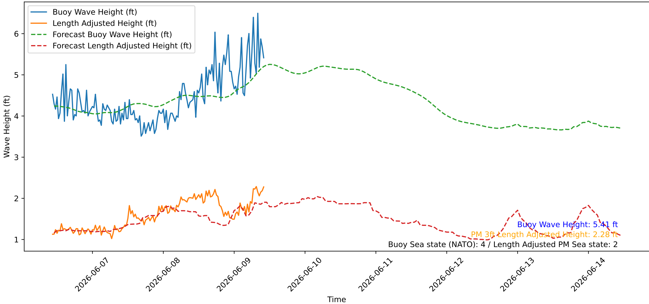
Wave Heights over Time for Oceanside Harbor at 2026-06-09 10:40:26
