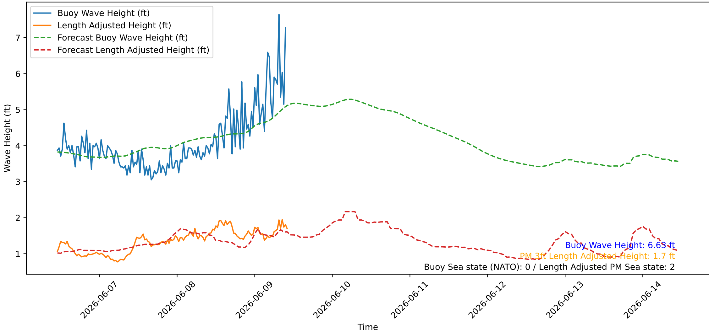
Wave Heights over Time for Red Beach at 2026-06-09 10:40:45
