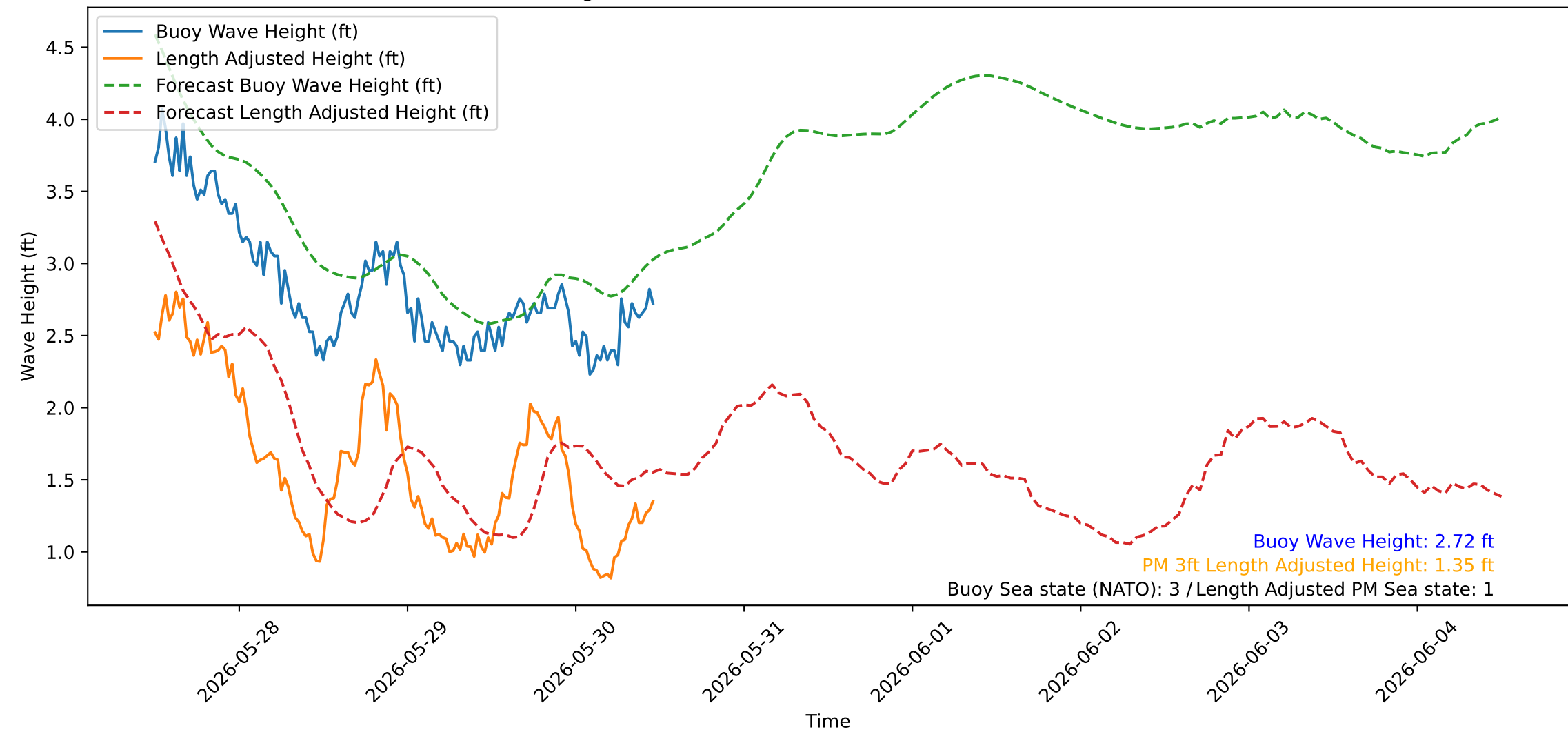
Wave Heights over Time for Red Beach at 2026-05-30 11:50:44
