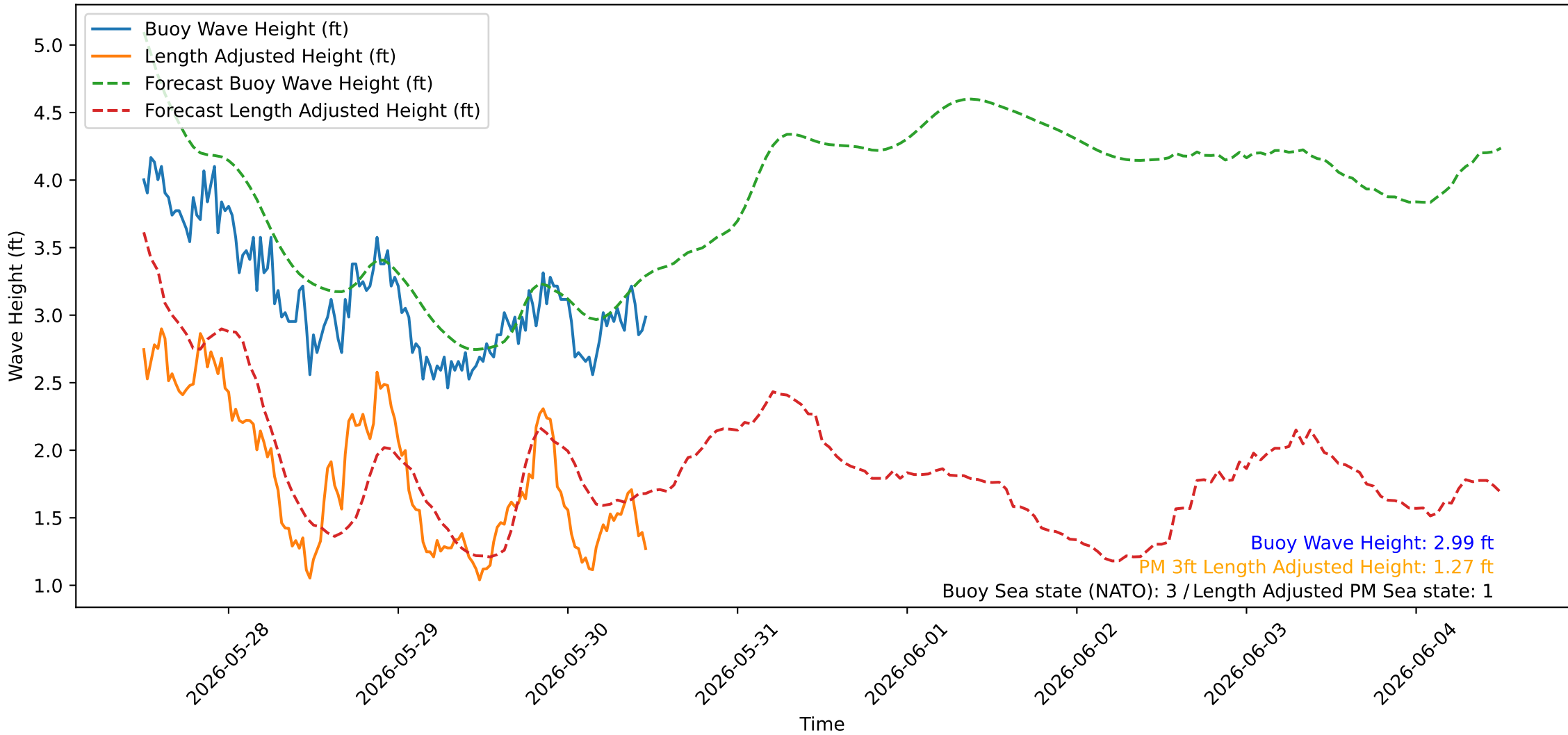
Wave Heights over Time for Green Beach at 2026-05-30 11:51:07
