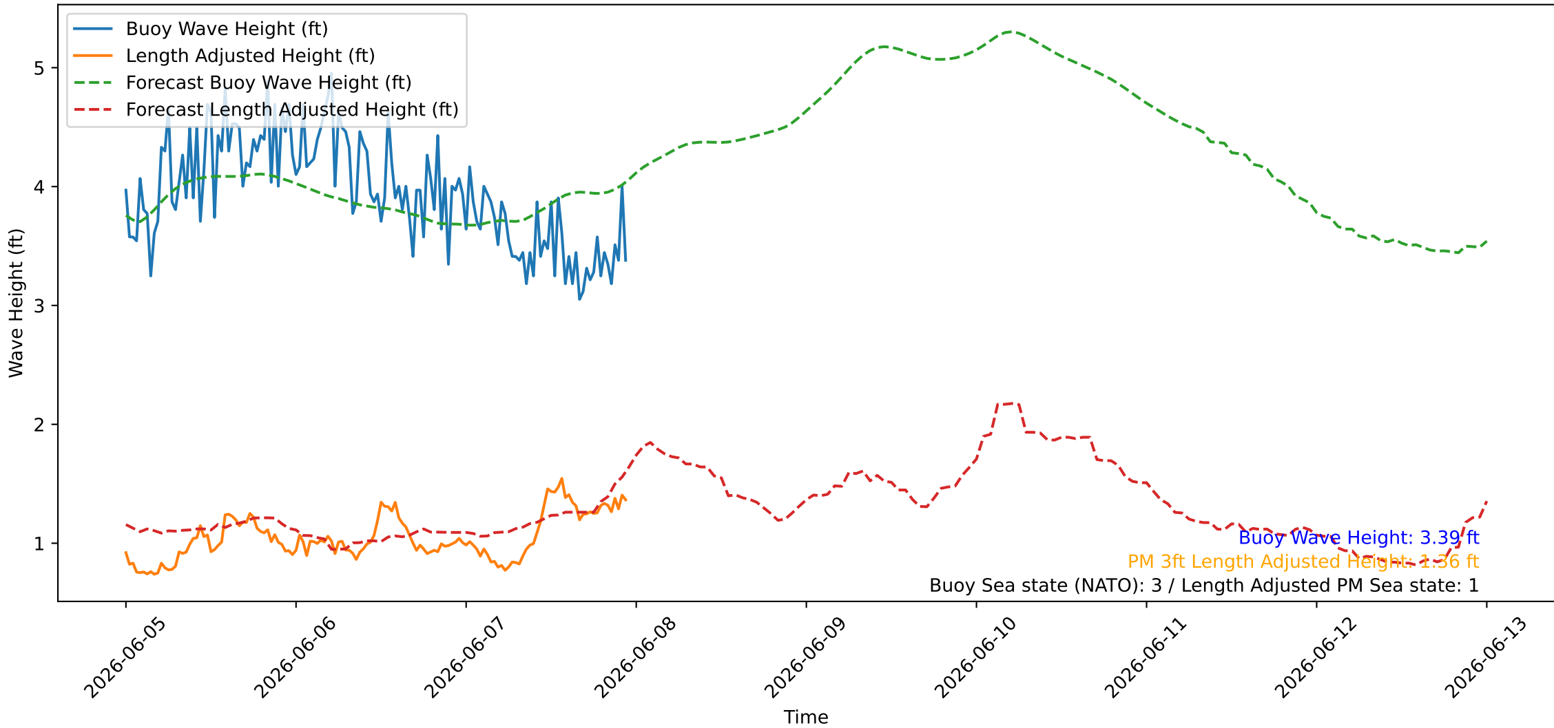
Wave Heights over Time for Red Beach at 2026-06-07 23:30:45
