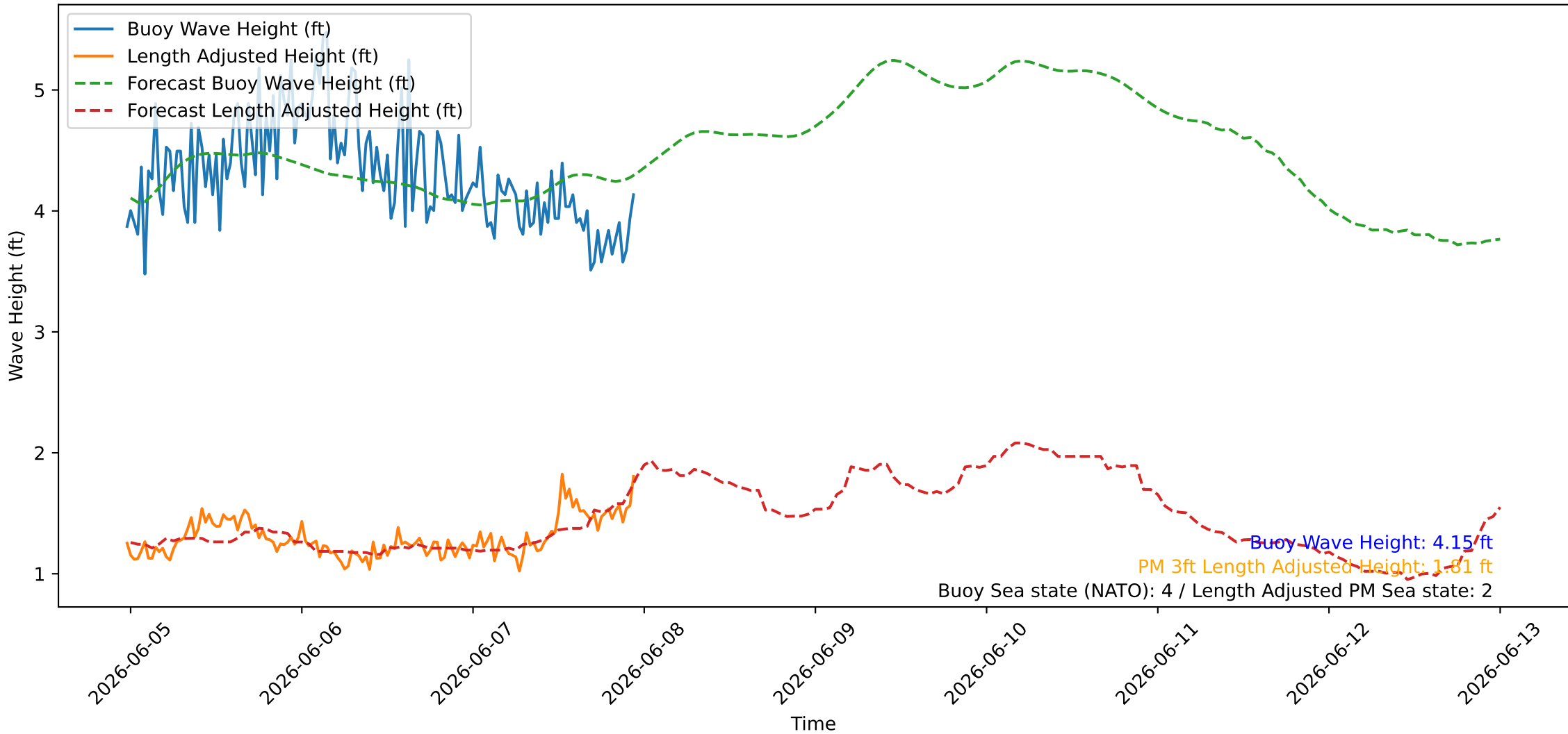
Wave Heights over Time for Oceanside Harbor at 2026-06-07 23:30:26
