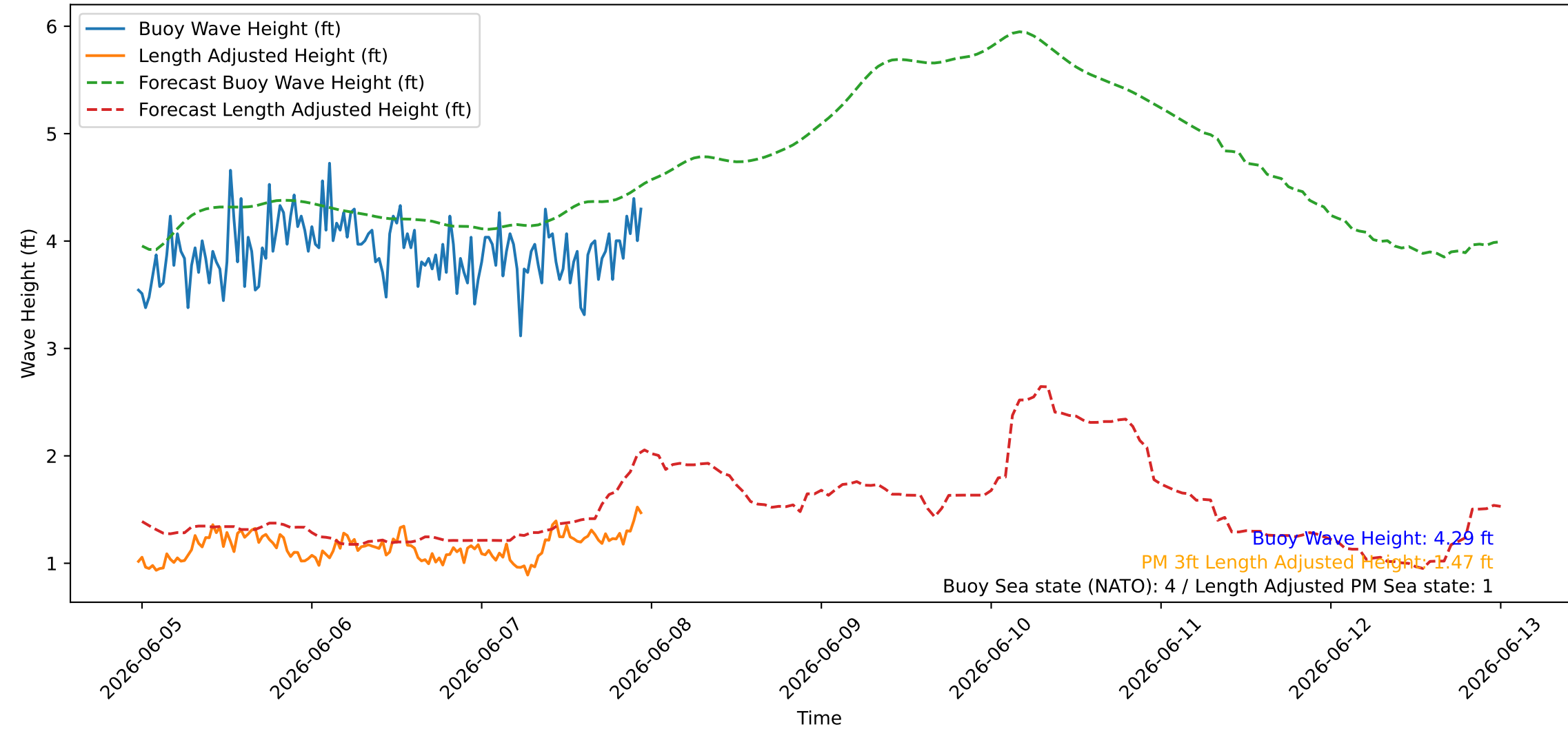
Wave Heights over Time for Green Beach at 2026-06-07 23:31:08
