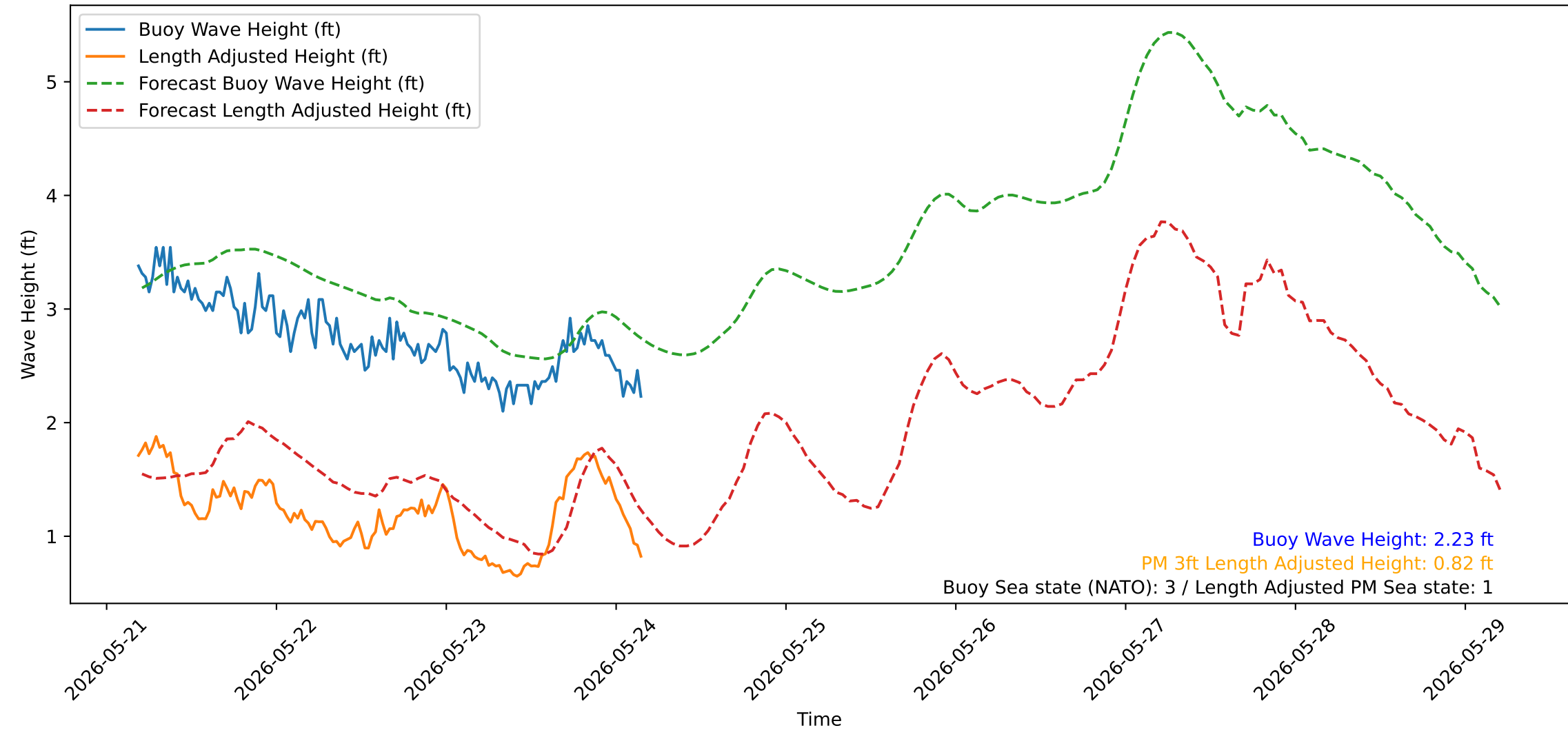
Wave Heights over Time for Green Beach at 2026-05-24 04:31:14
