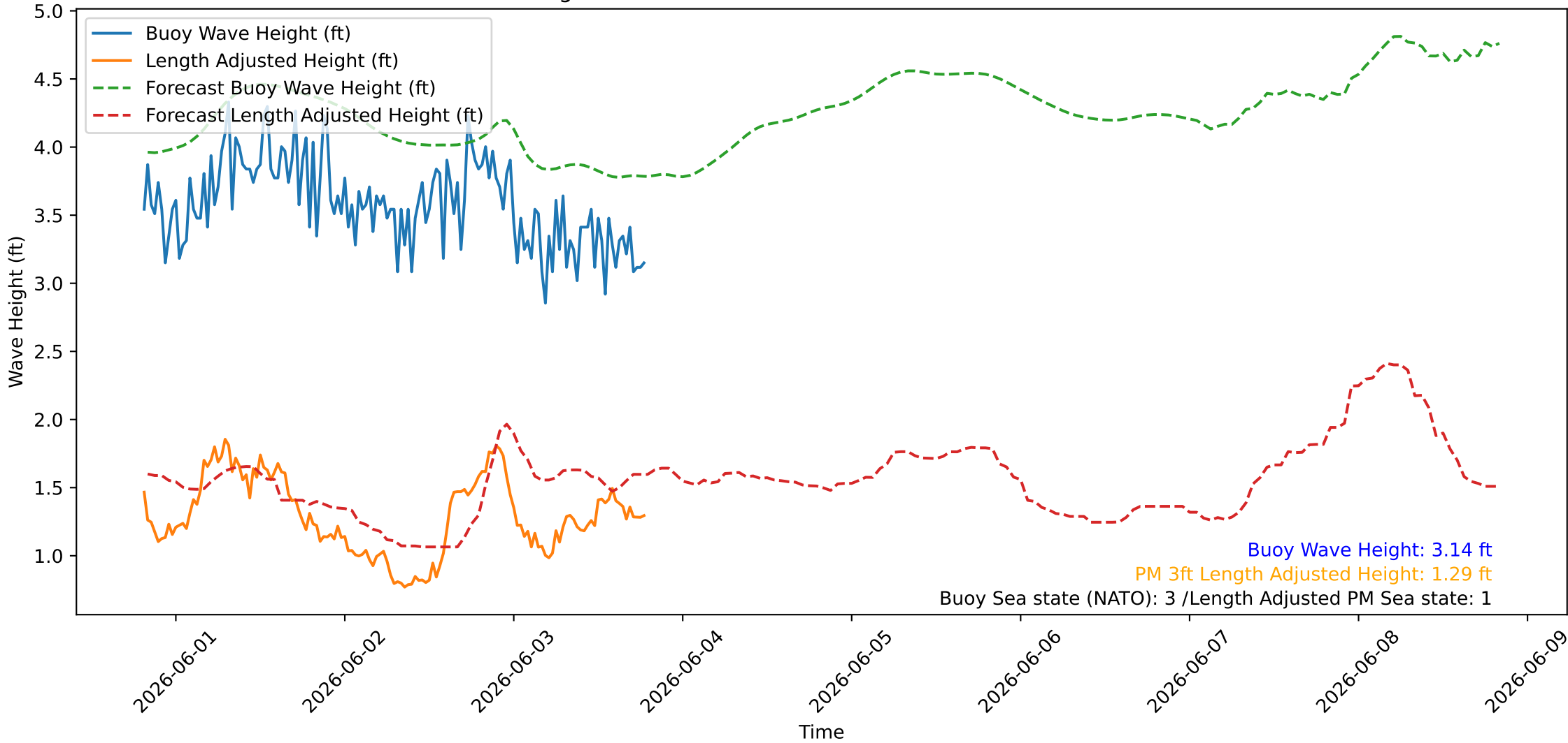
Wave Heights over Time for Green Beach at 2026-06-03 19:31:08
