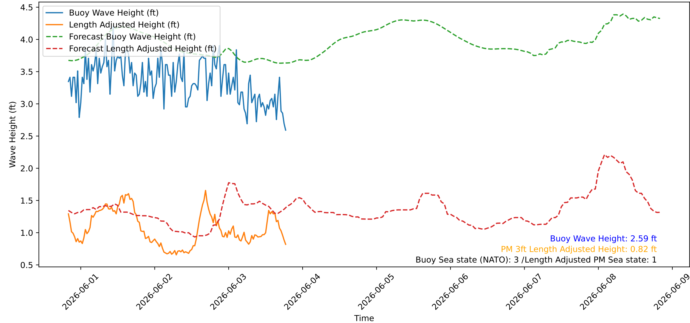
Wave Heights over Time for Red Beach at 2026-06-03 19:30:45
