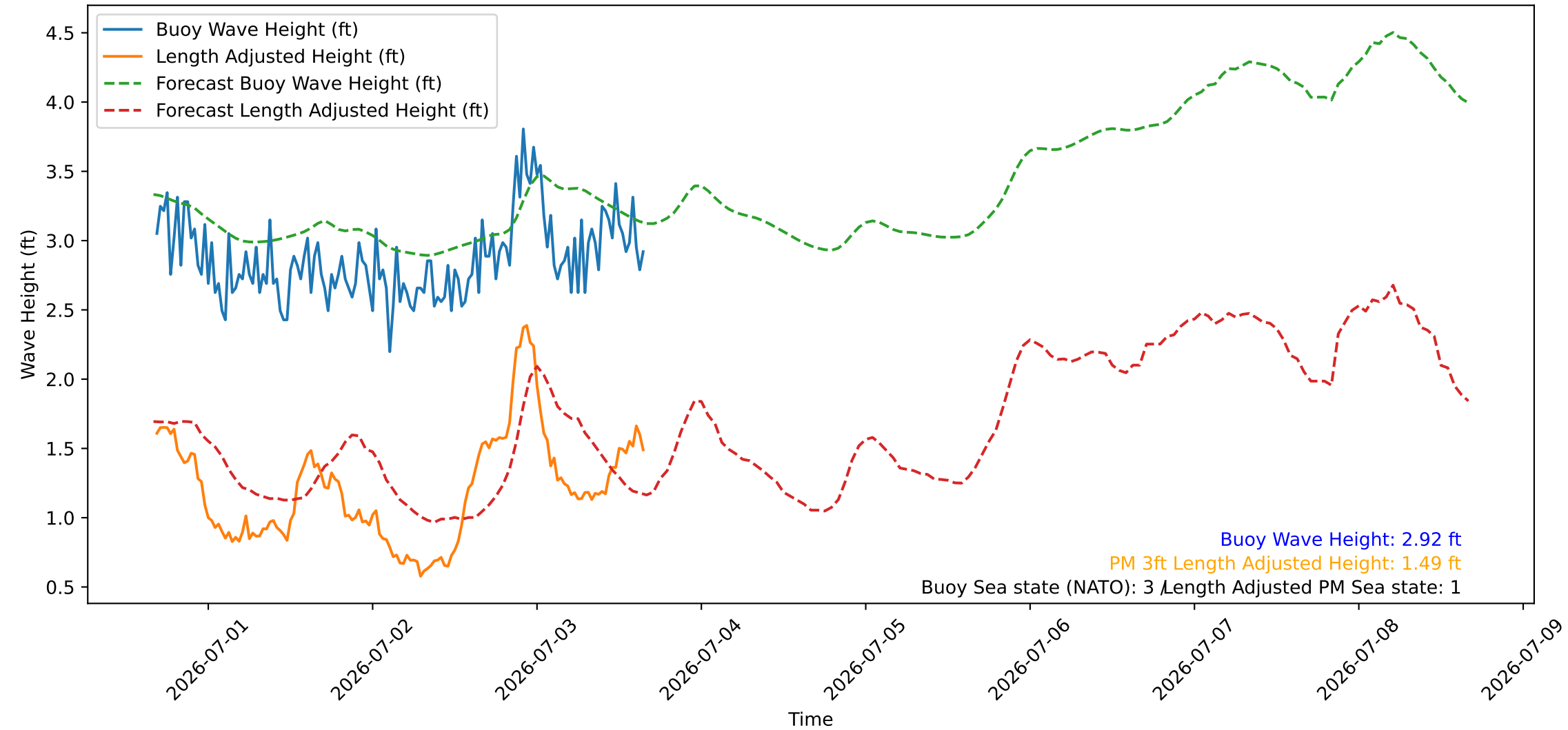
Wave Heights over Time for Red Beach at 2026-07-03 16:20:47
