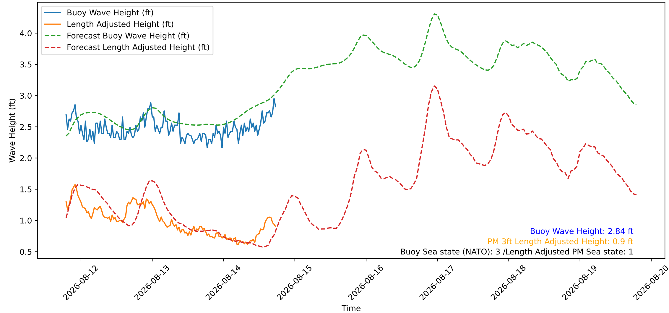
Wave Heights over Time for Red Beach at 2026-08-14 18:50:48
