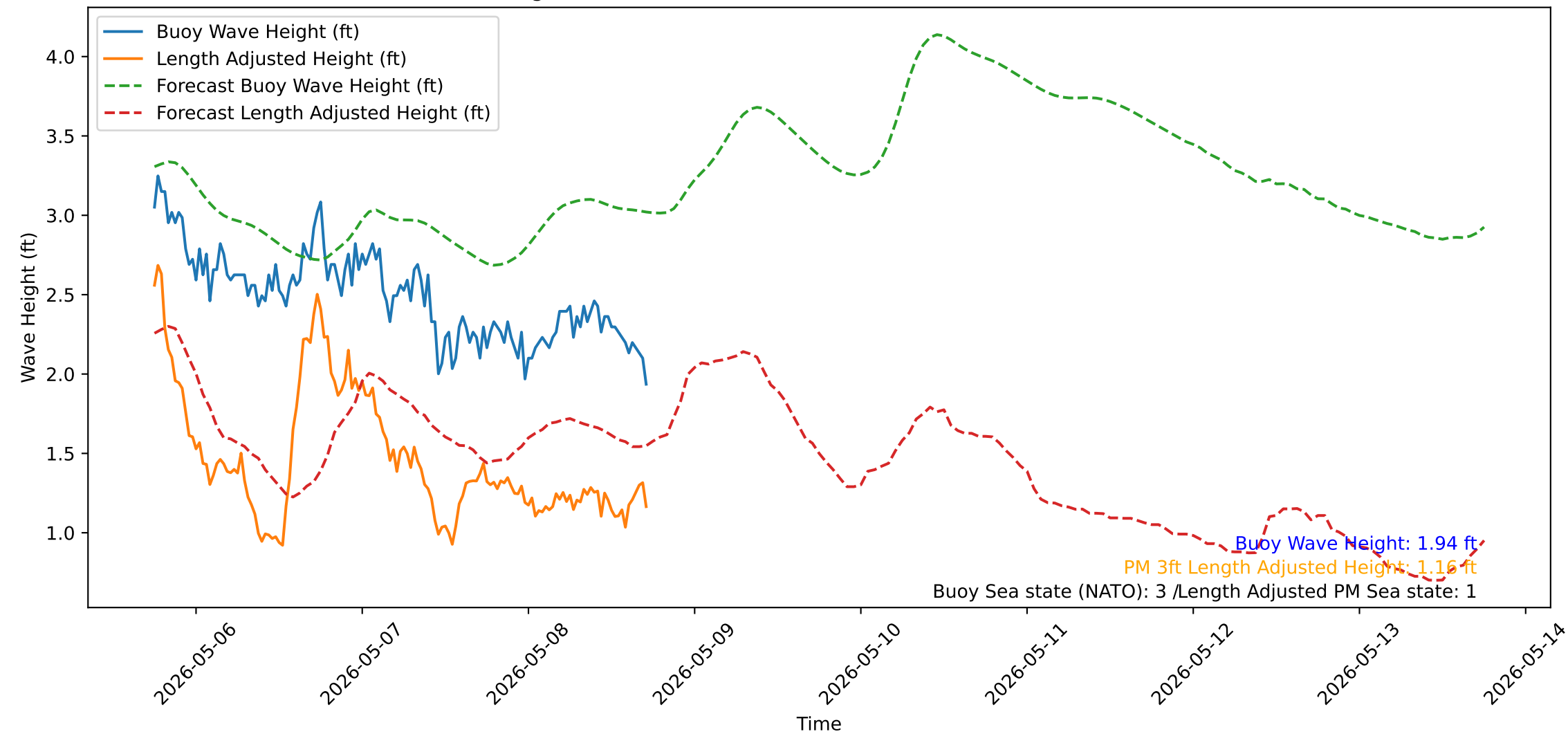
Wave Heights over Time for Oceanside Harbor at 2026-05-08 18:00:31
