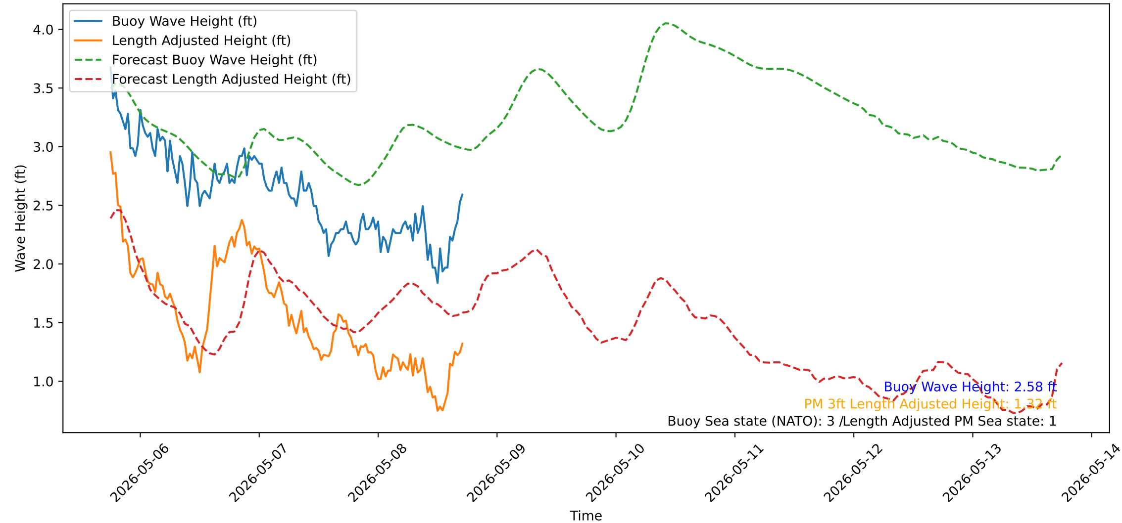
Wave Heights over Time for Green Beach at 2026-05-08 18:01:12
