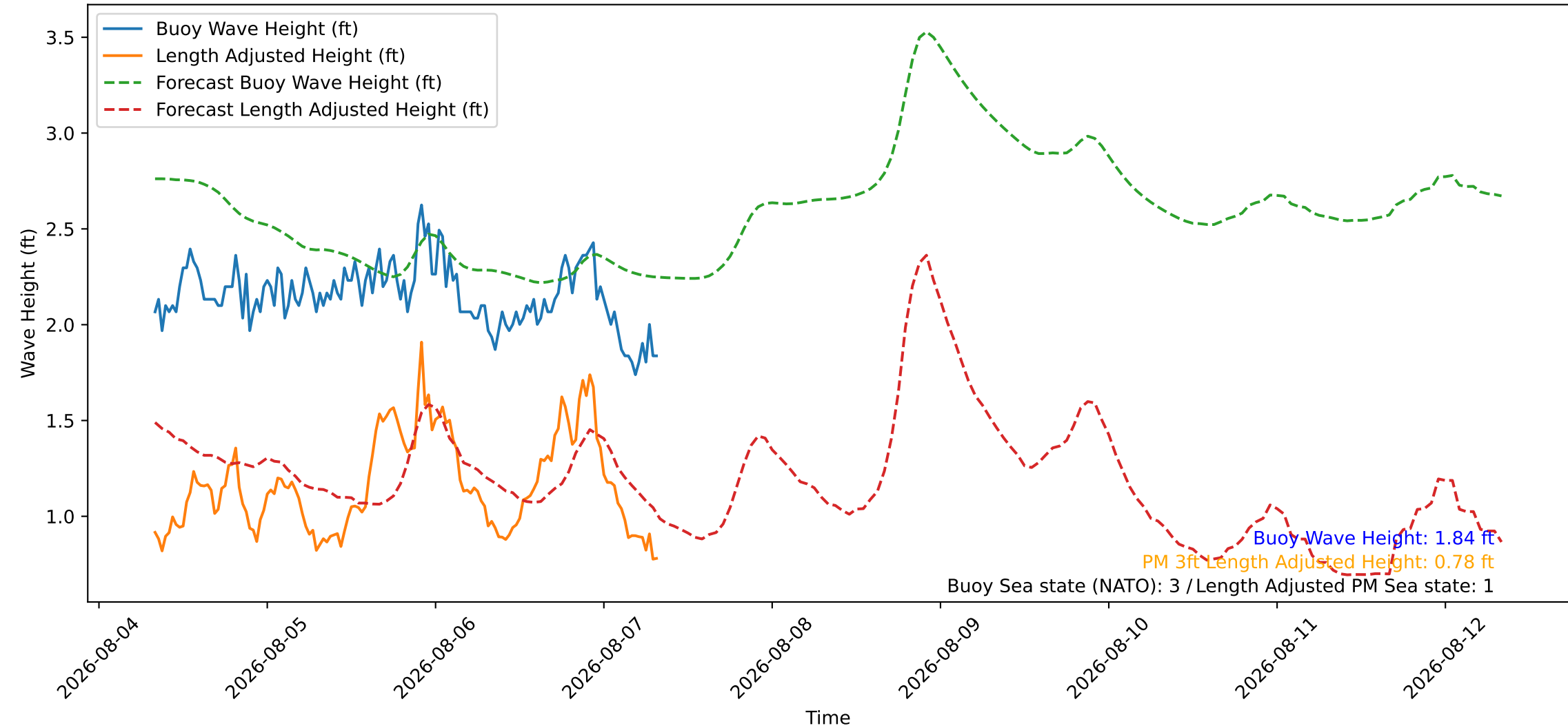
Wave Heights over Time for Green Beach at 2026-08-07 08:11:09
