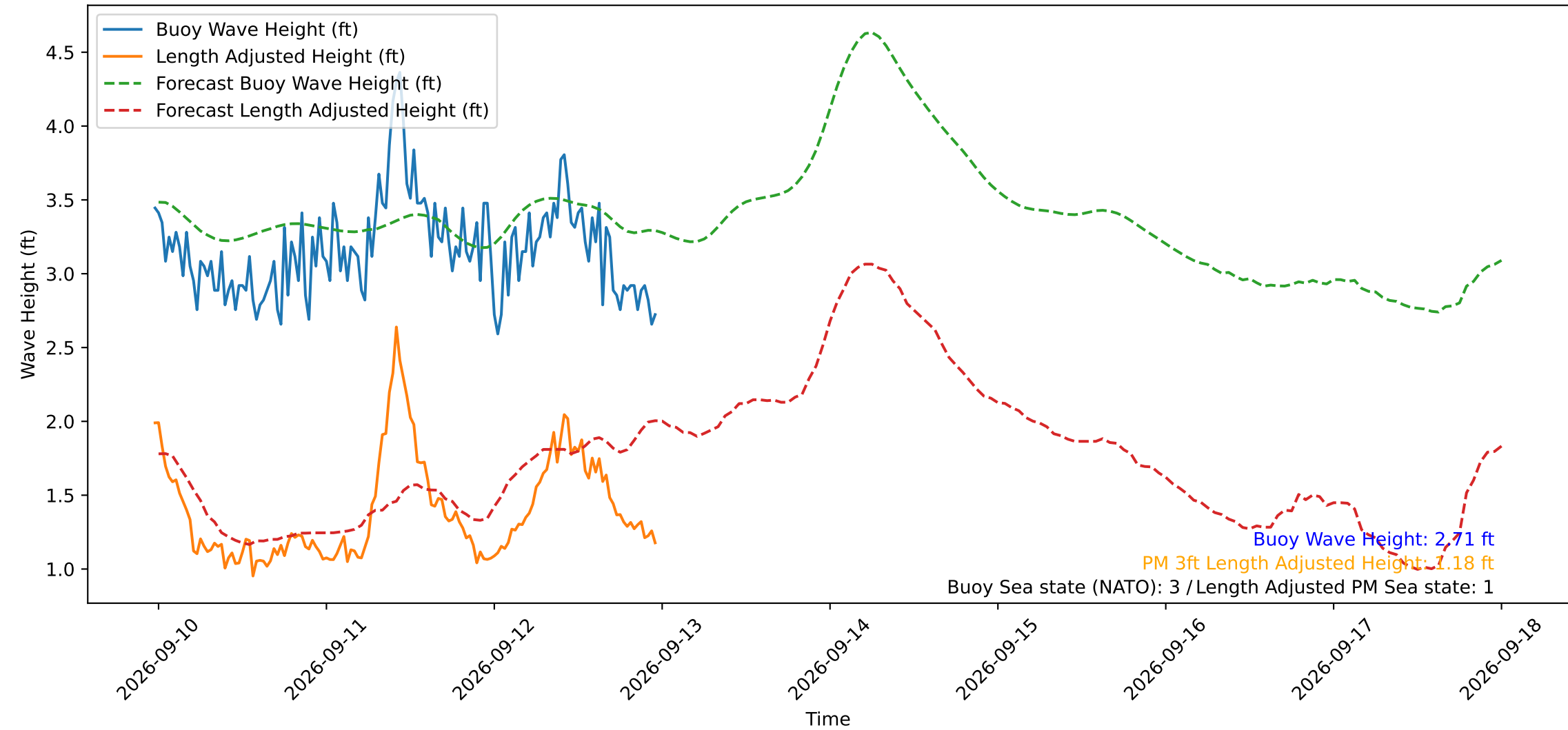
Wave Heights over Time for Oceanside Harbor at 2026-09-12 23:30:30
