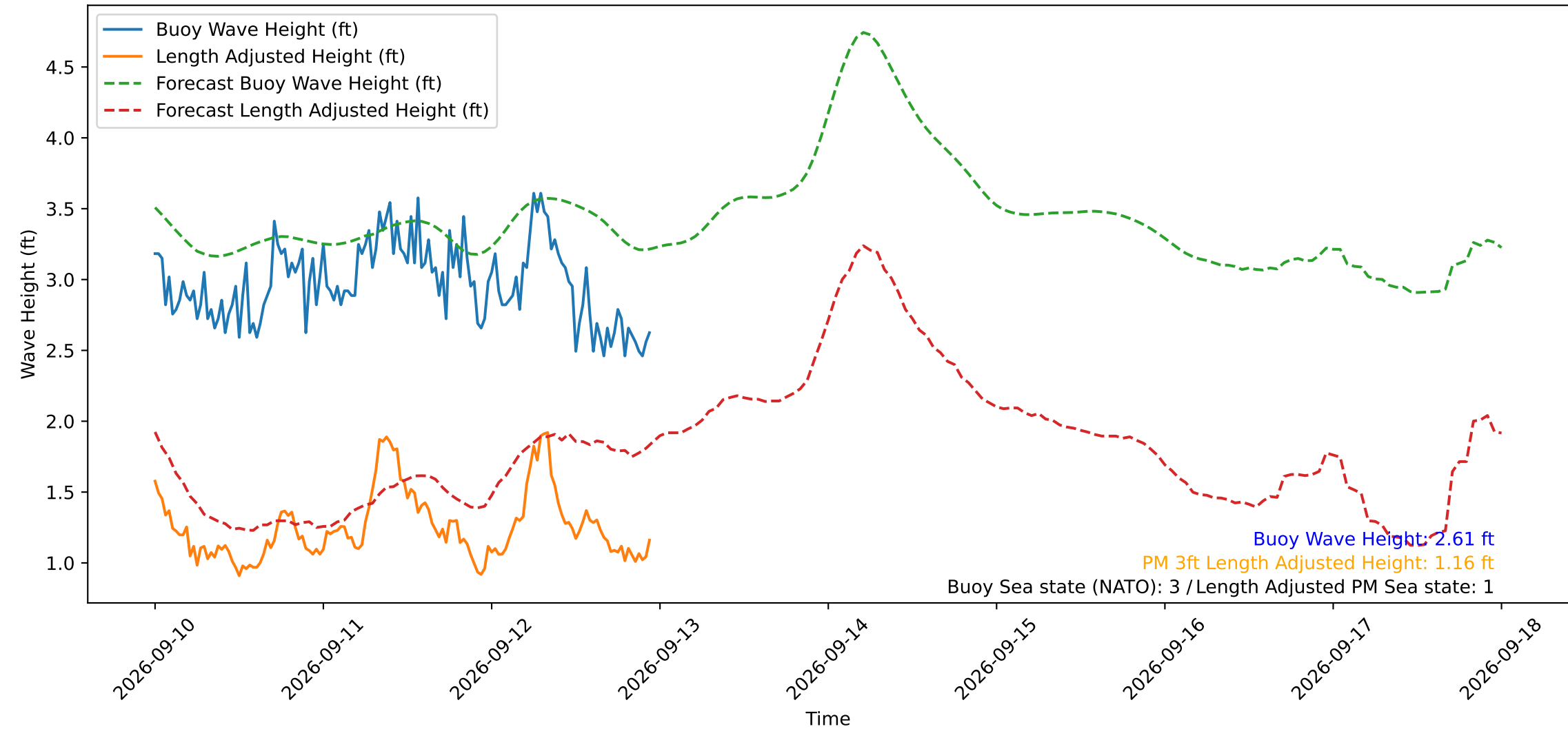
Wave Heights over Time for Green Beach at 2026-09-12 23:31:12
