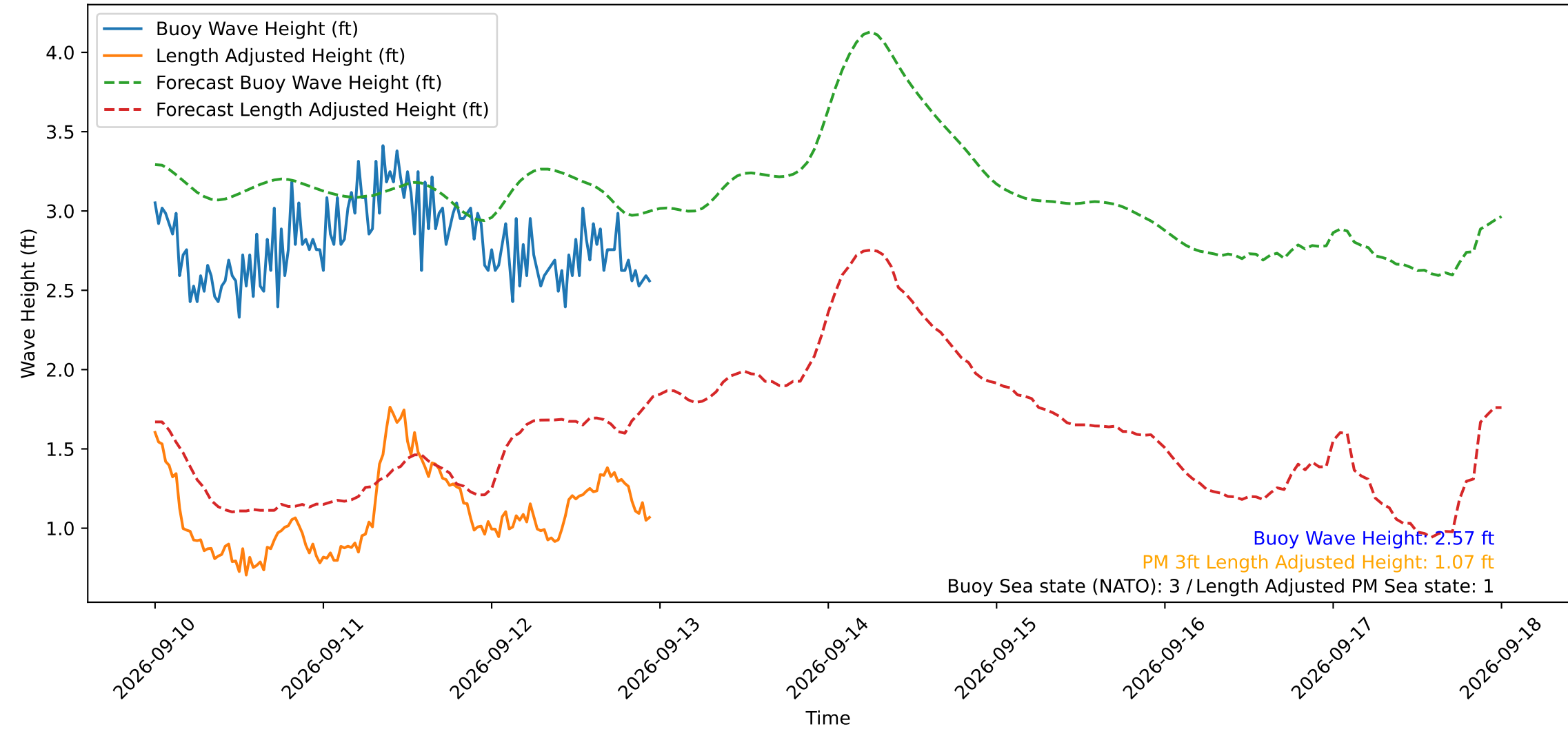
Wave Heights over Time for Red Beach at 2026-09-12 23:30:50
