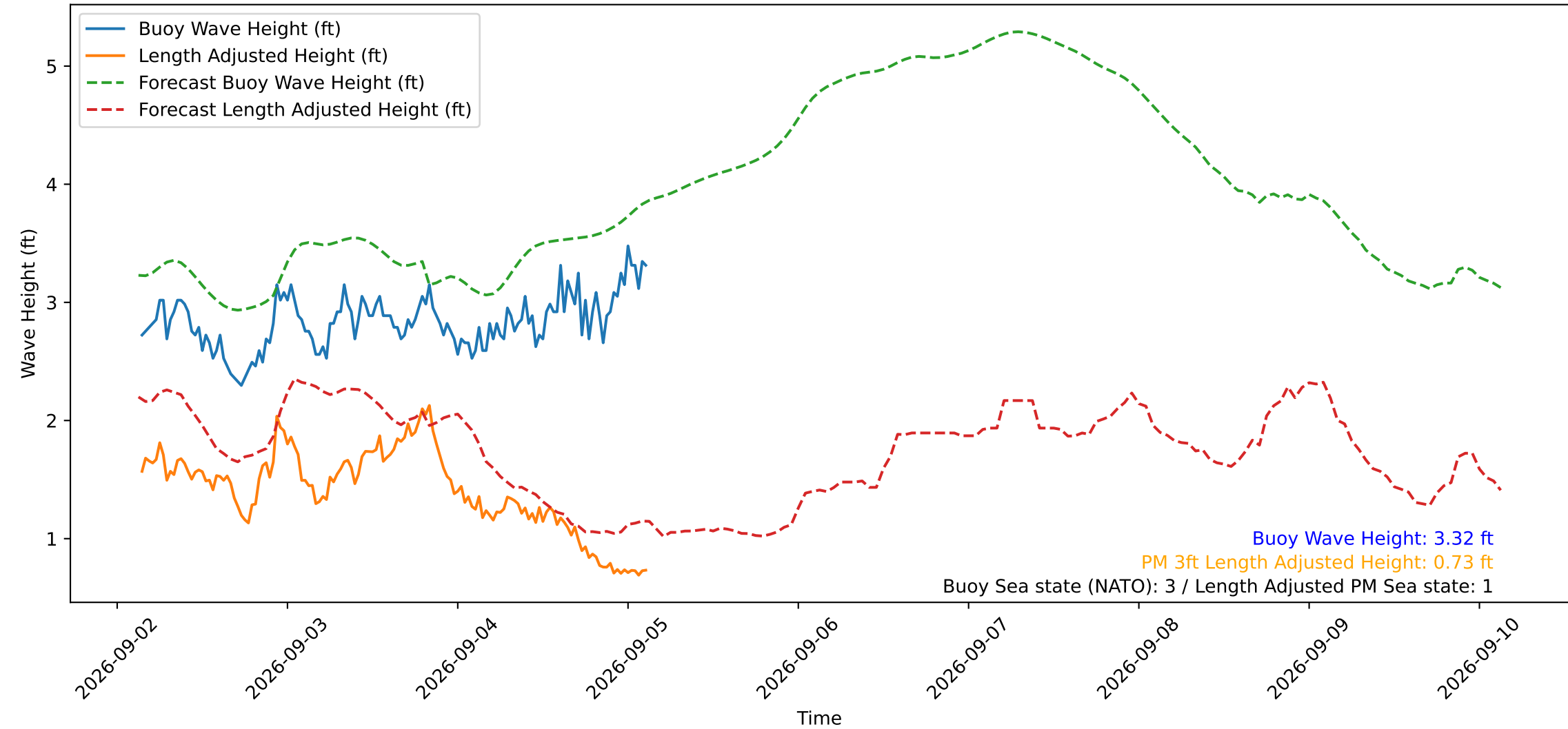
Wave Heights over Time for Red Beach at 2026-09-05 03:20:51
