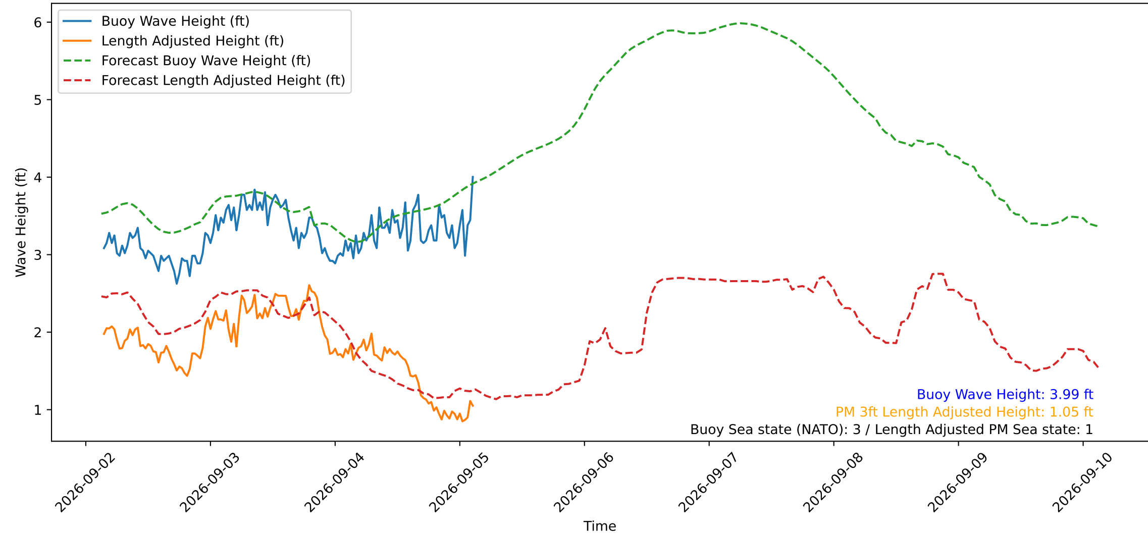
Wave Heights over Time for Oceanside Harbor at 2026-09-05 03:20:29
