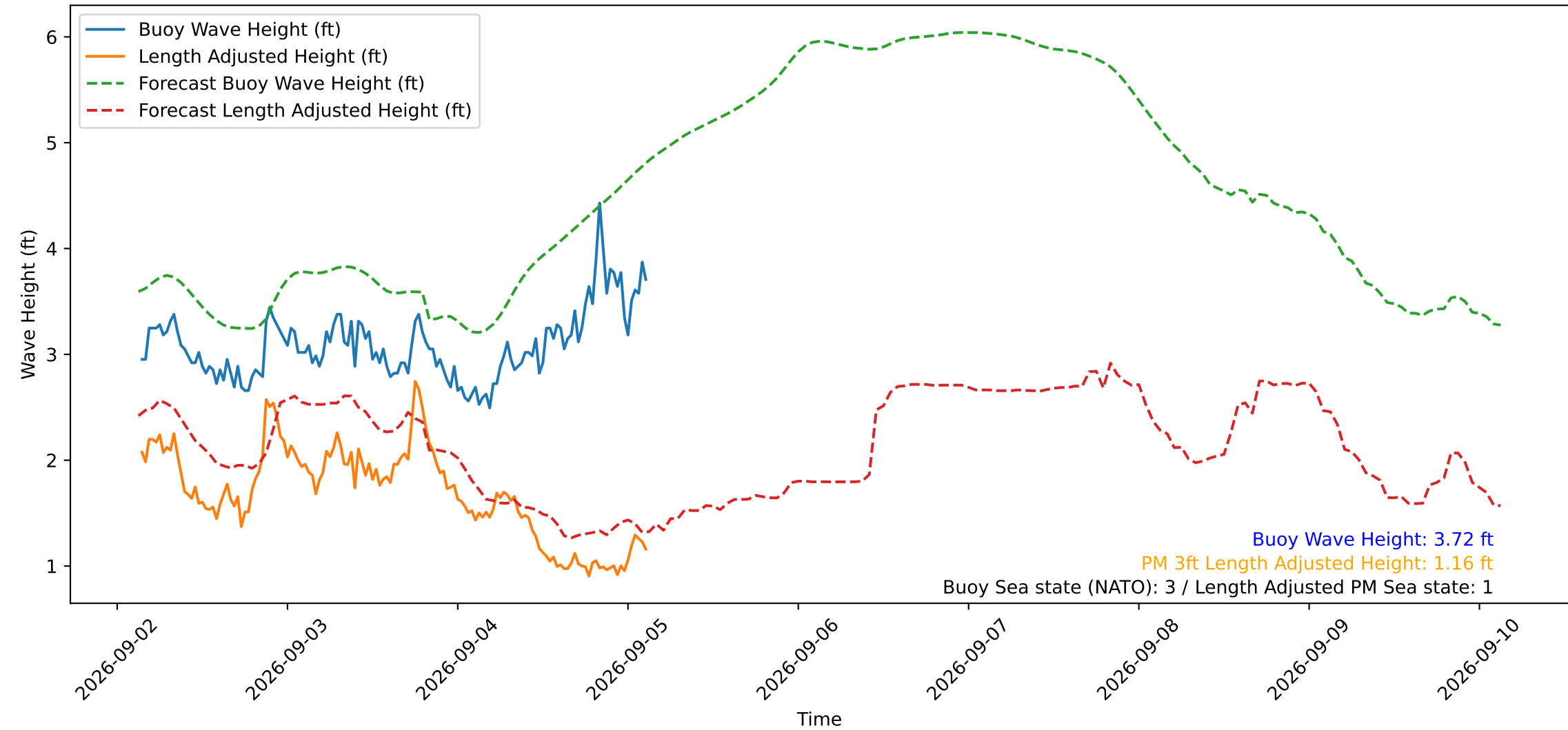
Wave Heights over Time for Green Beach at 2026-09-05 03:21:15
