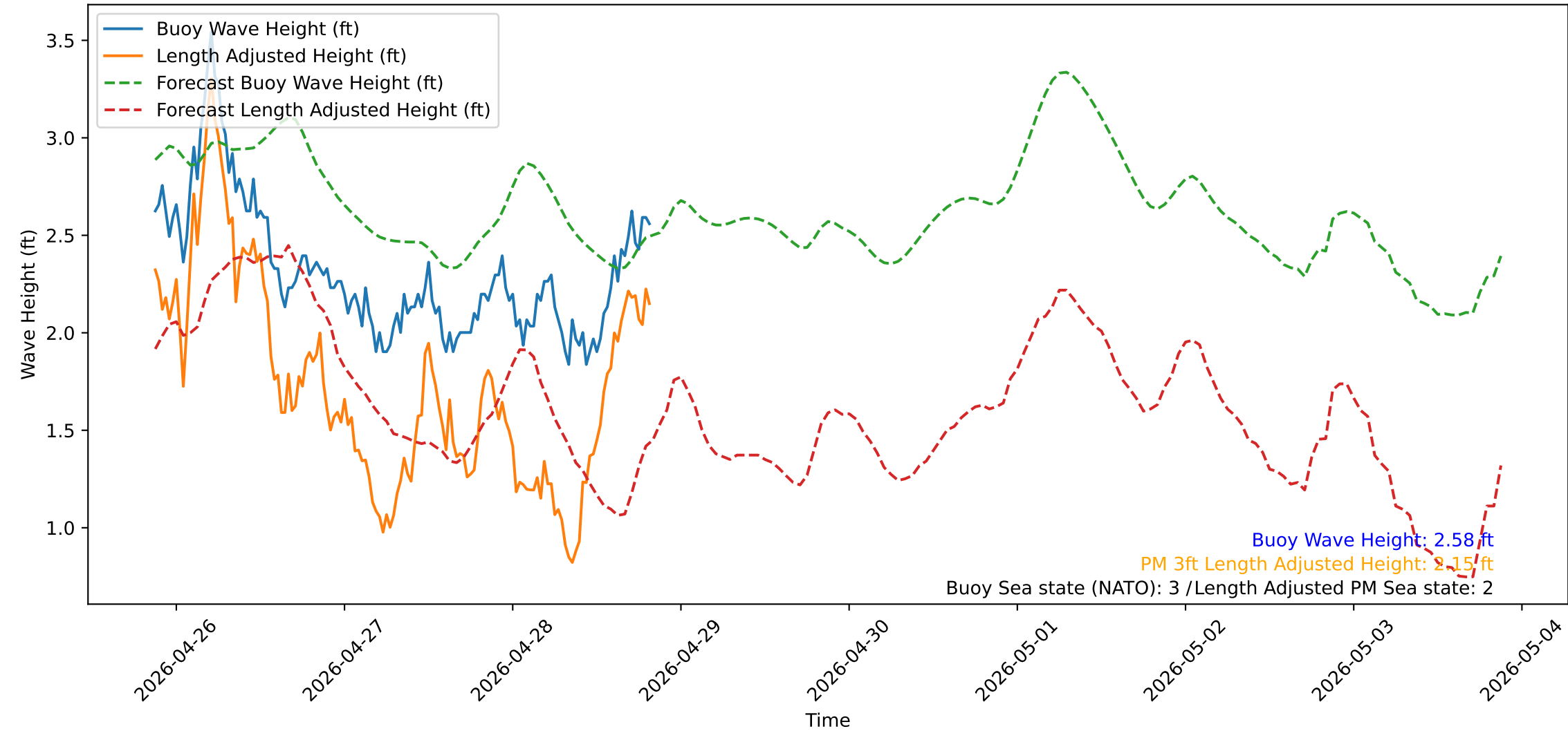
Wave Heights over Time for Red Beach at 2026-04-28 20:30:50
