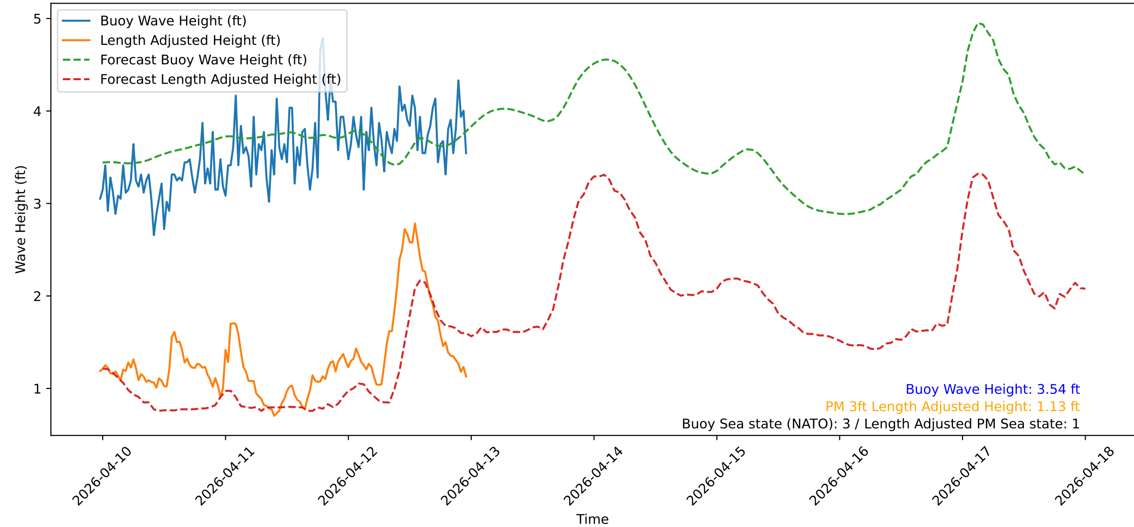
Wave Heights over Time for Oceanside Harbor at 2026-04-12 23:40:31
