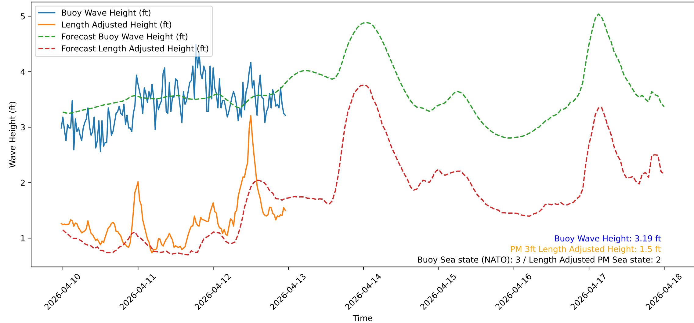
Wave Heights over Time for Green Beach at 2026-04-12 23:41:12
