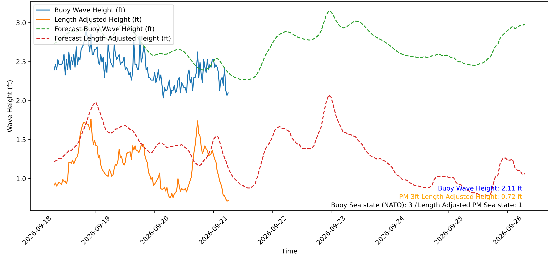
Wave Heights over Time for Red Beach at 2026-09-21 06:50:50
