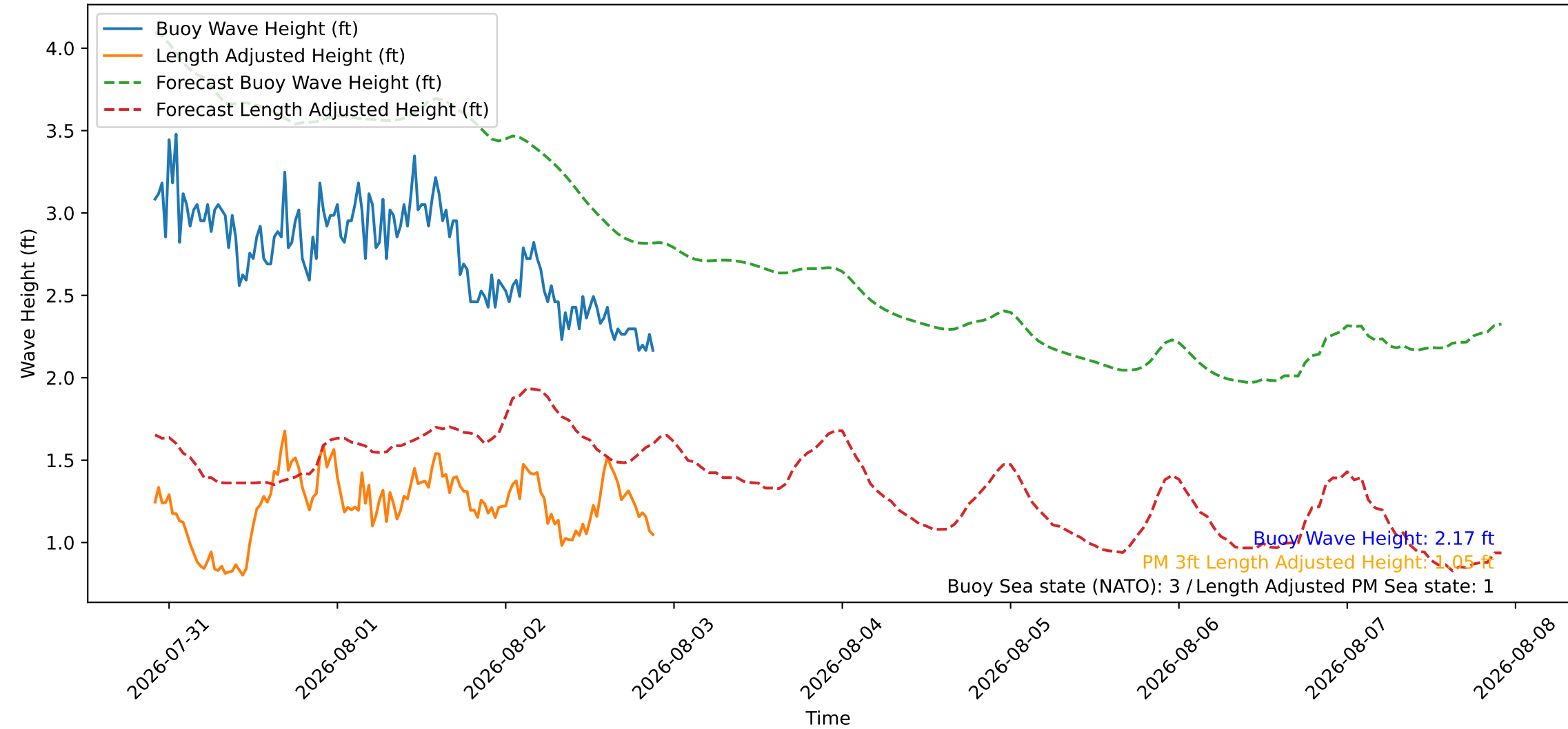
Wave Heights over Time for Red Beach at 2026-08-02 21:40:46
