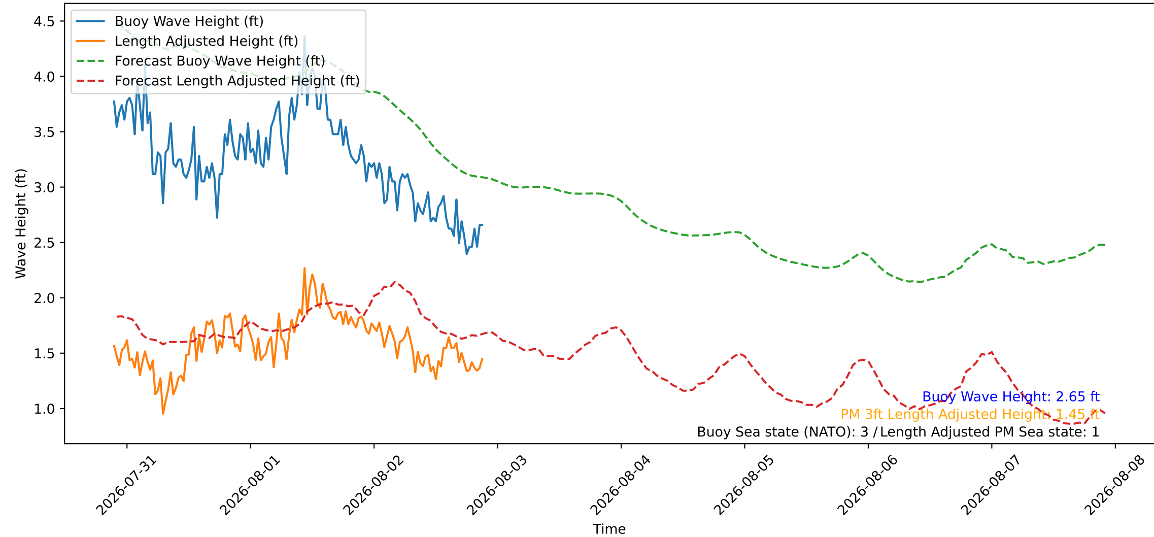
Wave Heights over Time for Oceanside Harbor at 2026-08-02 21:40:26
