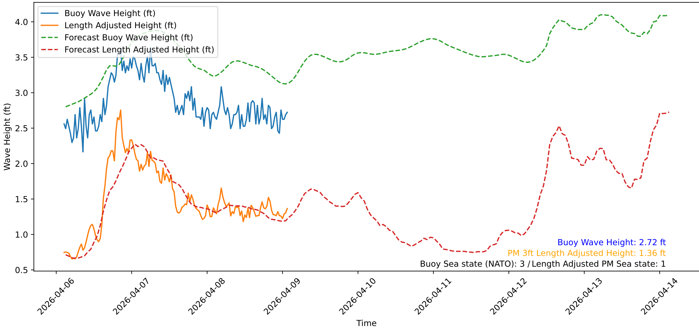
Wave Heights over Time for Oceanside Harbor at 2026-04-09 02:30:32
