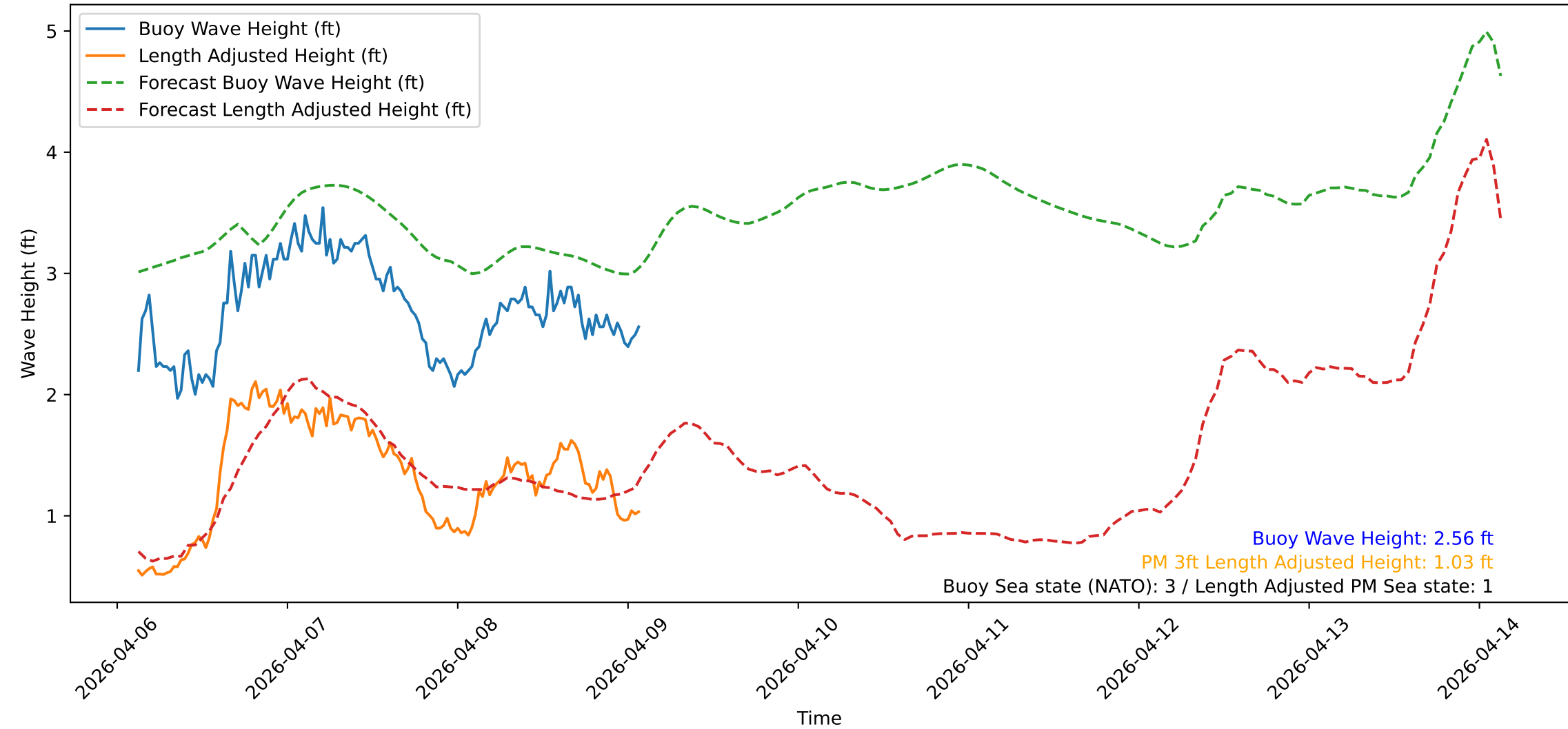
Wave Heights over Time for Red Beach at 2026-04-09 02:30:48
