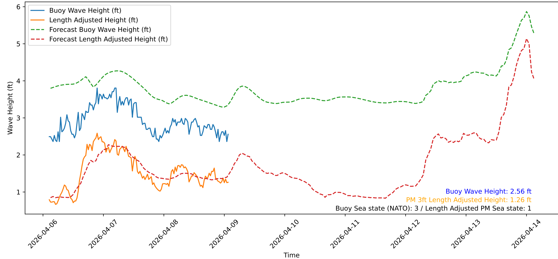
Wave Heights over Time for Green Beach at 2026-04-09 02:31:10
