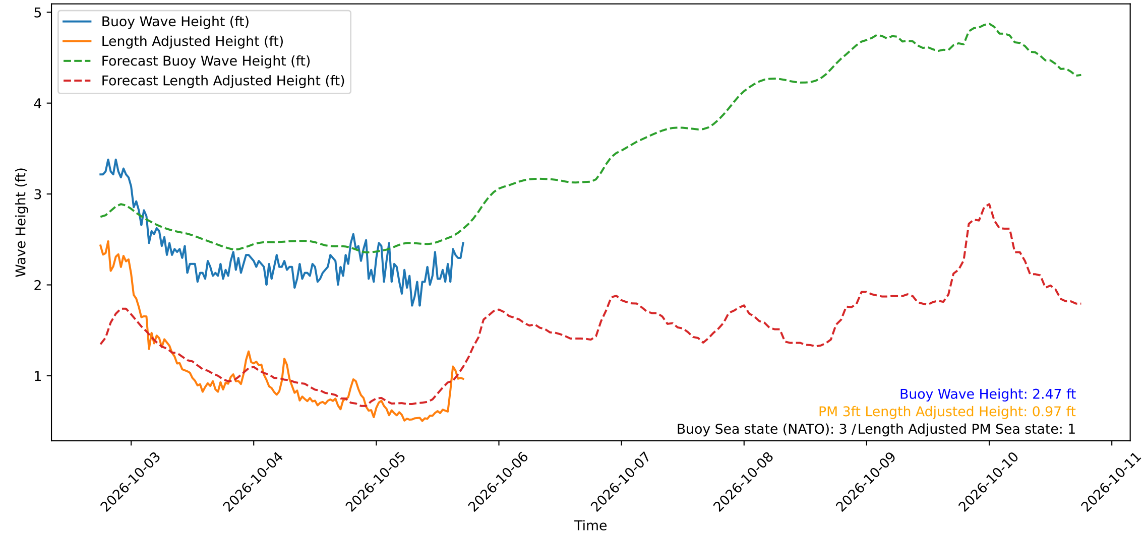
Wave Heights over Time for Green Beach at 2026-10-05 17:41:12
