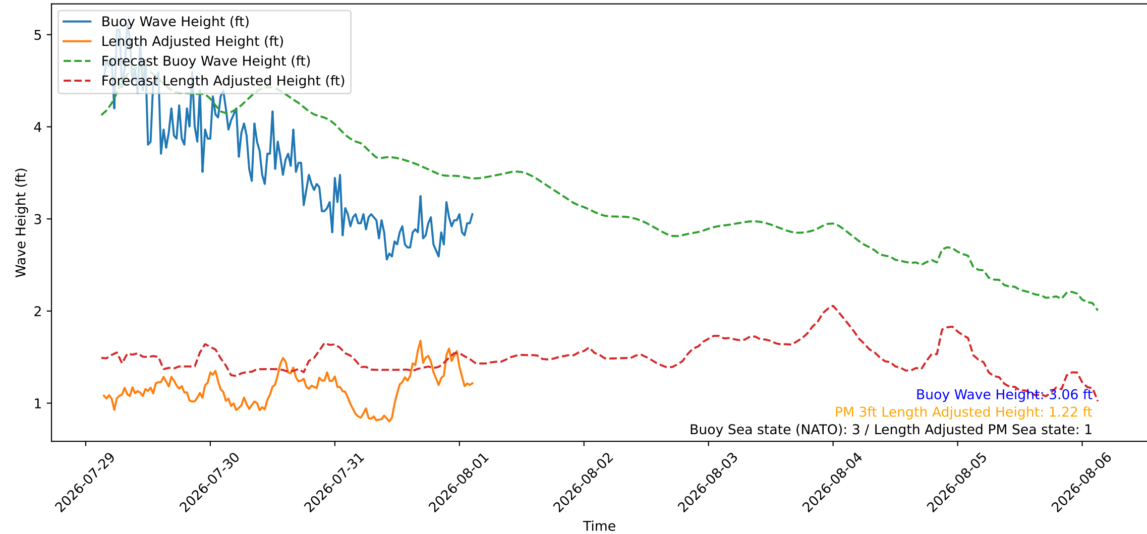
Wave Heights over Time for Red Beach at 2026-08-01 03:10:46
