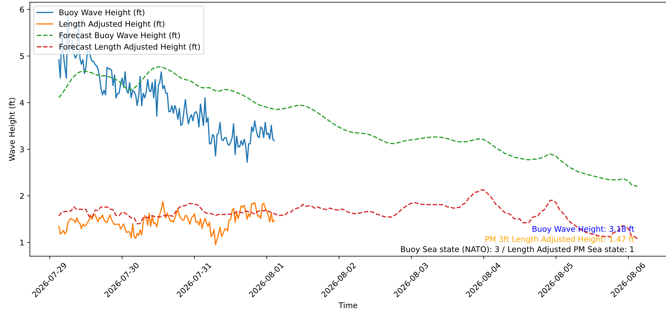
Wave Heights over Time for Oceanside Harbor at 2026-08-01 03:10:26
