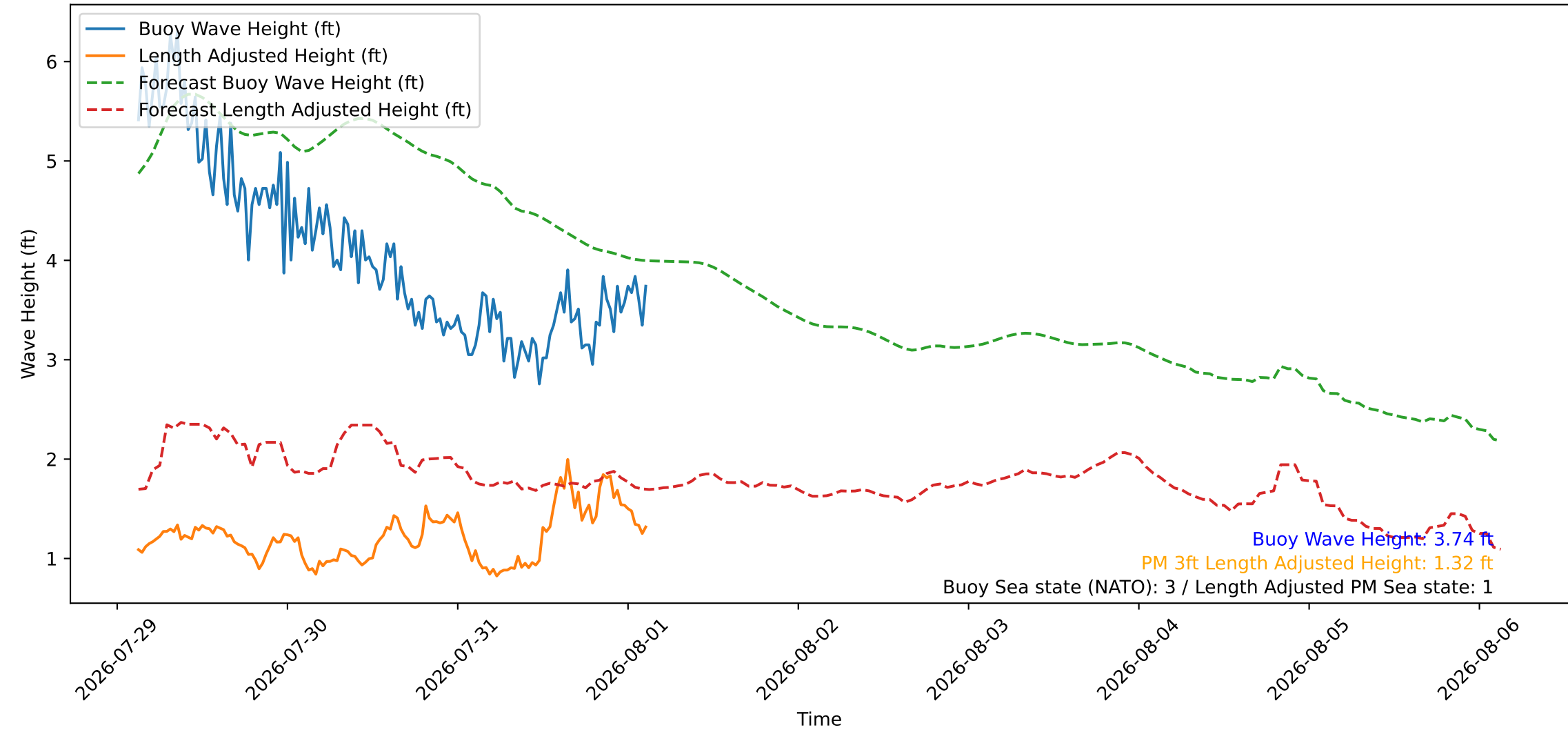
Wave Heights over Time for Green Beach at 2026-08-01 03:11:09
