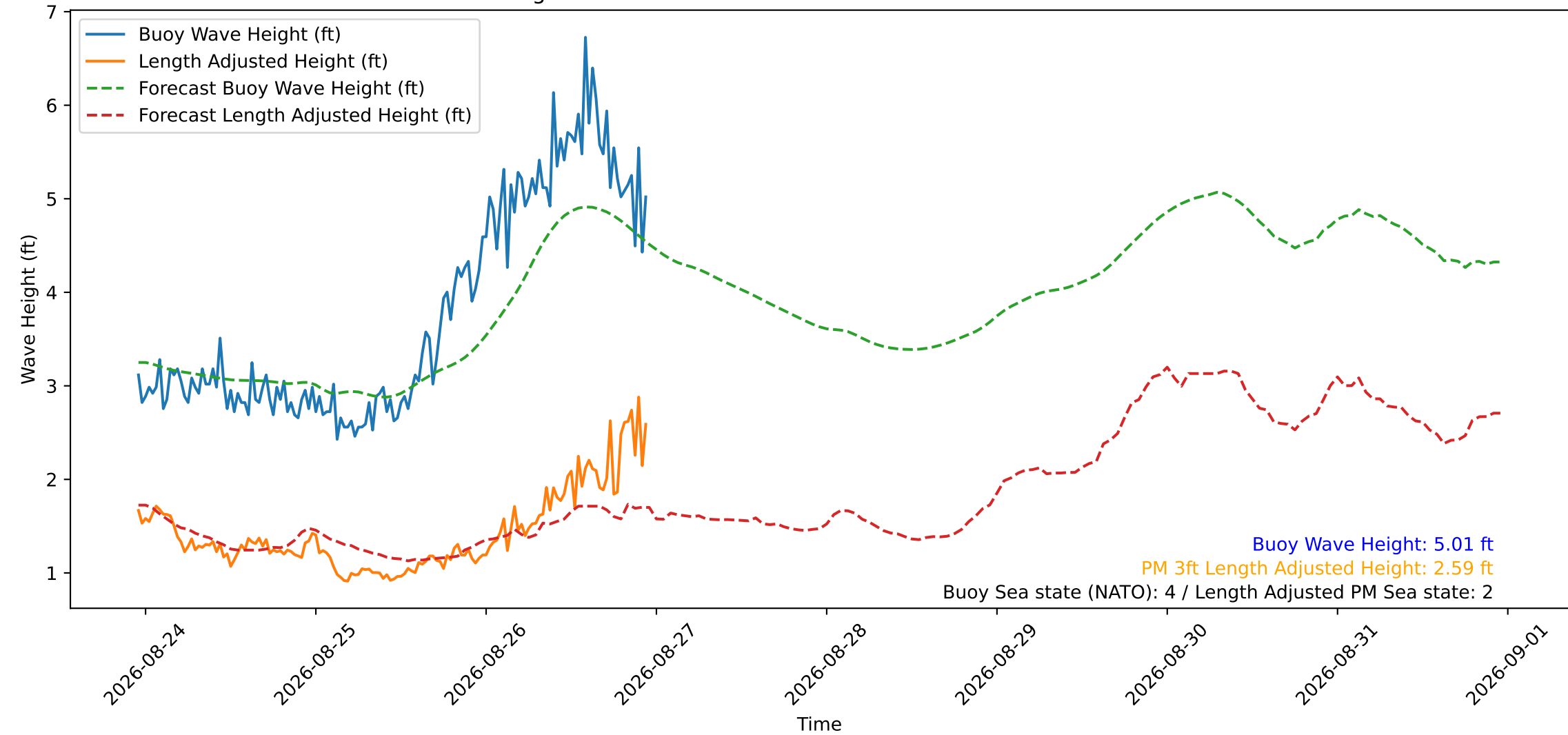
Wave Heights over Time for Oceanside Harbor at 2026-08-26 23:10:30
