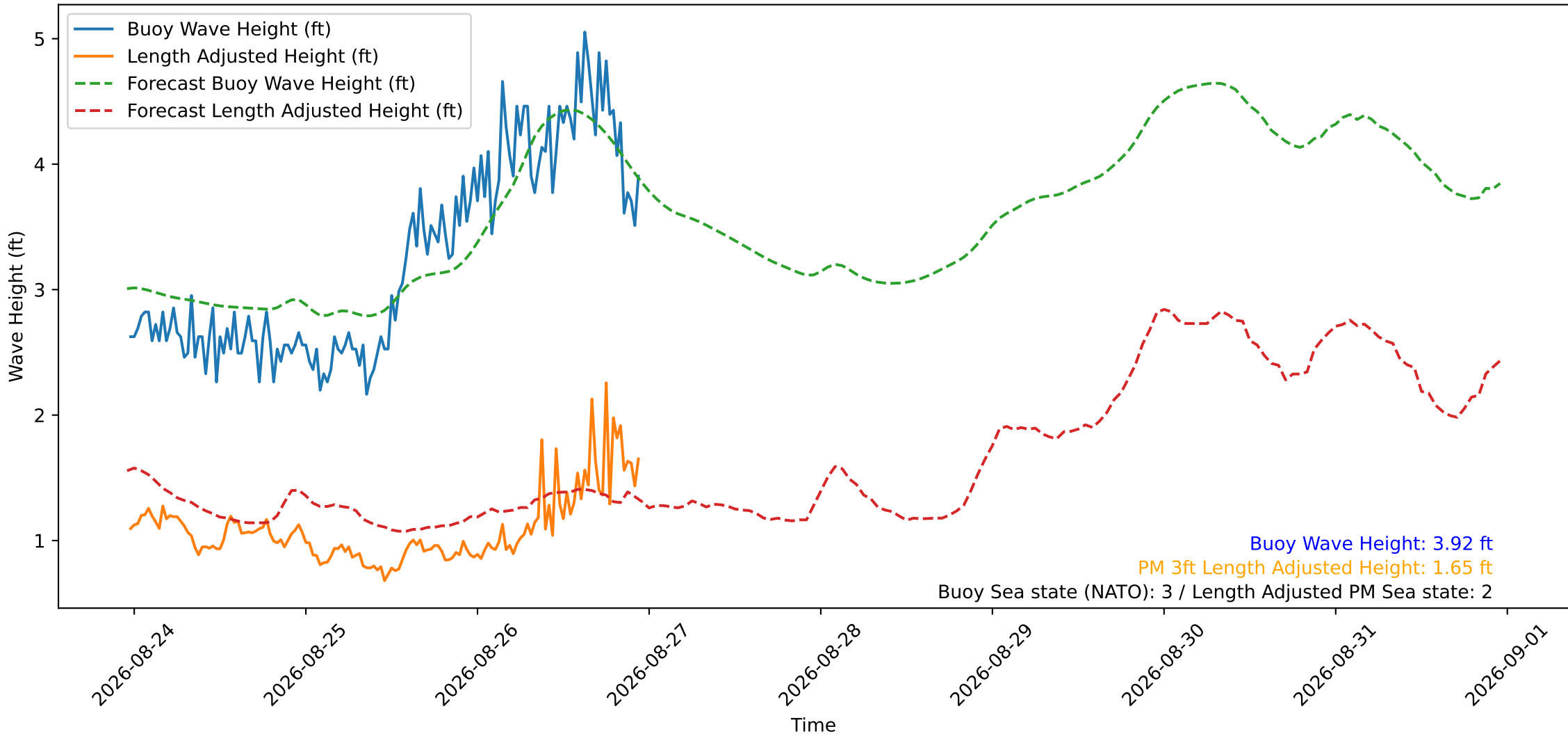
Wave Heights over Time for Red Beach at 2026-08-26 23:10:49
