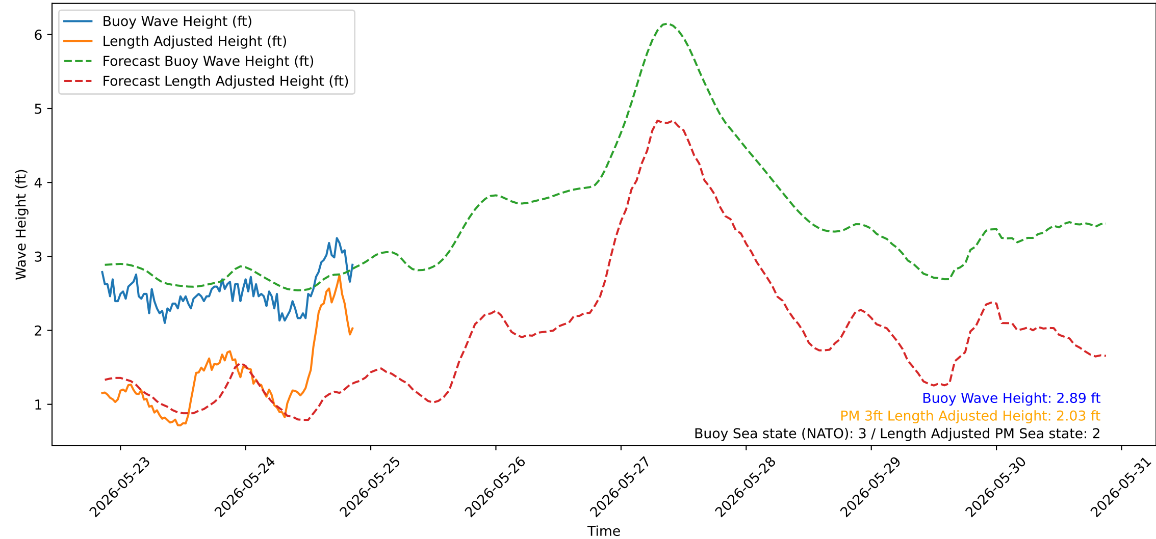
Wave Heights over Time for Oceanside Harbor at 2026-05-25 20:30:30
