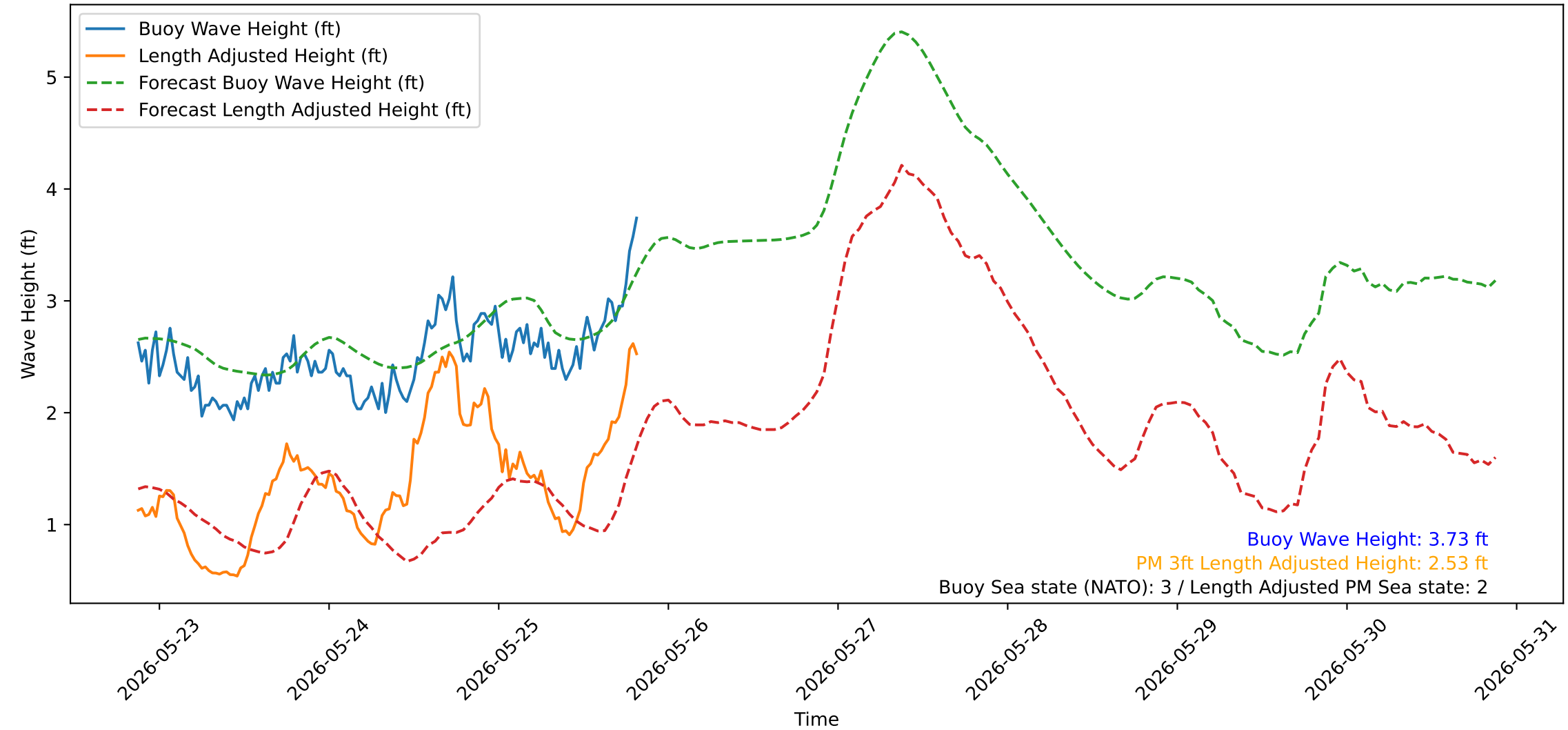
Wave Heights over Time for Red Beach at 2026-05-25 20:30:49
