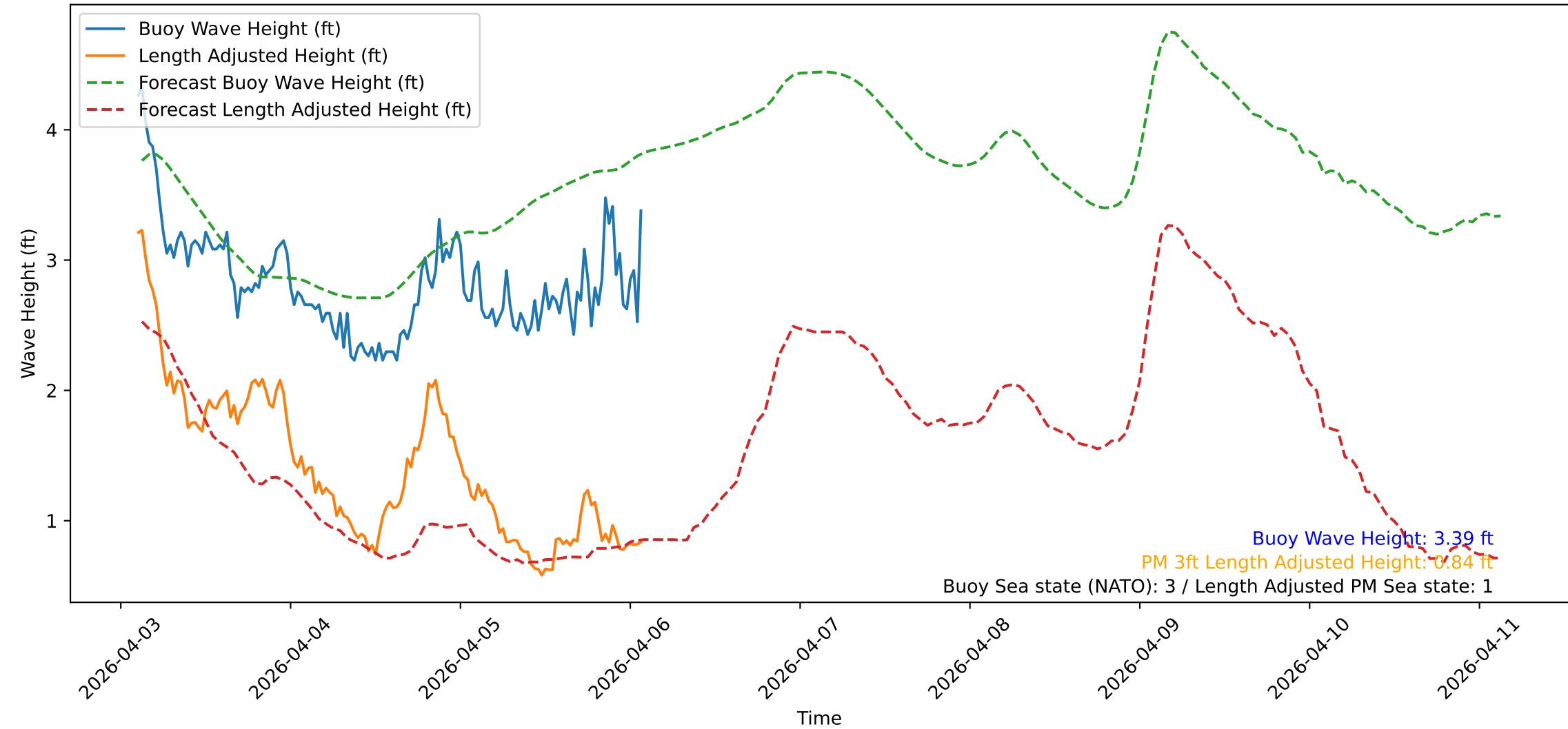
Wave Heights over Time for Green Beach at 2026-04-06 02:31:11
