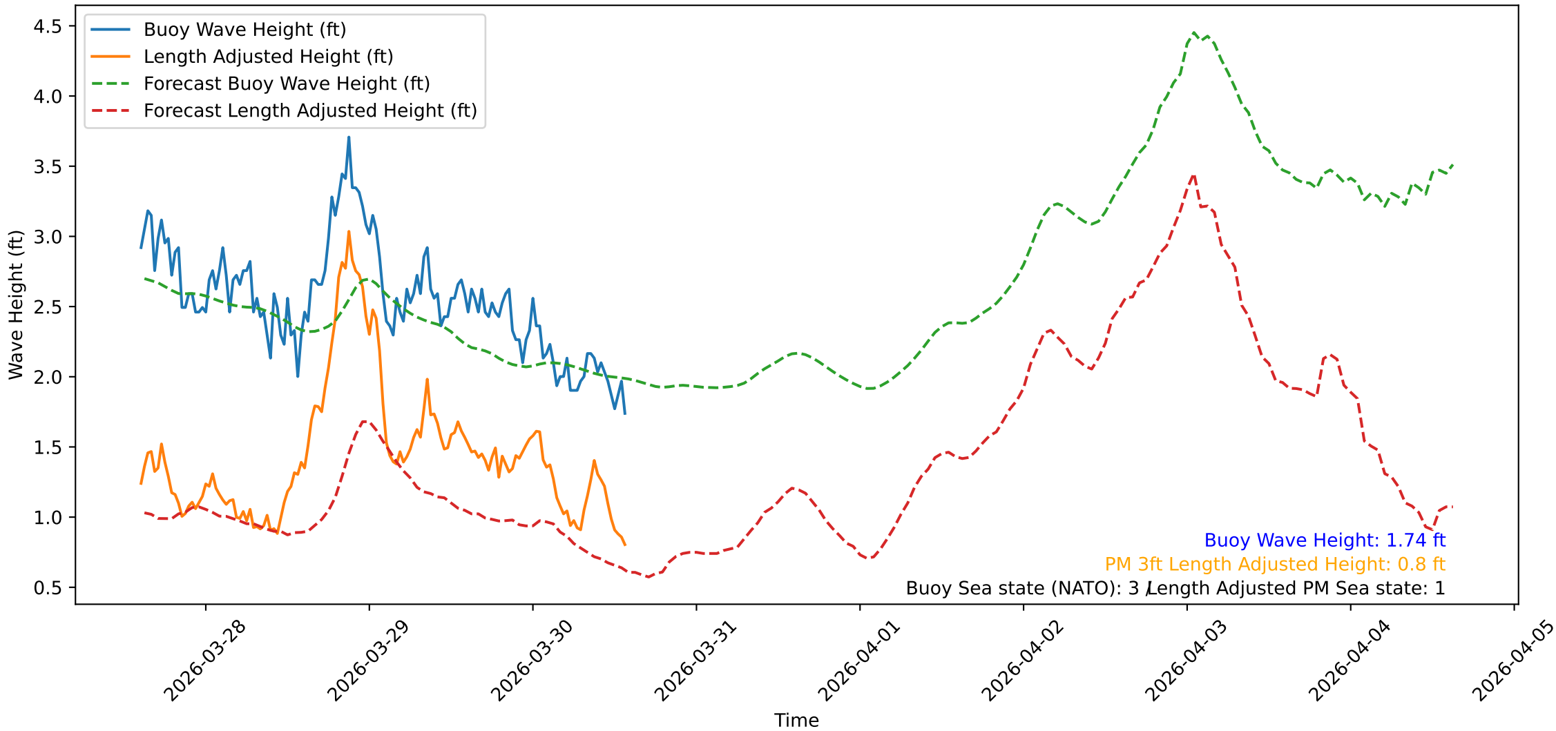
Wave Heights over Time for Green Beach at 2026-03-30 14:31:09
