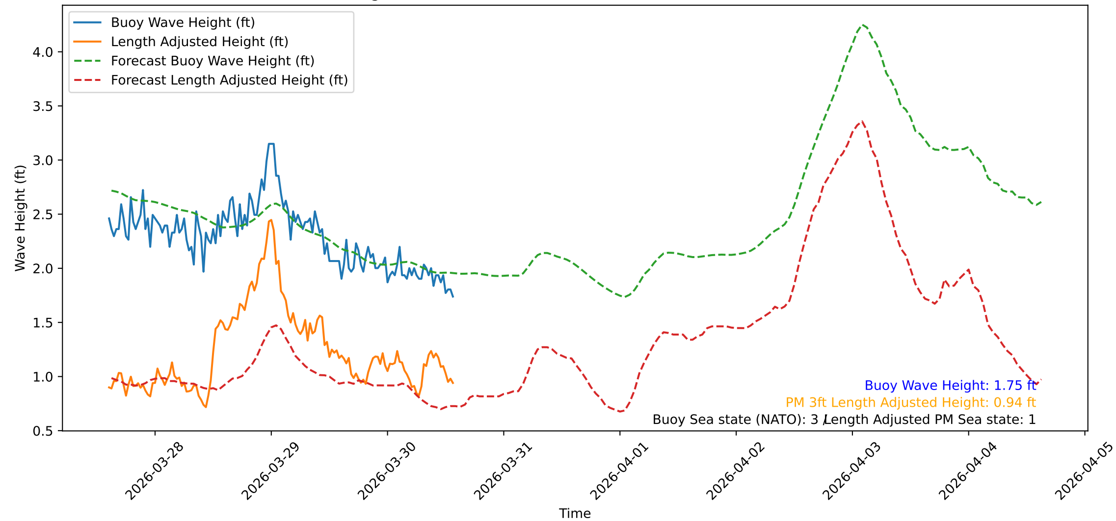
Wave Heights over Time for Oceanside Harbor at 2026-03-30 14:30:31
