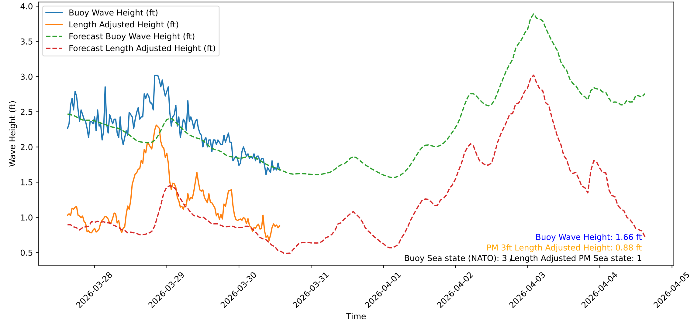
Wave Heights over Time for Red Beach at 2026-03-30 14:30:47
