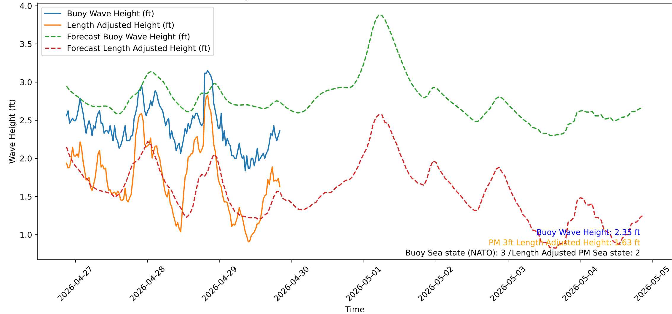
Wave Heights over Time for Green Beach at 2026-04-29 21:01:14
