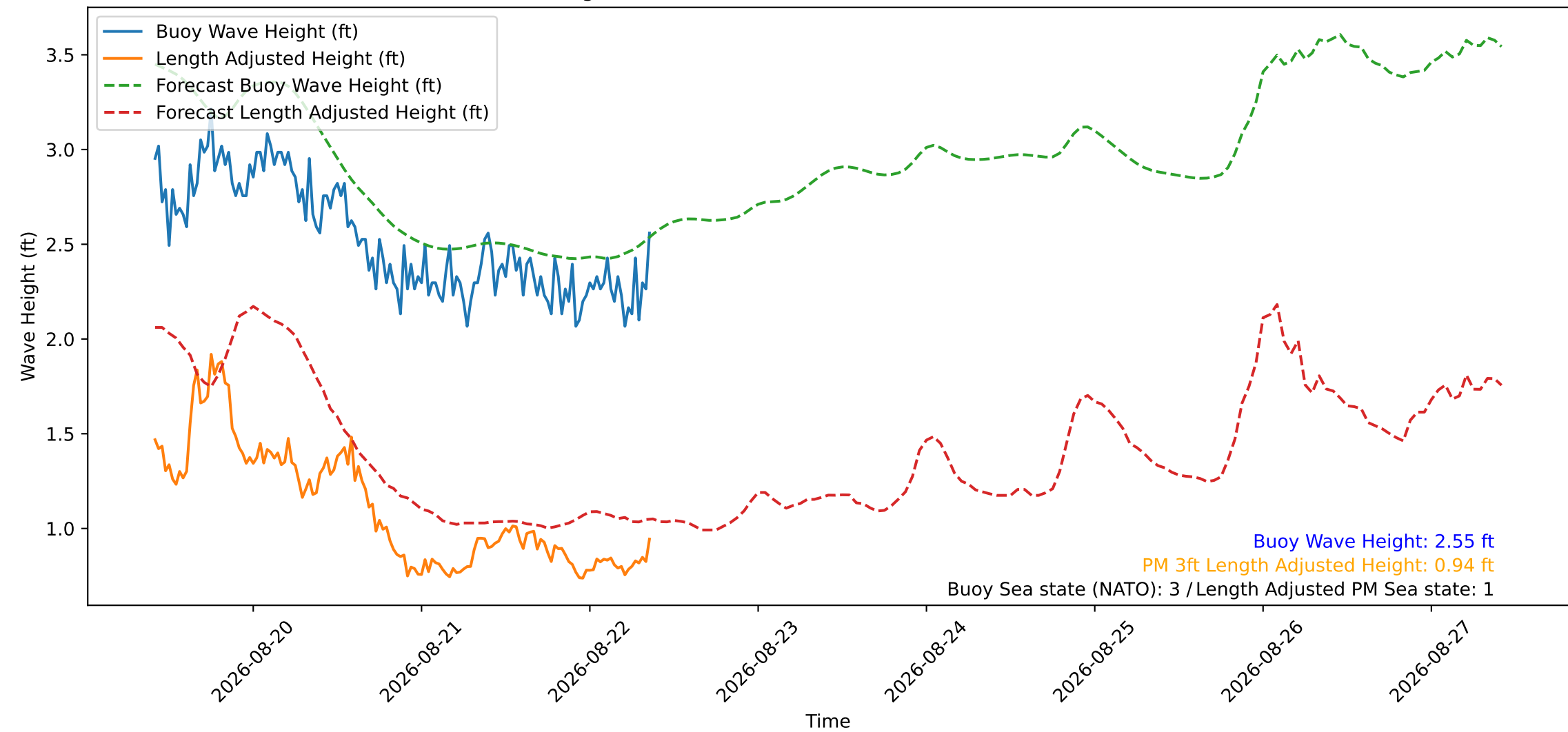
Wave Heights over Time for Red Beach at 2026-08-22 09:30:49
