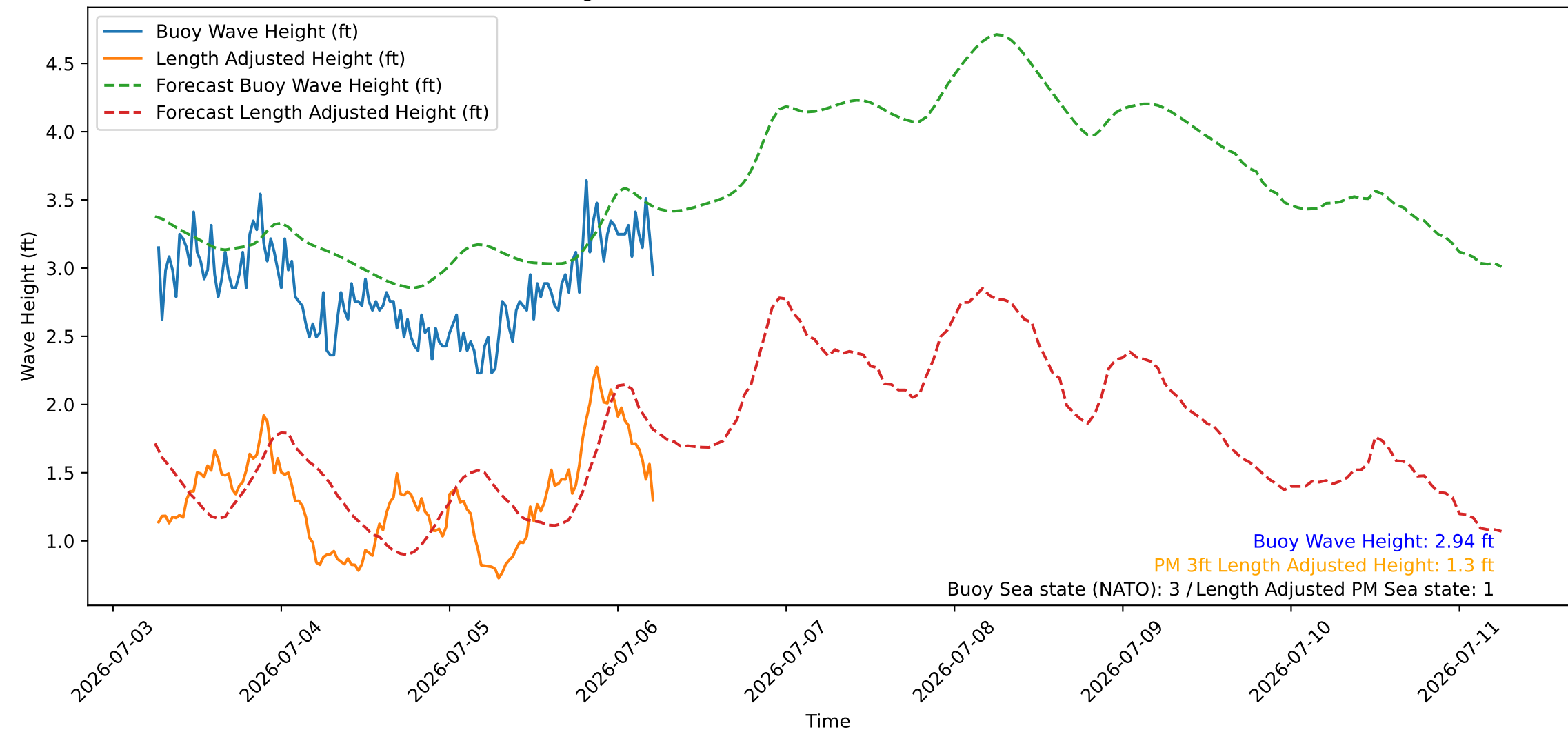
Wave Heights over Time for Red Beach at 2026-07-06 06:00:46
