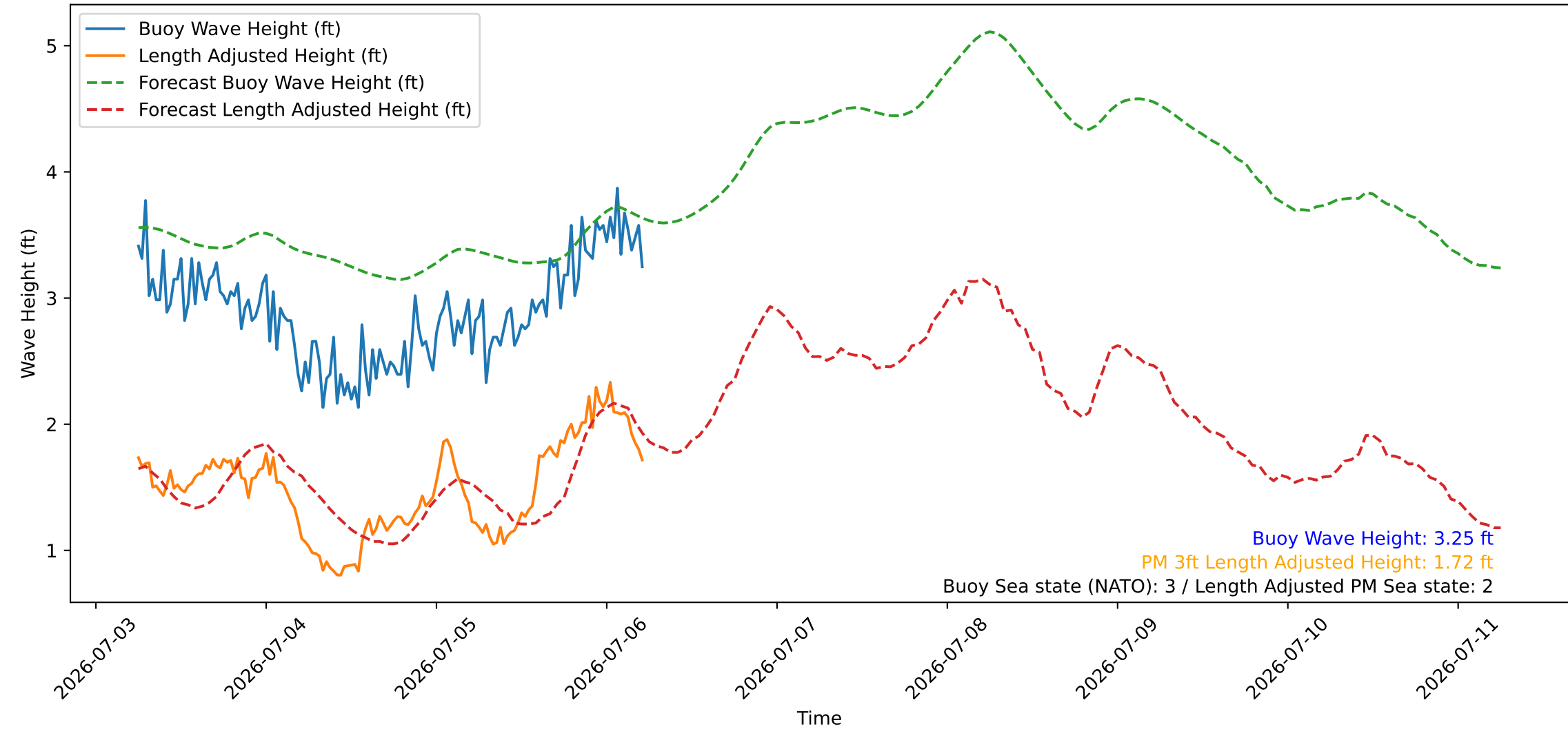
Wave Heights over Time for Oceanside Harbor at 2026-07-06 06:00:26
