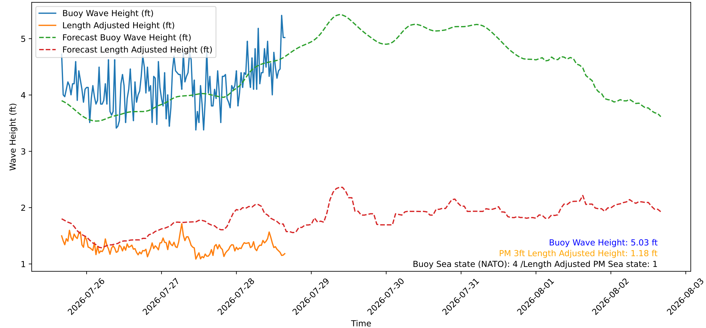
Wave Heights over Time for Green Beach at 2026-07-28 16:11:07
