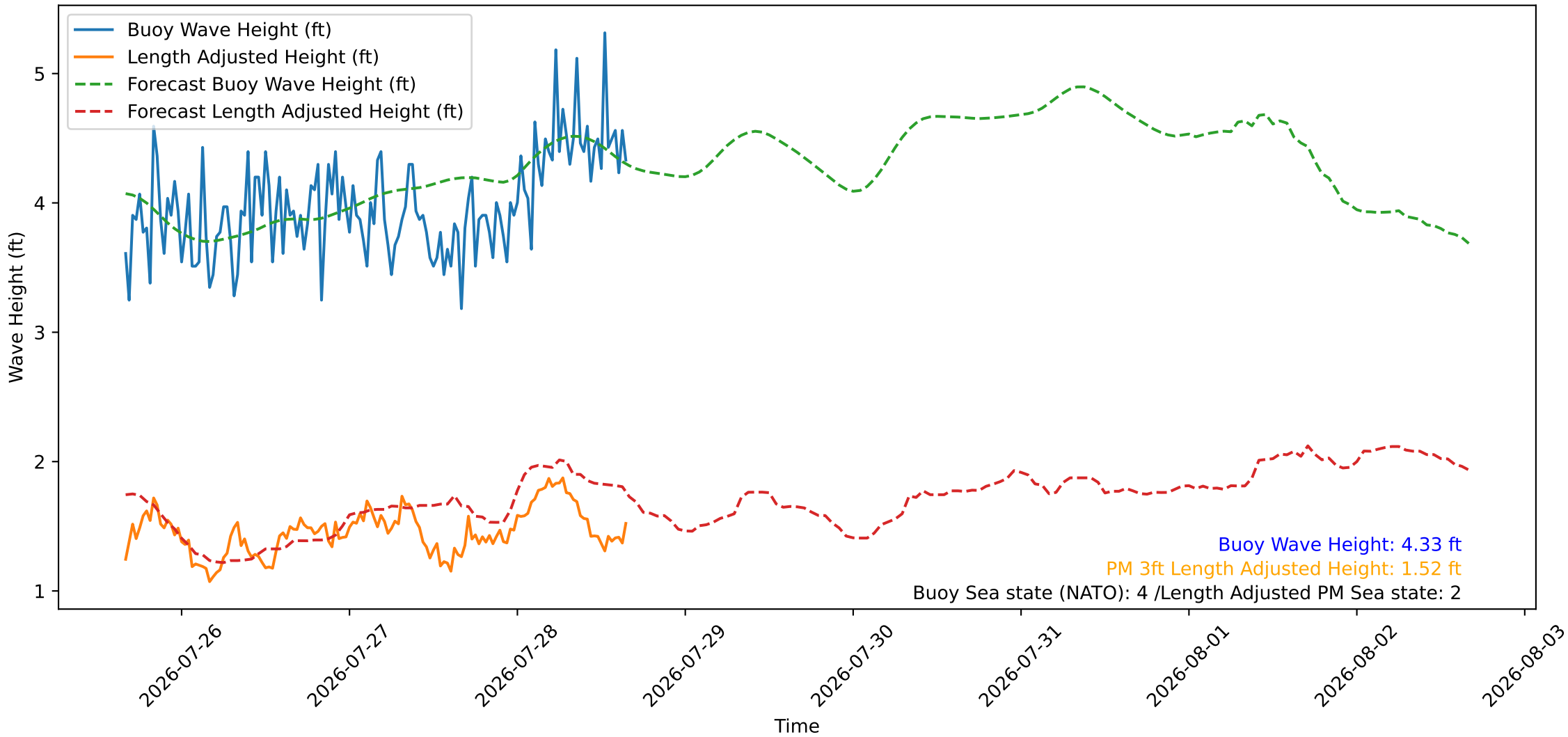
Wave Heights over Time for Oceanside Harbor at 2026-07-28 16:10:25
