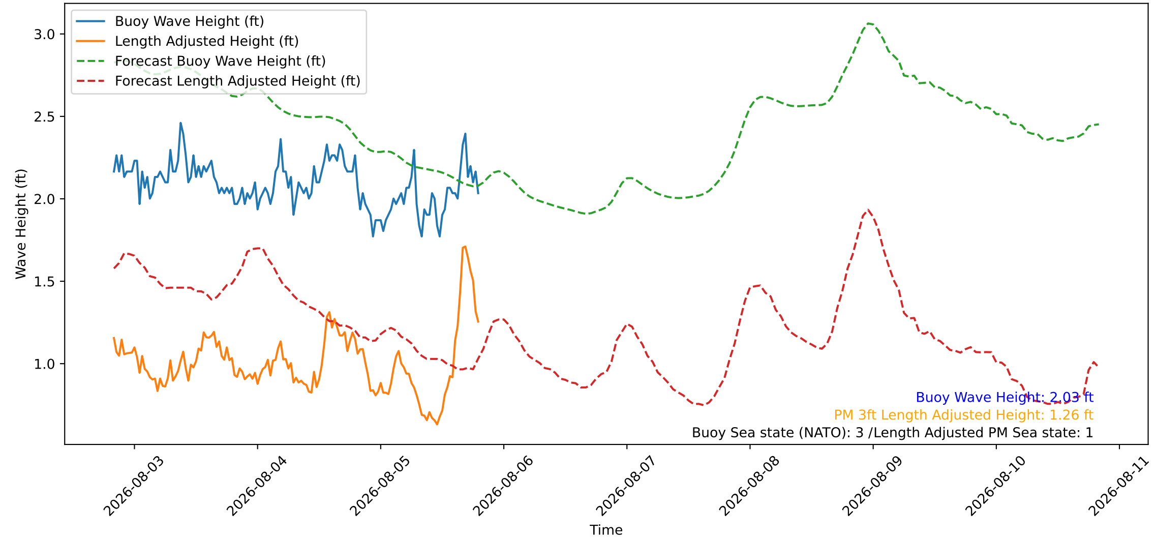
Wave Heights over Time for Red Beach at 2026-08-05 19:40:45
