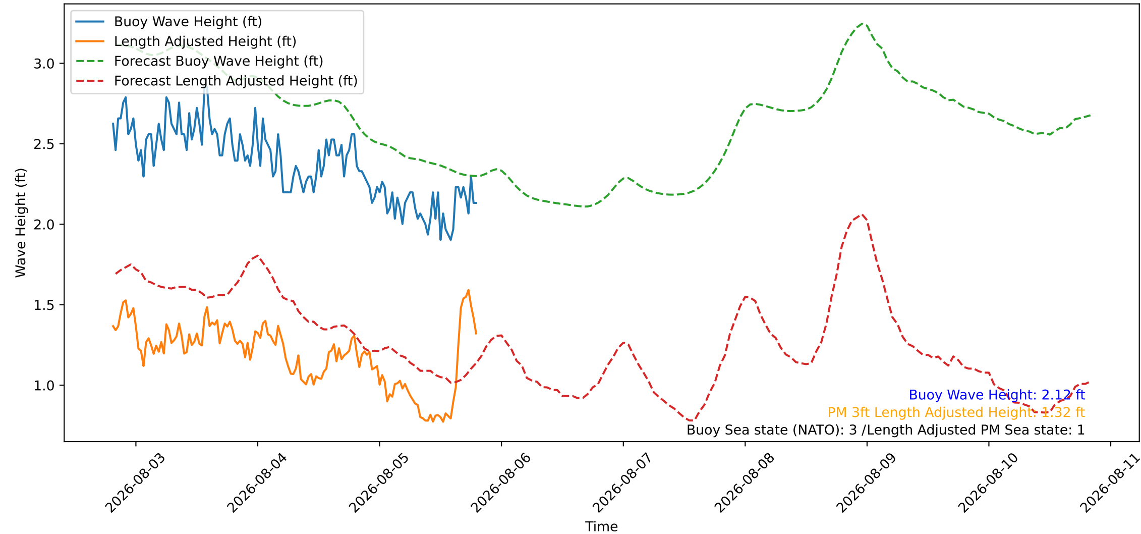
Wave Heights over Time for Oceanside Harbor at 2026-08-05 19:40:25
