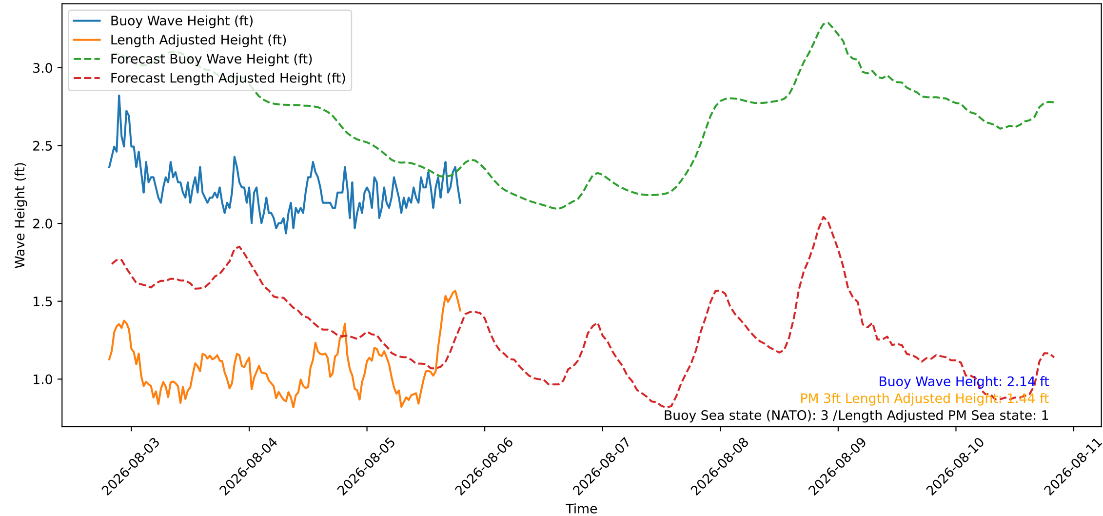
Wave Heights over Time for Green Beach at 2026-08-05 19:41:08
