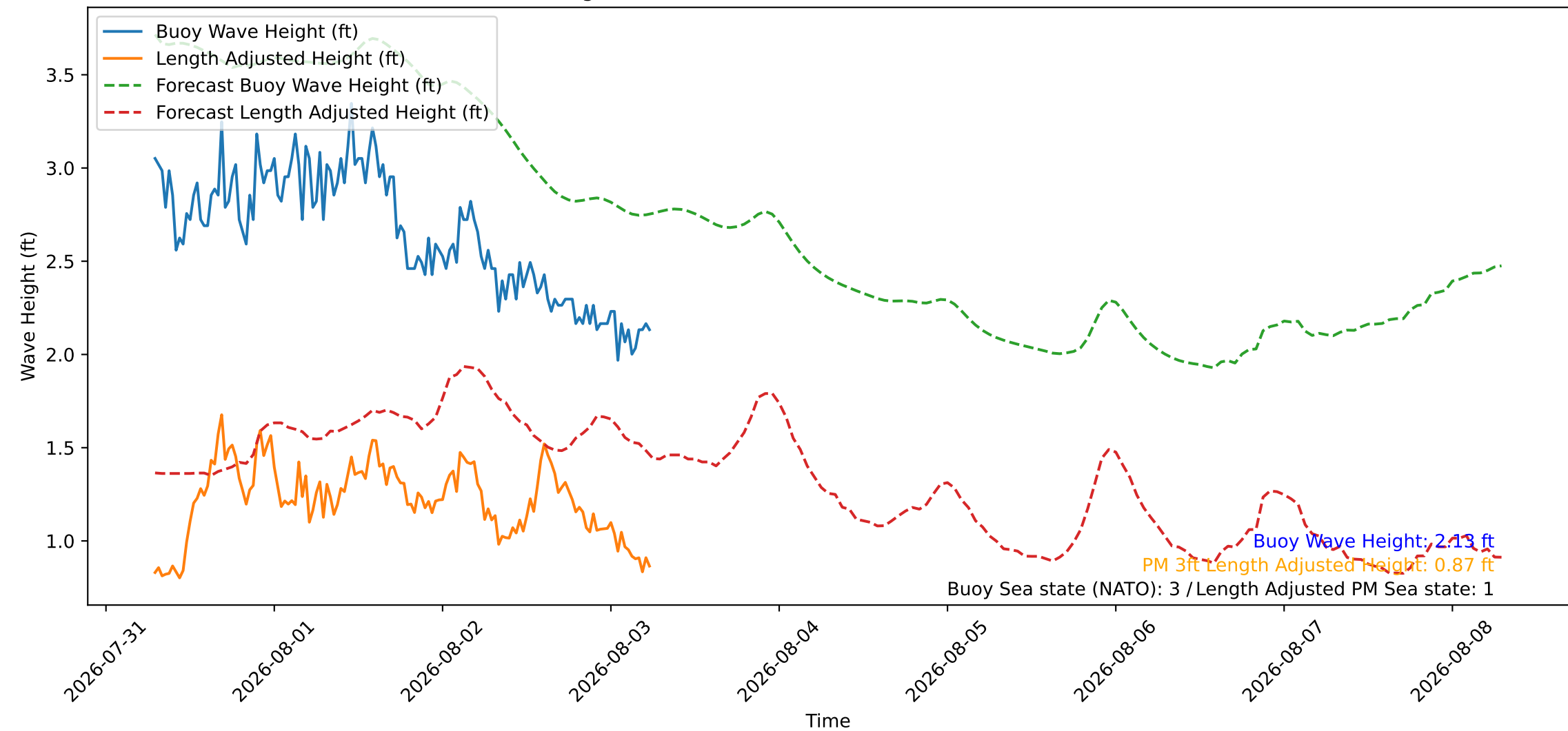
Wave Heights over Time for Red Beach at 2026-08-03 06:40:46
