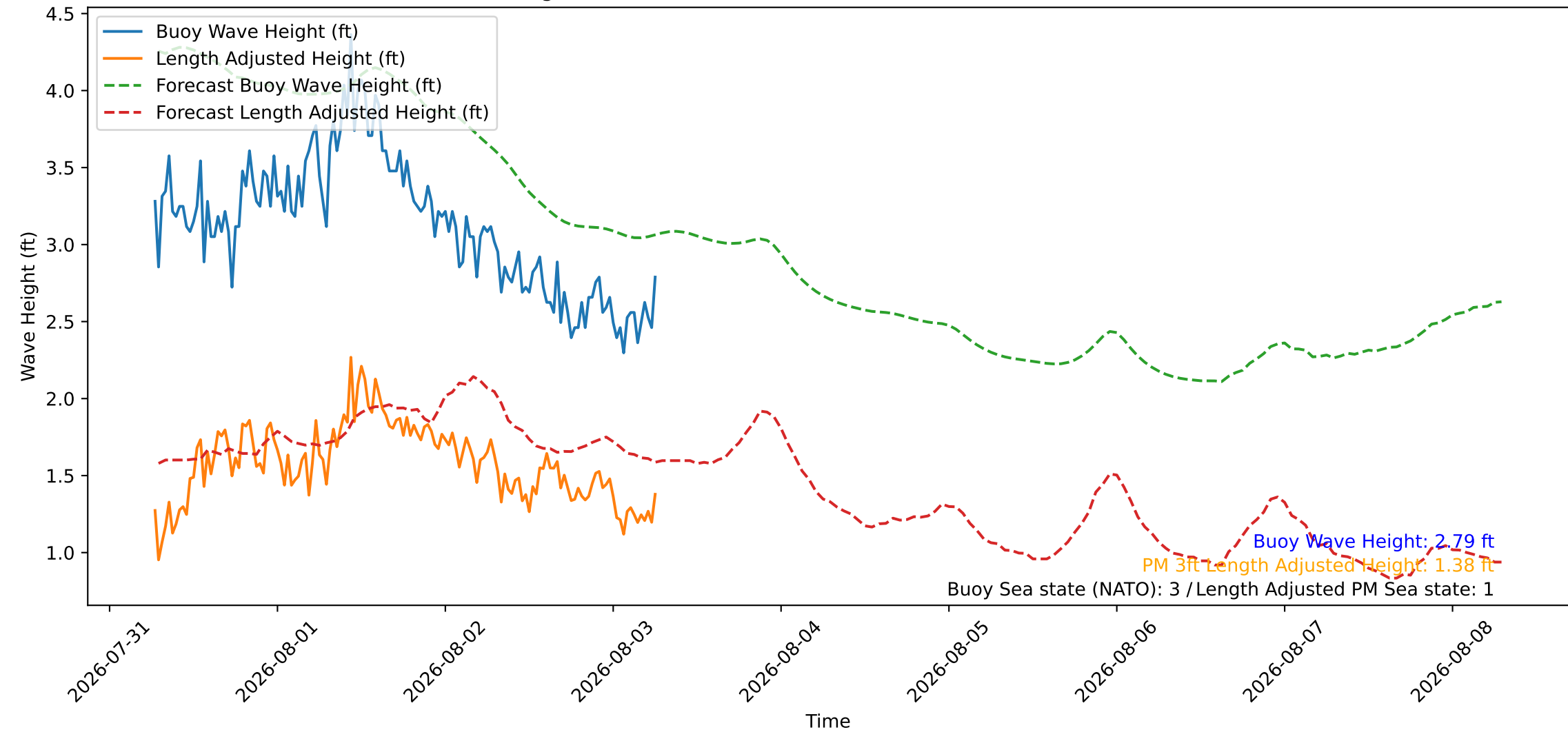
Wave Heights over Time for Oceanside Harbor at 2026-08-03 06:40:26
