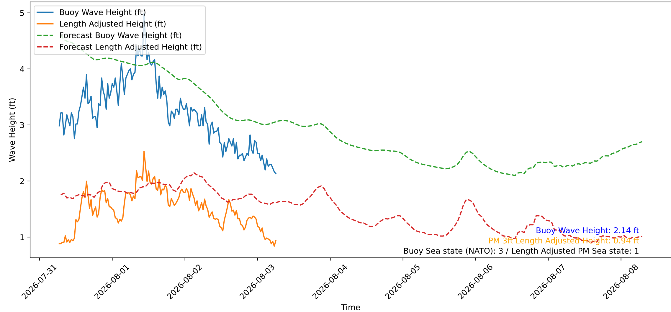
Wave Heights over Time for Green Beach at 2026-08-03 06:41:08
