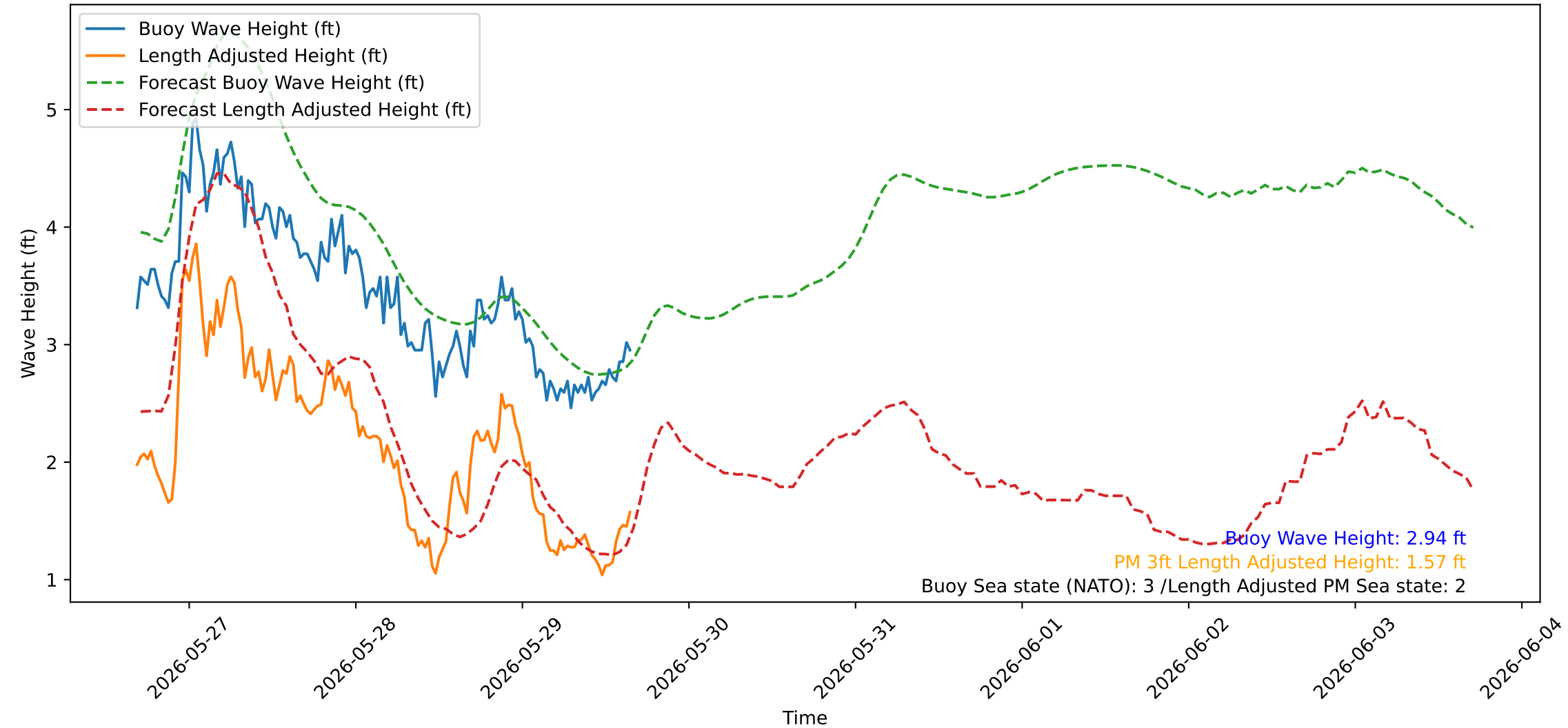
Wave Heights over Time for Green Beach at 2026-05-29 16:31:03
